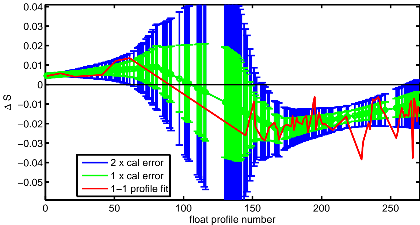
6900282 vertically-averaged salinity (PSS-78) additive correction \Delta S with errors
