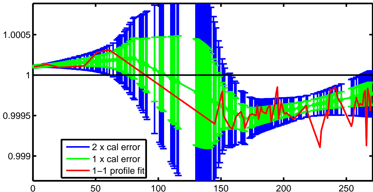
6900282 potential conductivity (mmho/cm) multiplicative correction r with errors
