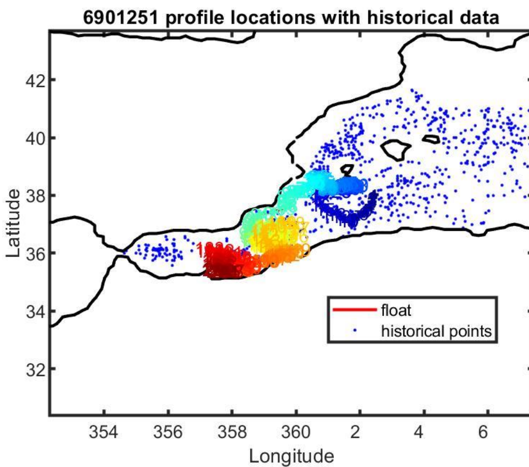
Figure 32: Float 6901251. Location of the float profiles (red line with colored numbers) and the reference data selected for mapping (blue dots).
