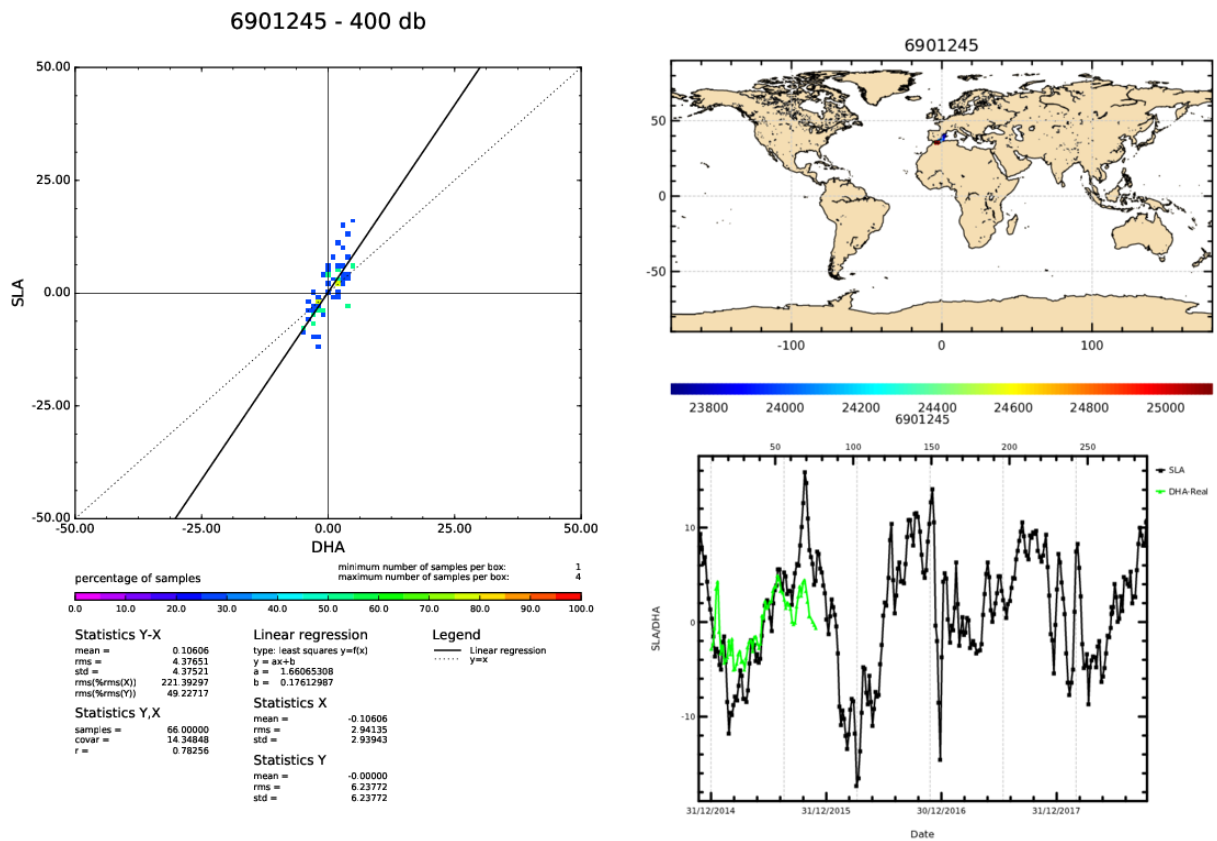
Figure 1: Float 6901245. The comparison between the sea surface height (SSH) from the satellite altimetry and dynamic height anomaly (DHA) extracted from the Argo float temperature and salinity. The figure is created by the CLS/Coriolis and distributed by Ifremer ( http://ftp.ifremer.fr/ifremer/argo/etc/argo-ast9-item13-AltimeterComparison/figures/ ).
