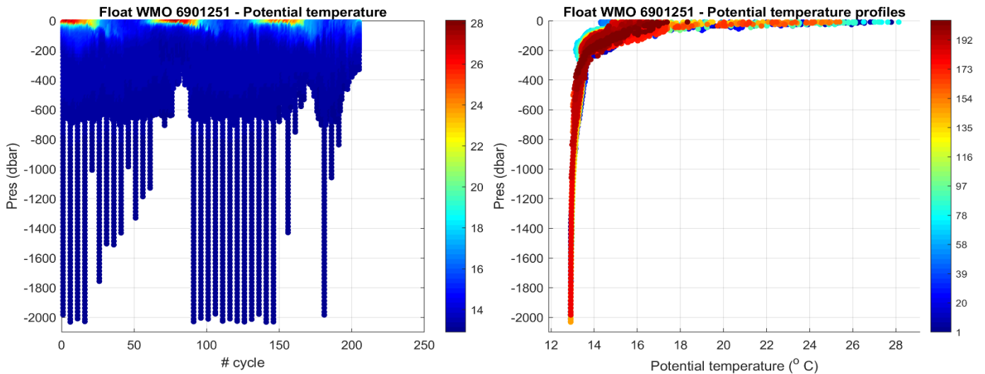
Figure 21: Float 6901251. Time series of Argo float potential temperature (°C) on the left, and potential temperature profiles color-coded per cycle number on the right.
