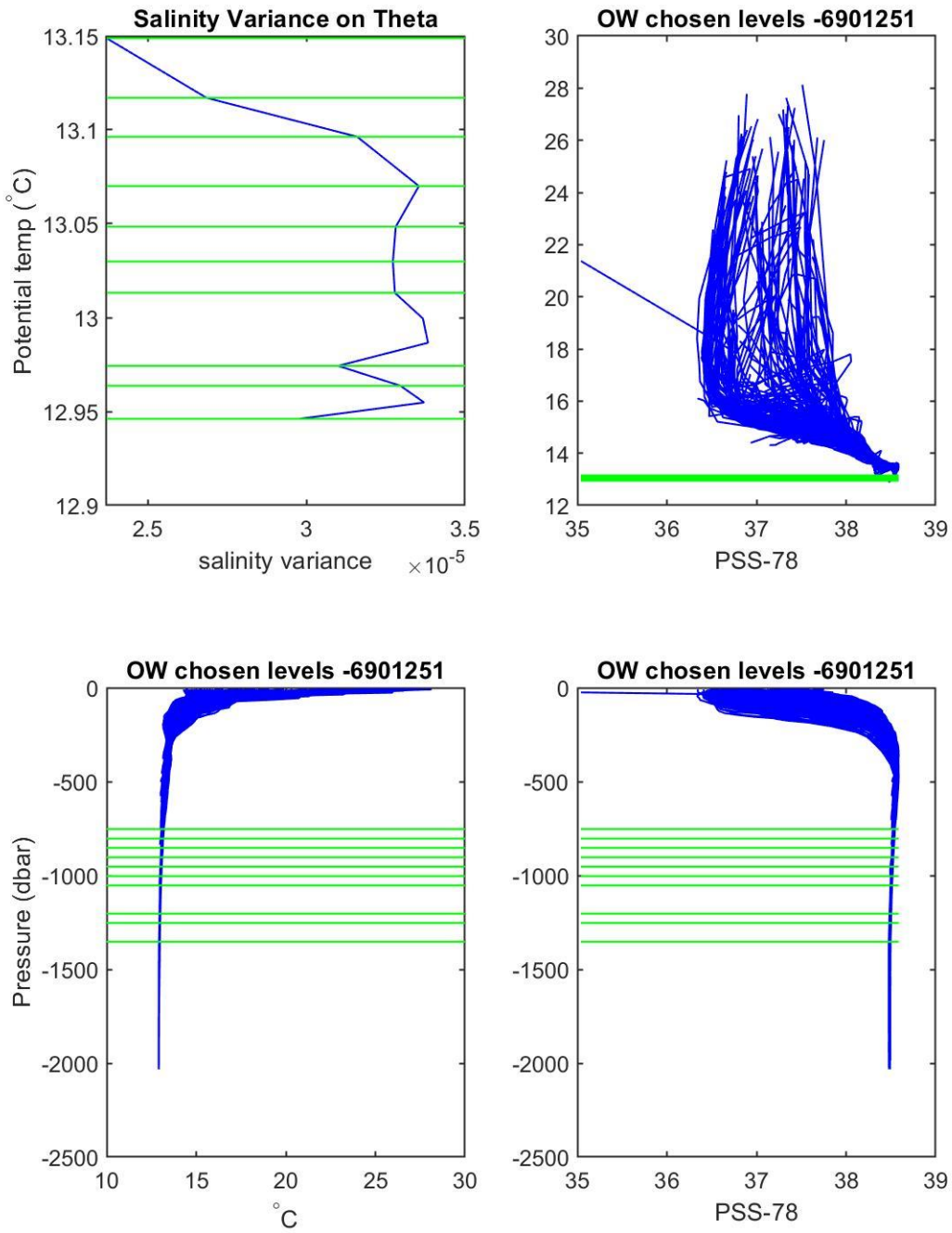
Figure 37: Float 6901251. Plots include the theta levels chosen for calibration: Top left: Salinity variance at theta levels. Top right: T/S diagram of all profiles of Argo float. Bottom left: potential temperature plotted against pressure. Bottom right: salinity plotted against pressure.
