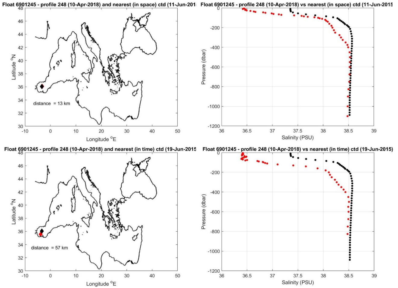
Figure 11: Float 6901245. The salinity float profile number 248 (black dots) are compared to the nearest in space (top) and in time (bottom) reference profile (red dots). The locations of the two profiles and their distance is given in the left panel.
