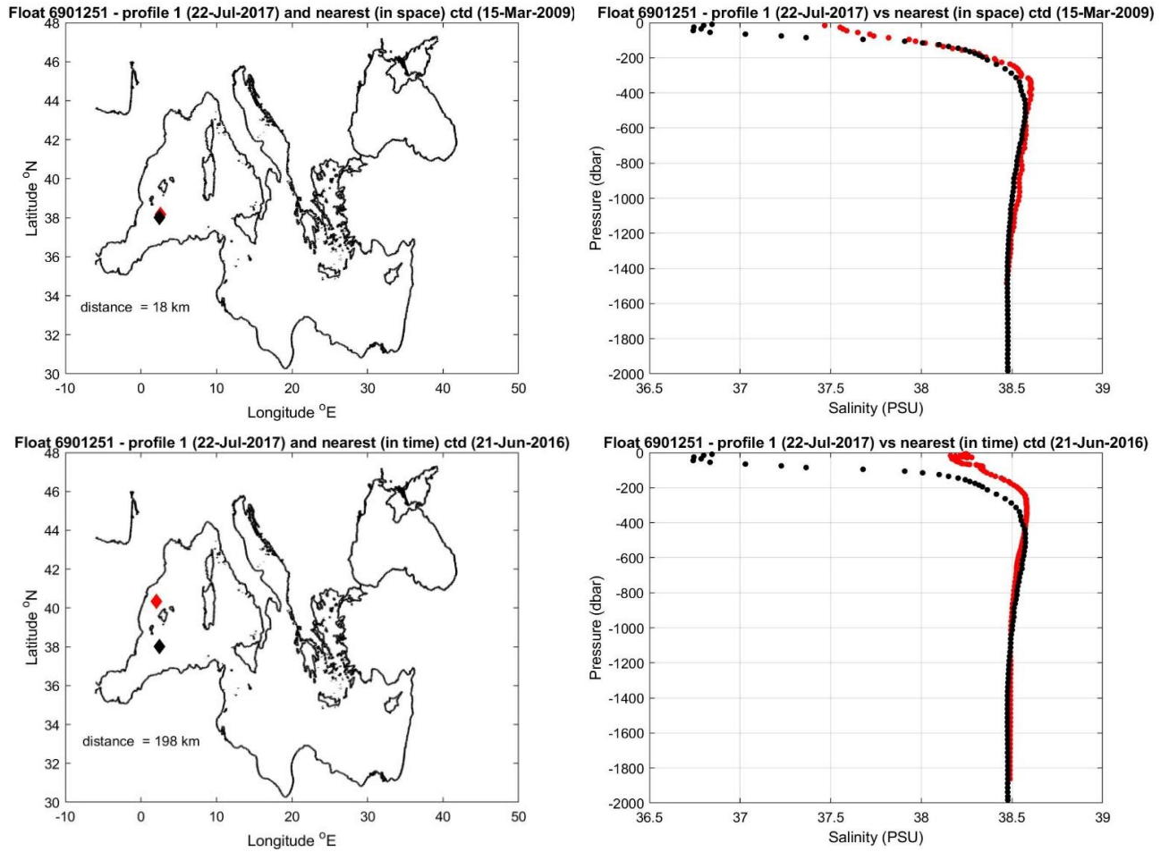
Figure 28: Float 6901251. The salinity float profile number 1 (black dots) are compared to the nearest in space (top) and in time (bottom) reference profile (red dots). The locations of the two profiles and their distance is given in the left panel.
