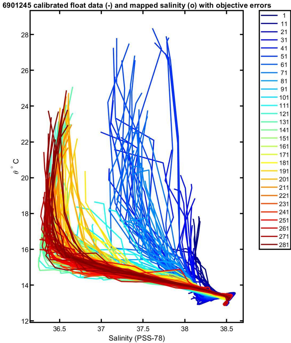
Figure 16: Float 6901245. The plot of calibrated float salinity and the objectively estimated reference salinity at the 10 float theta levels that are used in calibration.
