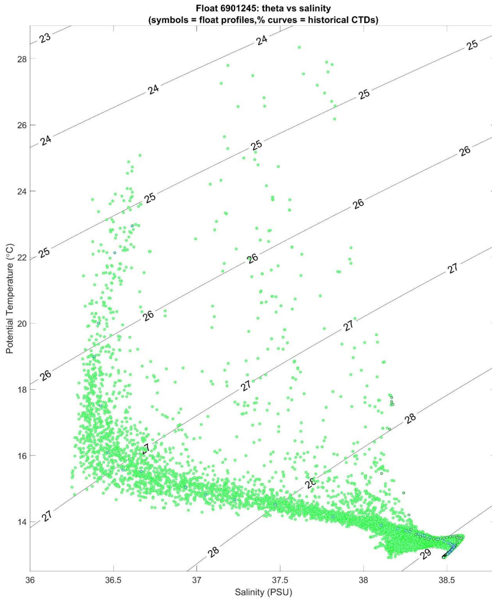
Figure 12: Float 6901245. T/S diagram plotted with and data from WMO boxes of CTD reference data +/- 10° of latitude and longitude. The black and blue cycles indicate the first and the last Argo profile, respectively. Green symbols represent other Argo profiles from this float. The thin colours lines indicate the reference data.
