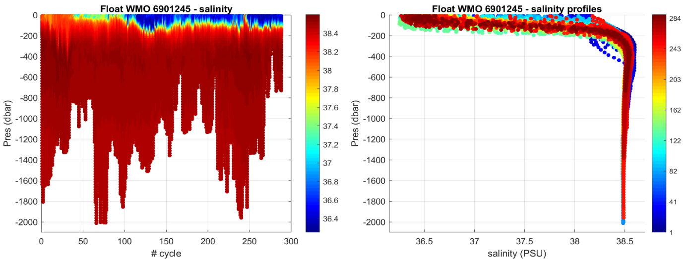
Figure 3: Float 6901245. Time series of Argo float potential salinity (PSS-78) on the left, and salinity profiles color-coded per cycle number on the right.
