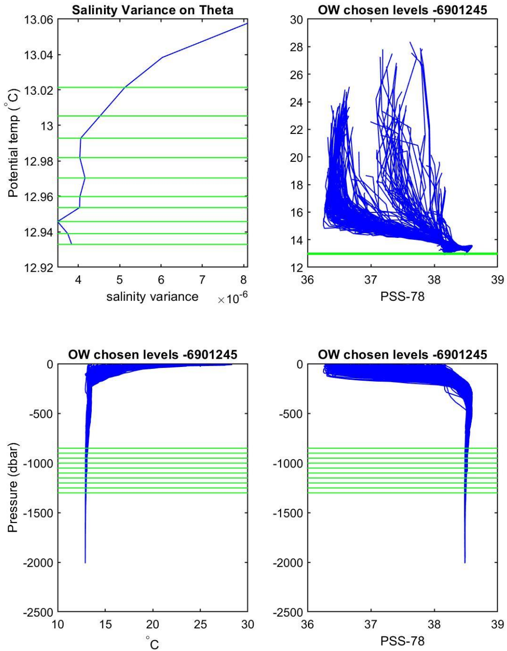
Figure 18: Float 6901245. Plots include the theta levels chosen for calibration: Top left: Salinity variance at theta levels. Top right: T/S diagram of all profiles of Argo float. Bottom left: potential temperature plotted against pressure. Bottom right: salinity plotted against pressure.
