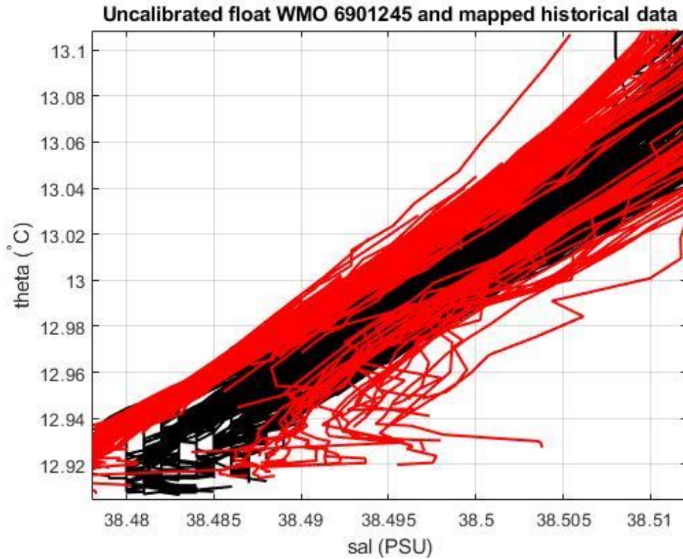
Figure 19: Float 6901245. Uncalibrated float salinity profile (black lines) and mapped historical data (red lines) in the most uniform part of the \theta -S curve.
