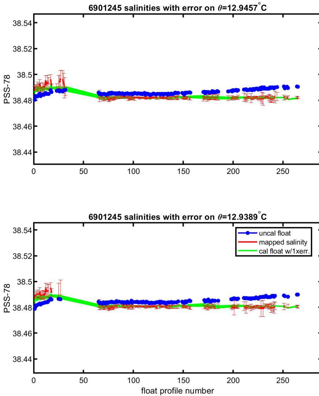
Figure 17: Float 6901245. Plots of the evolution of salinity with time along with selected theta levels with minimum salinity variance.
