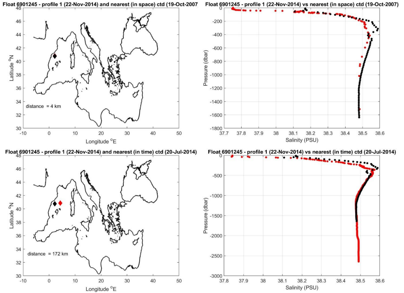
Figure 9: Float 6901245. The salinity float profile number 1 (black dots) are compared to the nearest in space (top) and in time (bottom) reference profile (red dots). The locations of the two profiles and their distance is given in the left panel.
