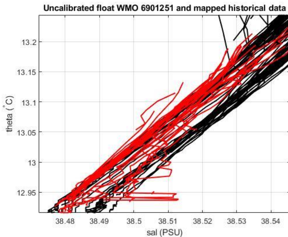
Figure 38: Float 6901251. Uncalibrated float salinity profile (black lines) and mapped historical data (red lines) in the most uniform part of the \theta -S curve.
