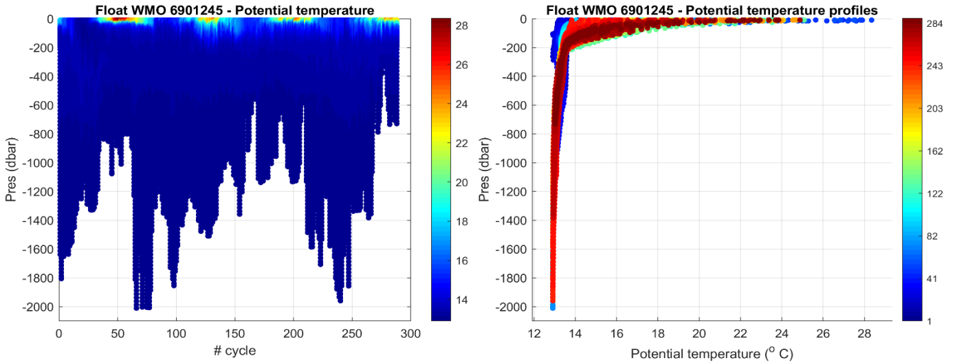
Figure 2: Float 6901245. Time series of Argo float potential temperature (°C) on the left, and potential temperature profiles color-coded per cycle number on the right.
