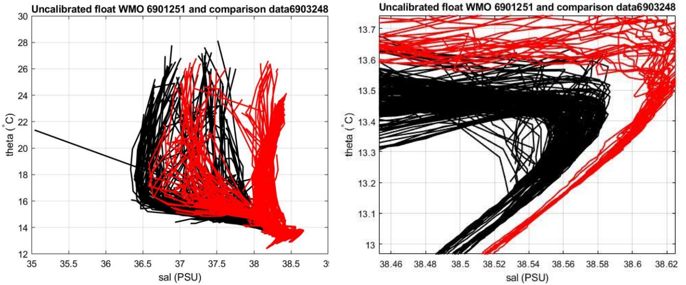
Figure 40: Float 6901251. Comparison between float 6901251 (black line) and float 6903248 (red line), on the left. On the right zoom in the most uniform part of the \theta -S curve and only for cycles from 269 to 300 (Catalan and Algerian sub basins).
