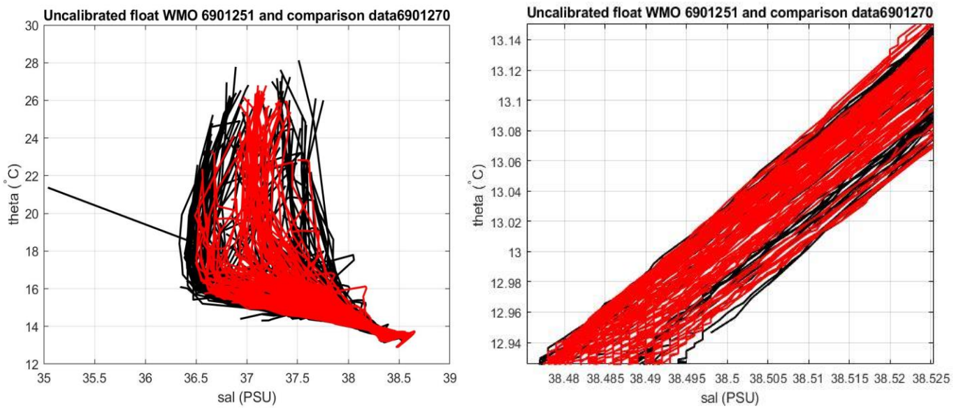
Figure 41: Float 6901251. Comparison between float 6901251 (black line) and float 6901270 (red line), on the left. On the right zoom in the most uniform part of the \theta -S curve.
