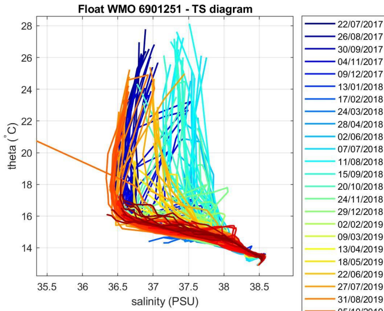
Figure 23: Float 6901251. \theta -S diagram color-coded per cycle number.
