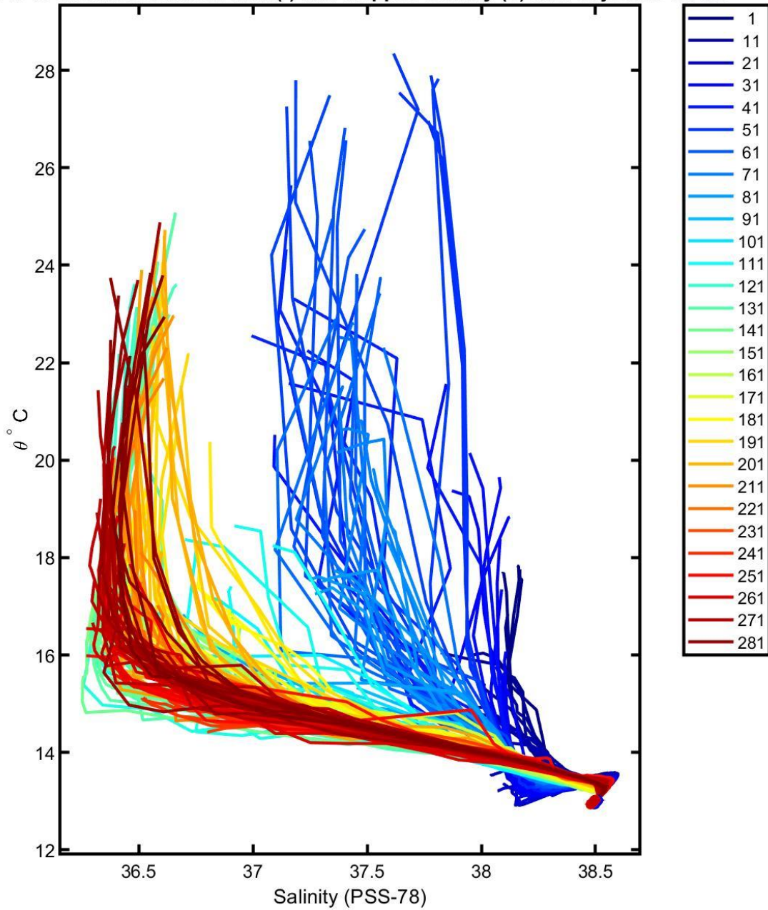
6901245 uncalibrated float data (-) and mapped salinity (o) with objective errors
