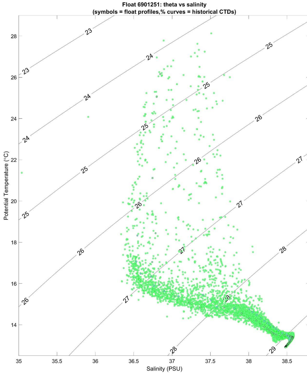
Figure 31: Float 6901251. T/S diagram plotted with and data from WMO boxes of CTD reference data +/- 10° of latitude and longitude. The black and blue circles indicate the first and the last Argo profile, respectively. Green symbols represent other Argo profiles from this float. The thin colours lines indicate the reference data.
