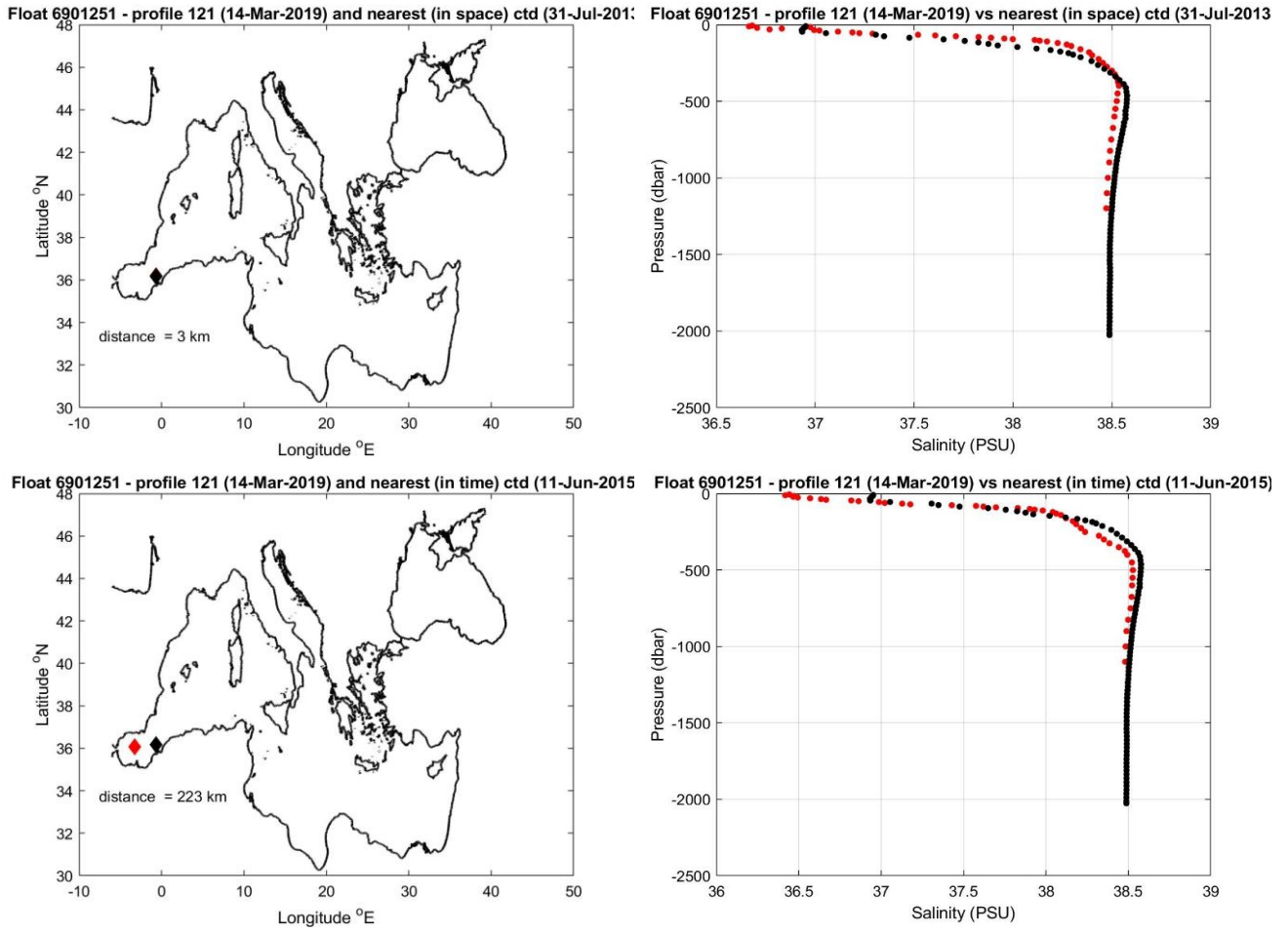
Figure 29: Float 6901251. The salinity float profile number 121 (black dots) are compared to the nearest in space (top) and in time (bottom) reference profile (red dots). The locations of the two profiles and their distance is given in the left panel.
