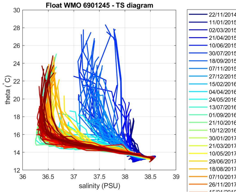
Figure 4: Float 6901245. \theta -S diagram color-coded per cycle number.
