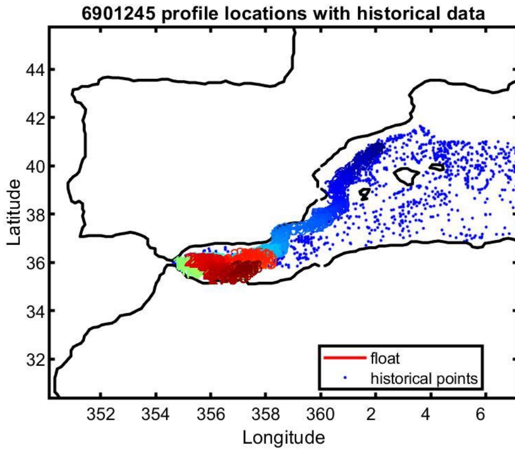
Figure 13: Float 6901245. Location of the float profiles (red line with colored numbers) and the reference data selected for mapping (blue dots).
