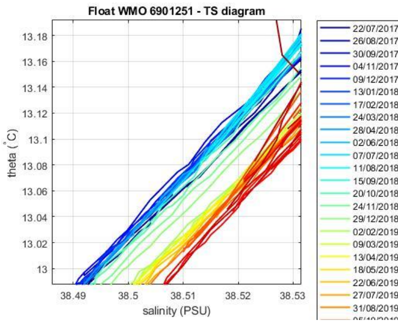
Figure 24: Float 6901251. Area of the \theta -S diagram (color-coded per cycle number) where the \theta -S relationship is more uniform.
