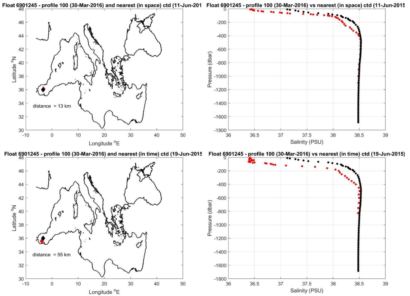
Figure 10: Float 6901245. The salinity float profile number 100 (black dots) are compared to the nearest in space (top) and in time (bottom) reference profile (red dots). The locations of the two profiles and their distance is given in the left panel.
