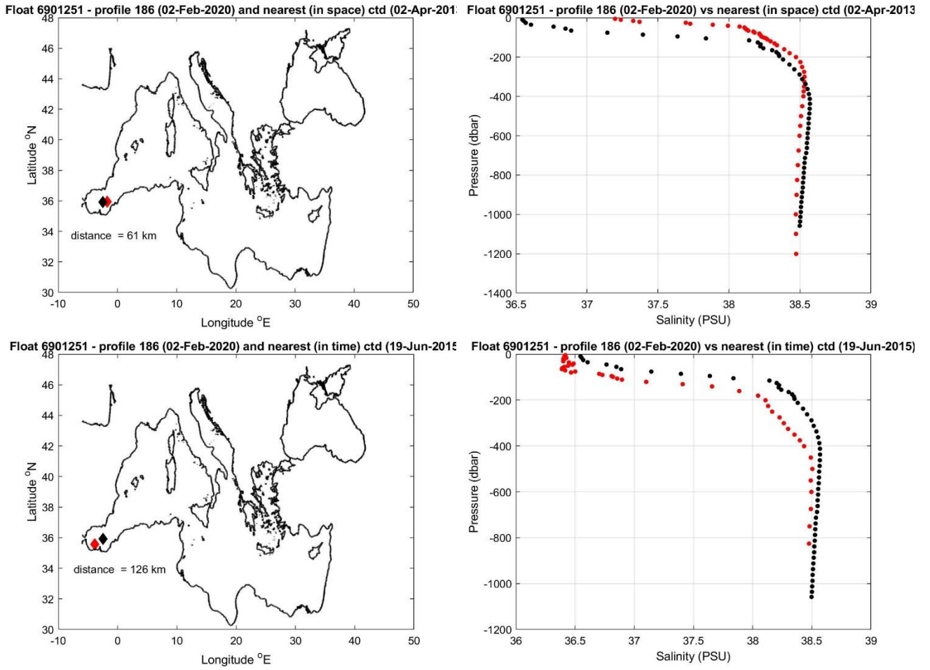
Figure 30: Float 6901251. The salinity float profile number 186 (black dots) are compared to the nearest in space (top) and in time (bottom) reference profile (red dots). The locations of the two profiles and their distance is given in the left panel.
