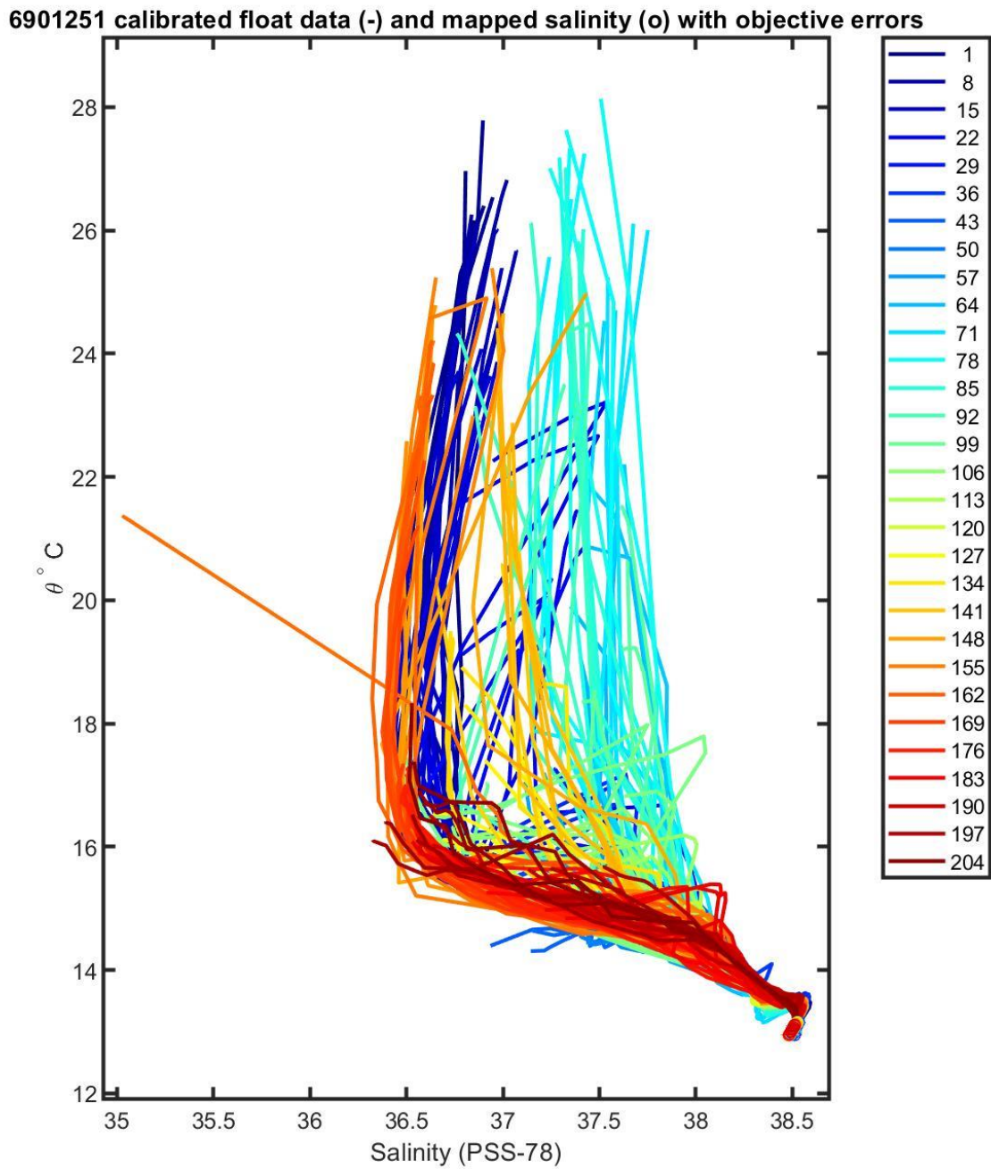
Figure 35: Float 6901251. The plot of calibrated float salinity and the objectively estimated reference salinity at the 10 float theta levels that are used in calibration.
