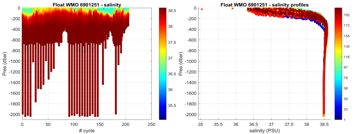
Figure 22: Float 6901251. Time series of Argo float potential salinity (PSS-78) on the left, and salinity profiles color-coded per cycle number on the right.
