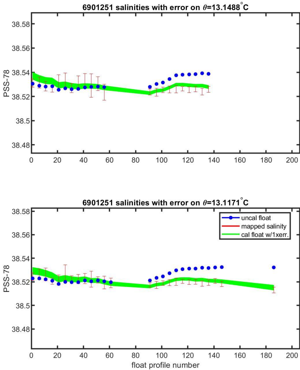
Figure 36: Float 6901251. Plots of the evolution of salinity with time along with selected theta levels with minimum salinity variance.
