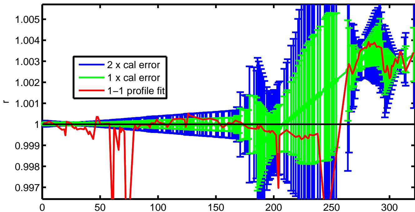
6900281 potential conductivity (mmho/cm) multiplicative correction r with errors
