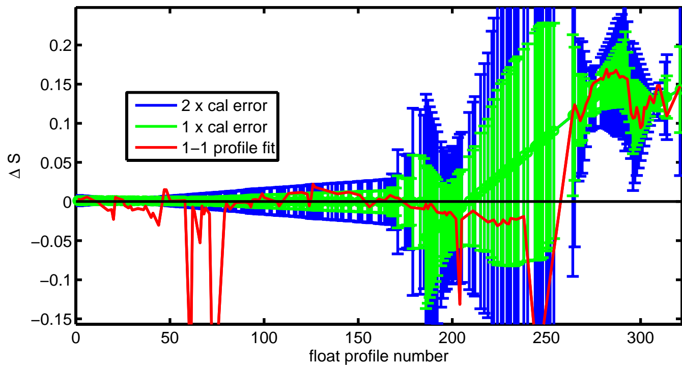
6900281 vertically-averaged salinity (PSS-78) additive correction \Delta S with errors
