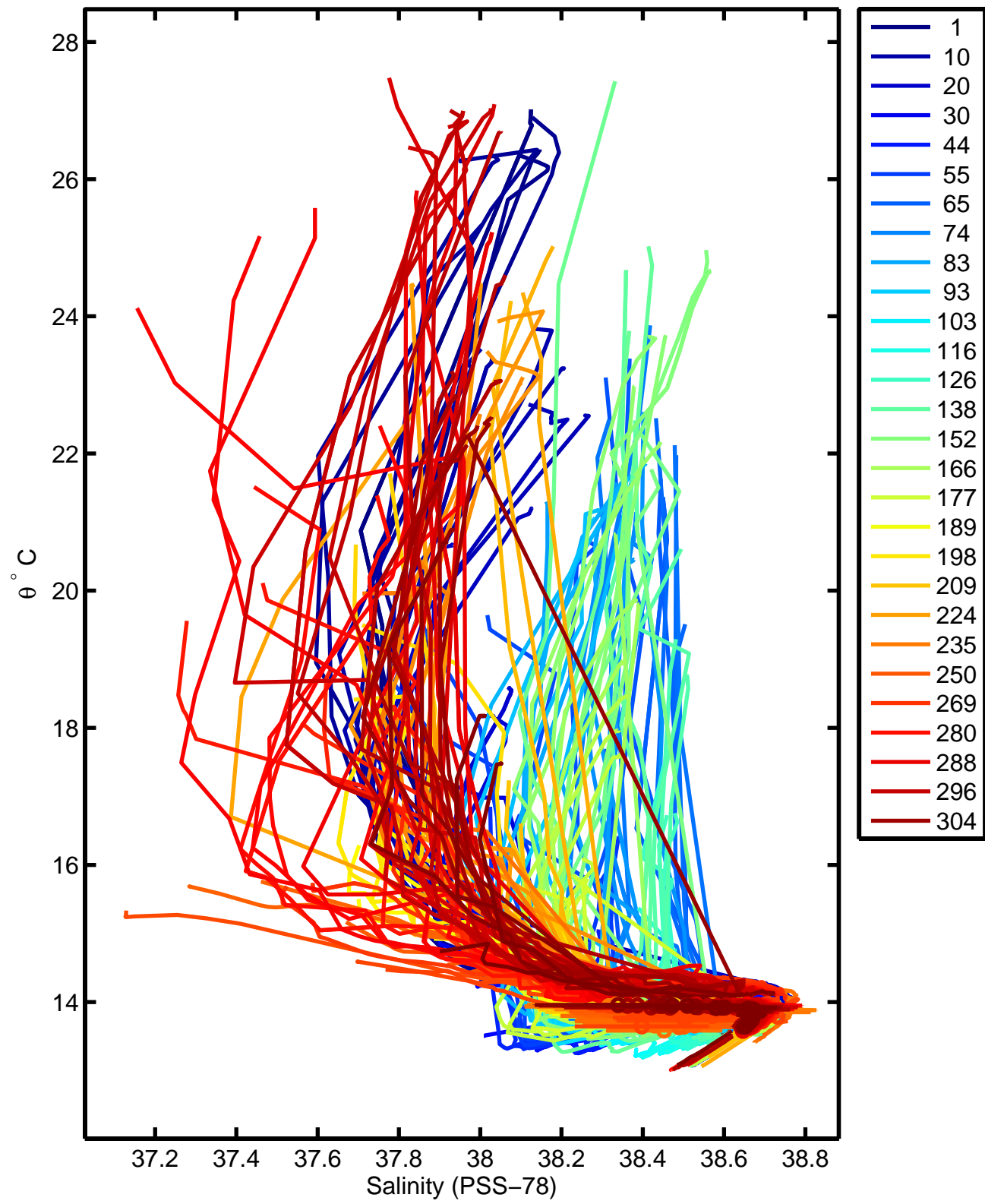
6900281 calibrated float data (-) and mapped salinity (o) with objective errors
