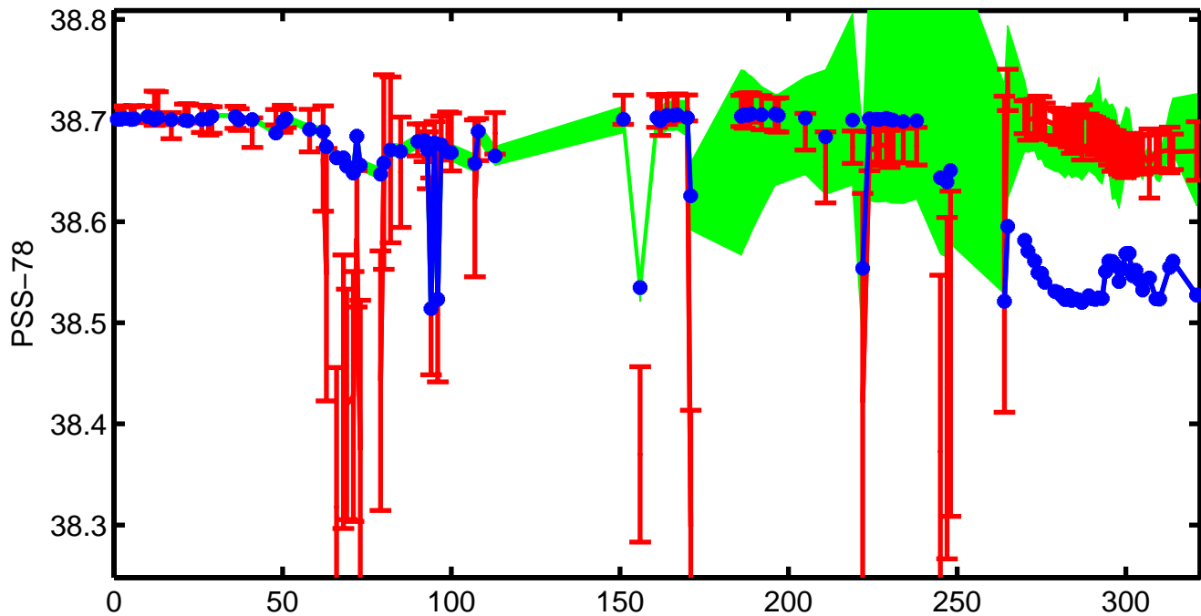
6900281 salinities with error on \theta=13.7943^\circ\text{C}
