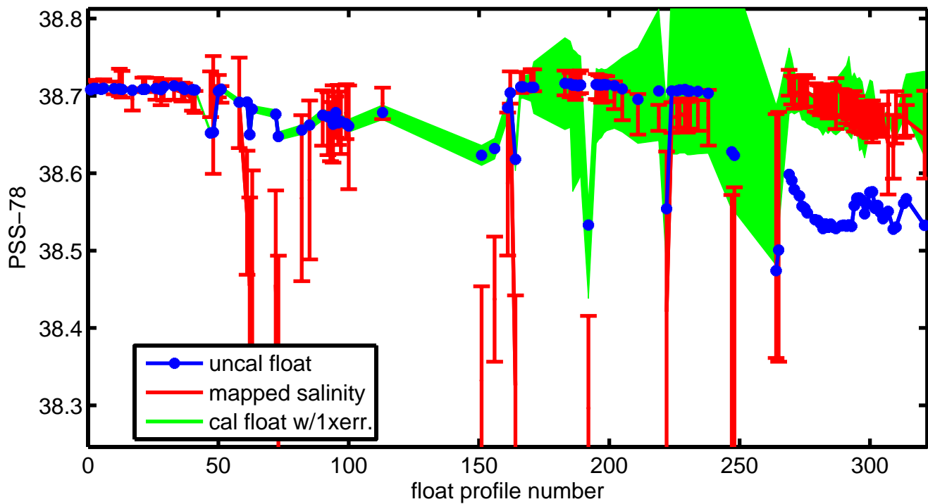
6900281 salinities with error on \theta=13.8315^\circ\text{C}
