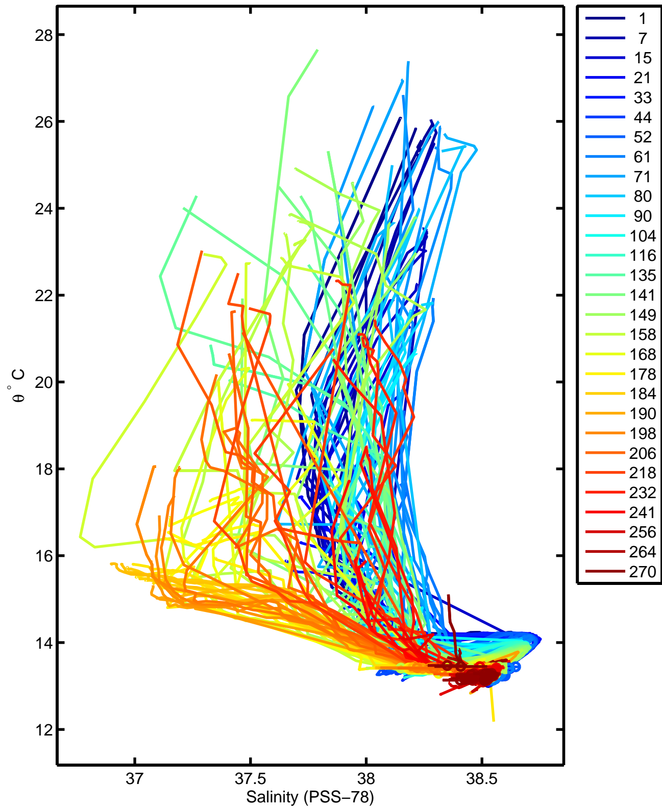
6900282 uncalibrated float data (-) and mapped salinity (o) with objective errors
