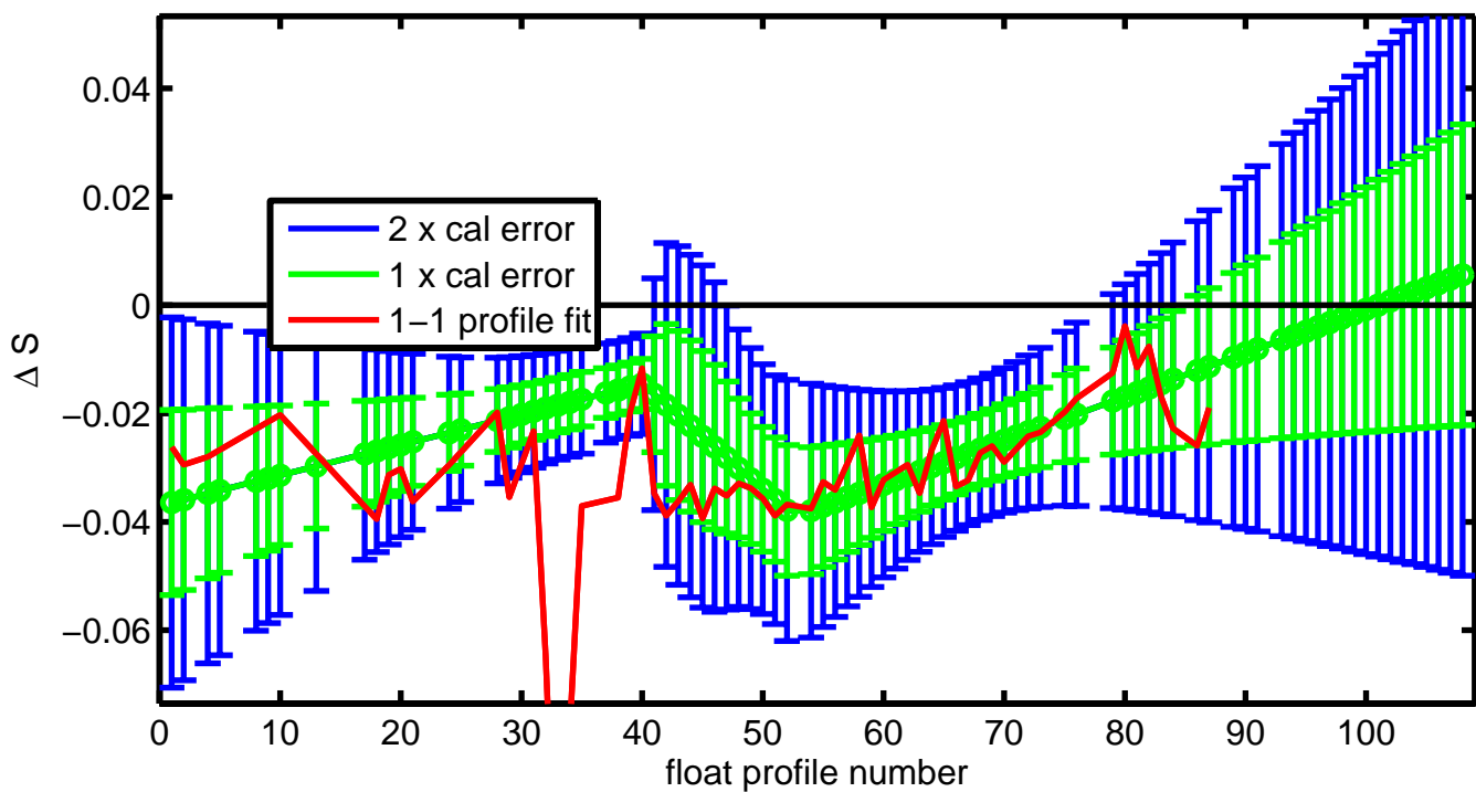
6900285 vertically-averaged salinity (PSS-78) additive correction \Delta S with errors
