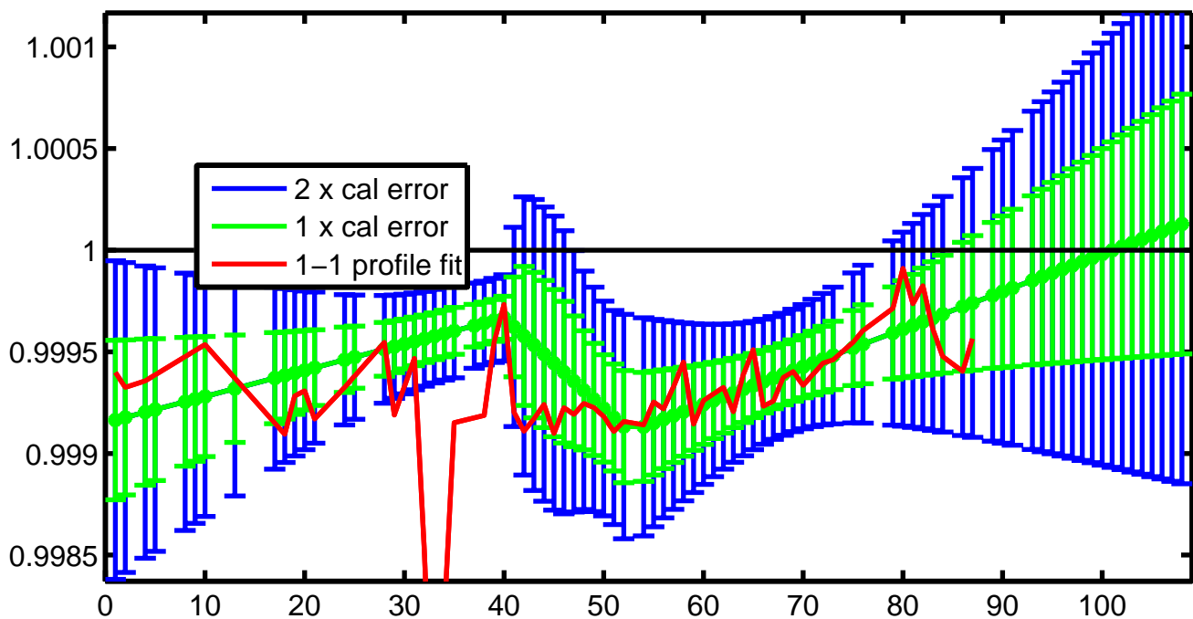
6900285 potential conductivity (mmho/cm) multiplicative correction r with errors
