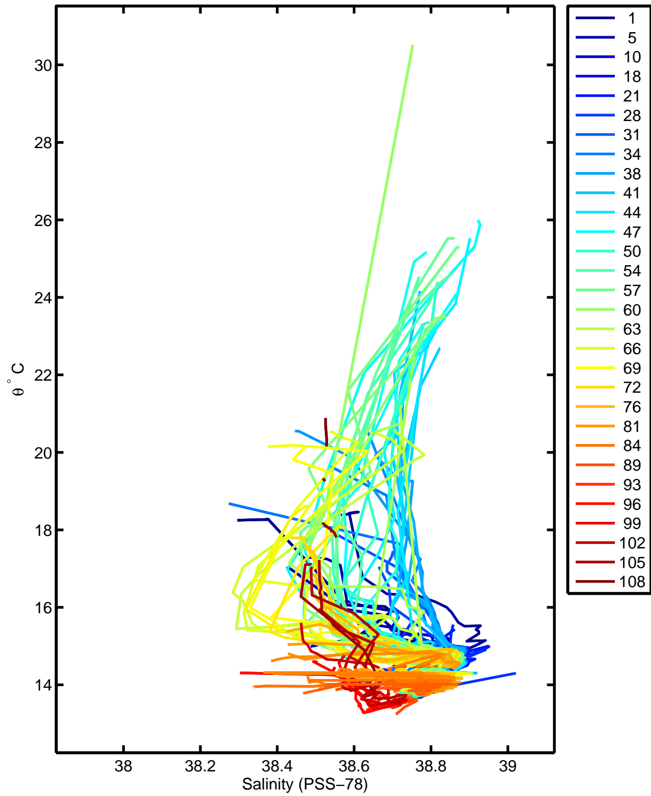
6900285 calibrated float data (-) and mapped salinity (o) with objective errors
