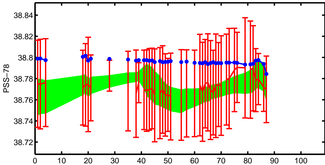
6900285 salinities with error on \theta=13.8512^{\circ}\text{C}
