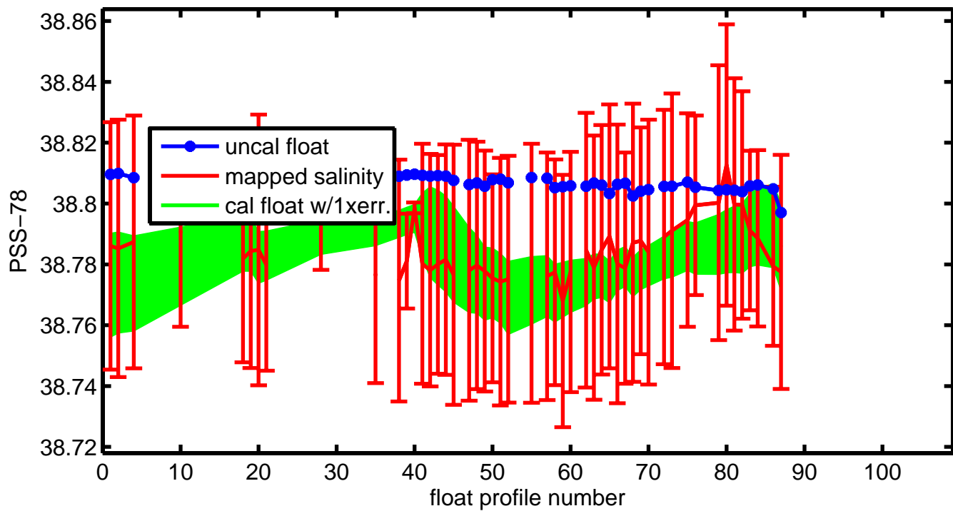
6900285 salinities with error on \theta=13.9107^{\circ}\text{C}
