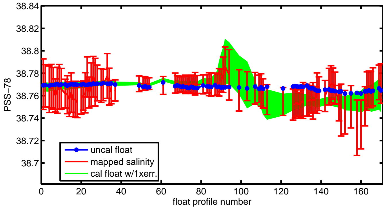
6900302 salinities with error on \theta=13.7003^\circ\text{C}
