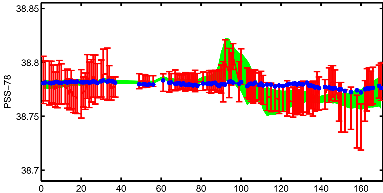
6900302 salinities with error on \theta=13.7528^\circ\text{C}
