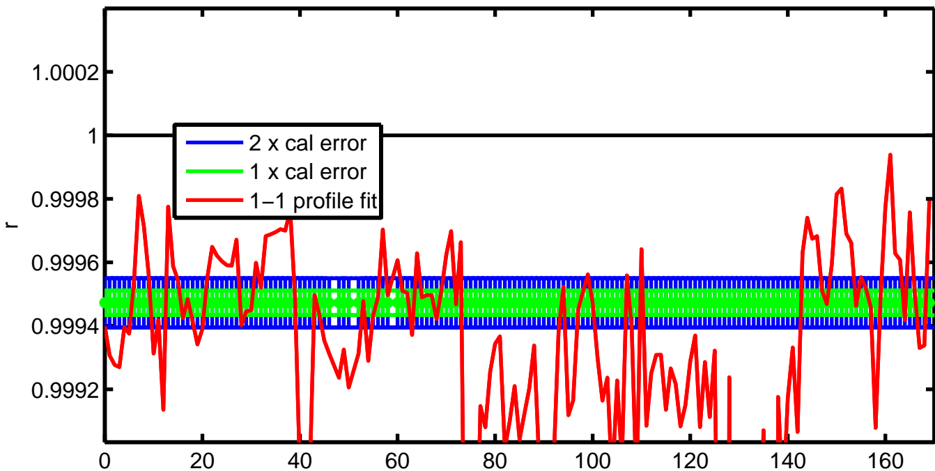
6900457 potential conductivity (mmho/cm) multiplicative correction r with errors
