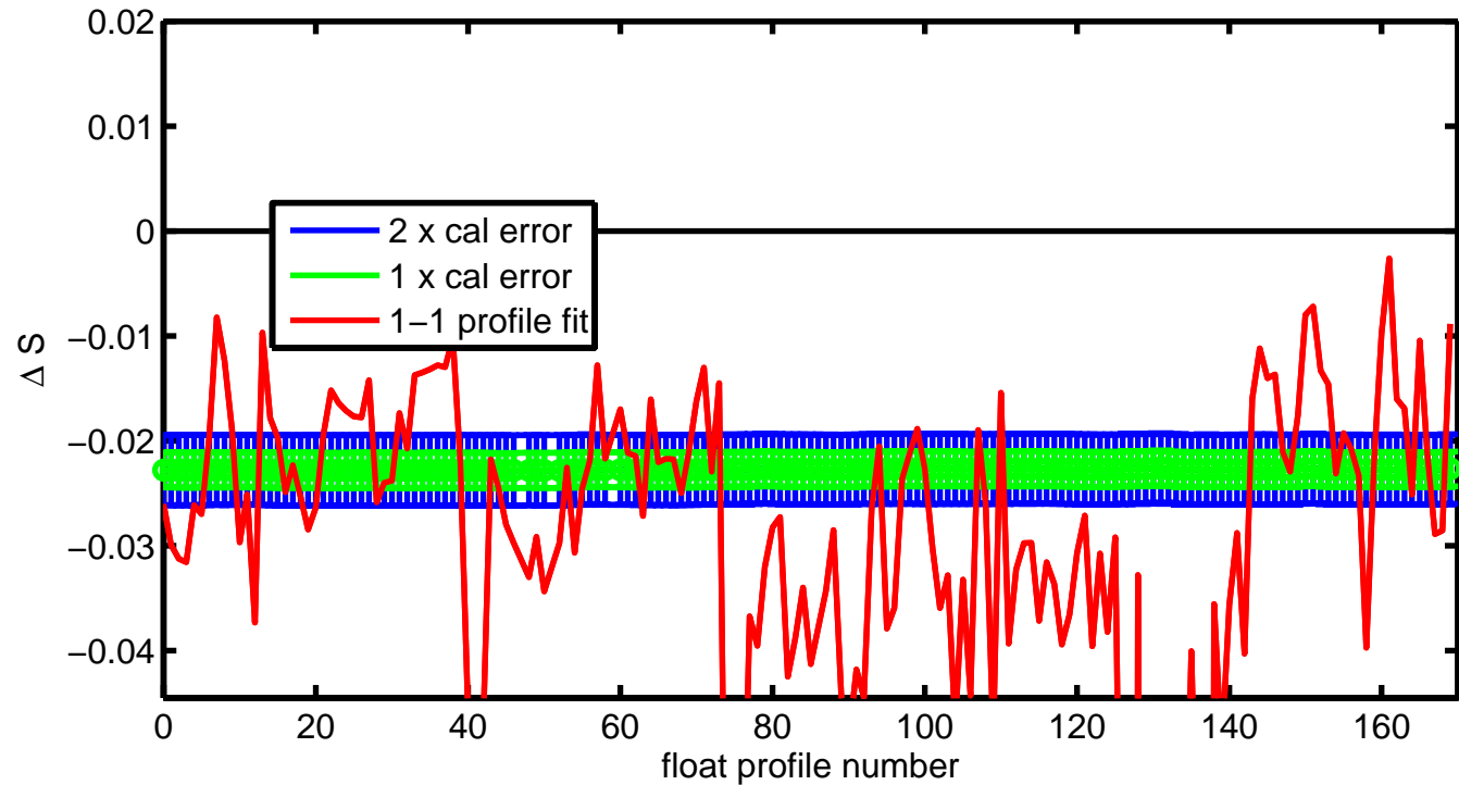
6900457 vertically-averaged salinity (PSS-78) additive correction \Delta S with errors
