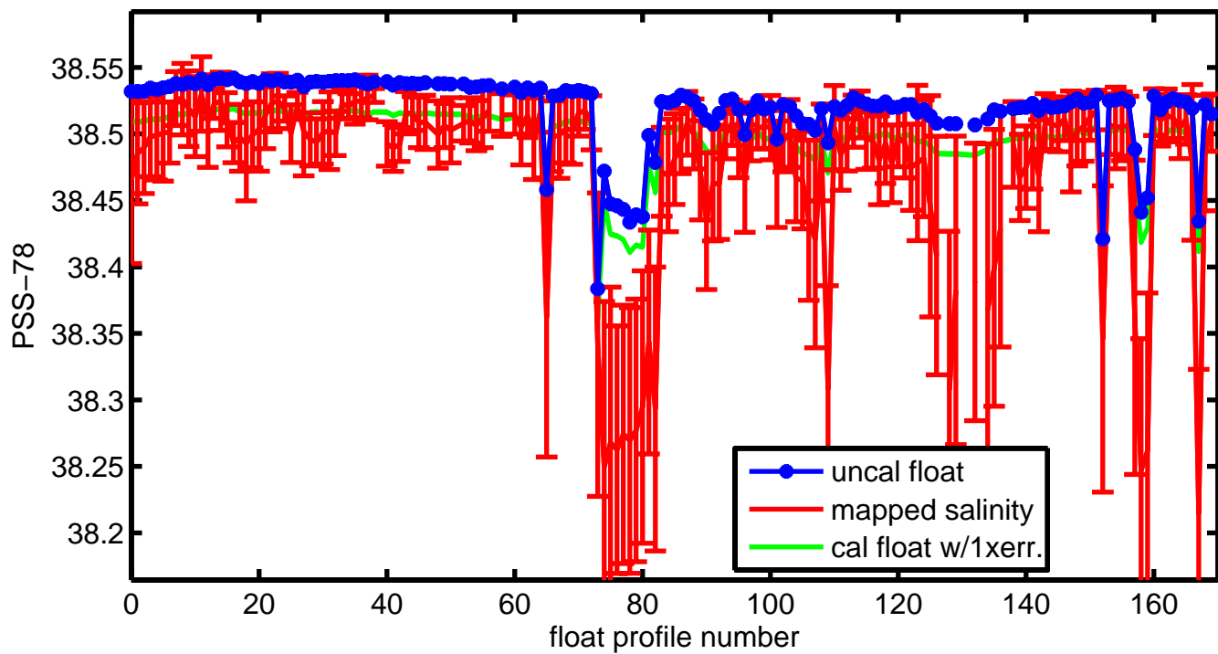
6900457 salinities with error on \theta=13.181^\circ\text{C}
