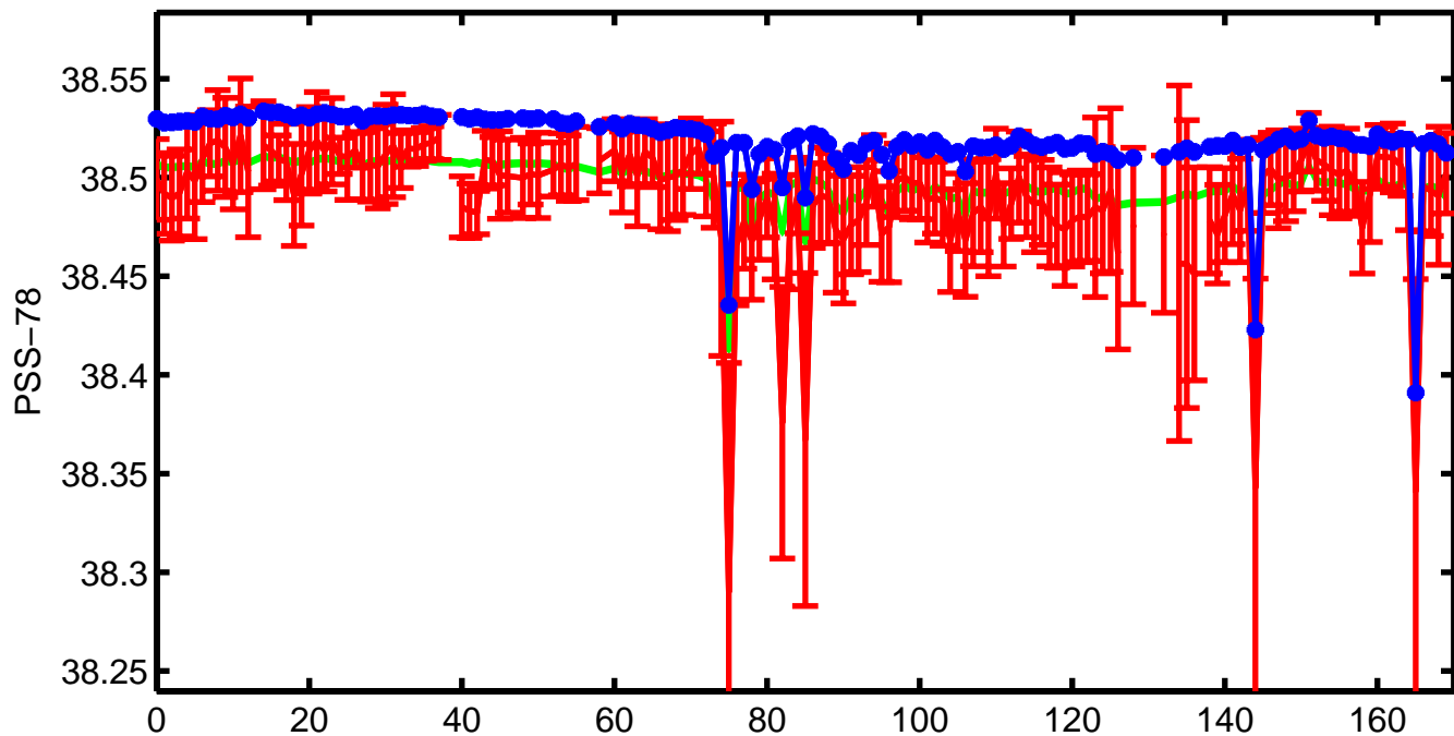
6900457 salinities with error on \theta=13.1459^\circ\text{C}
