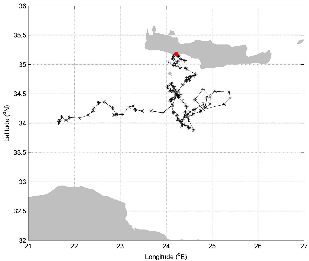
Figure 1. Float trajectory (the red dot represents the last float position).
