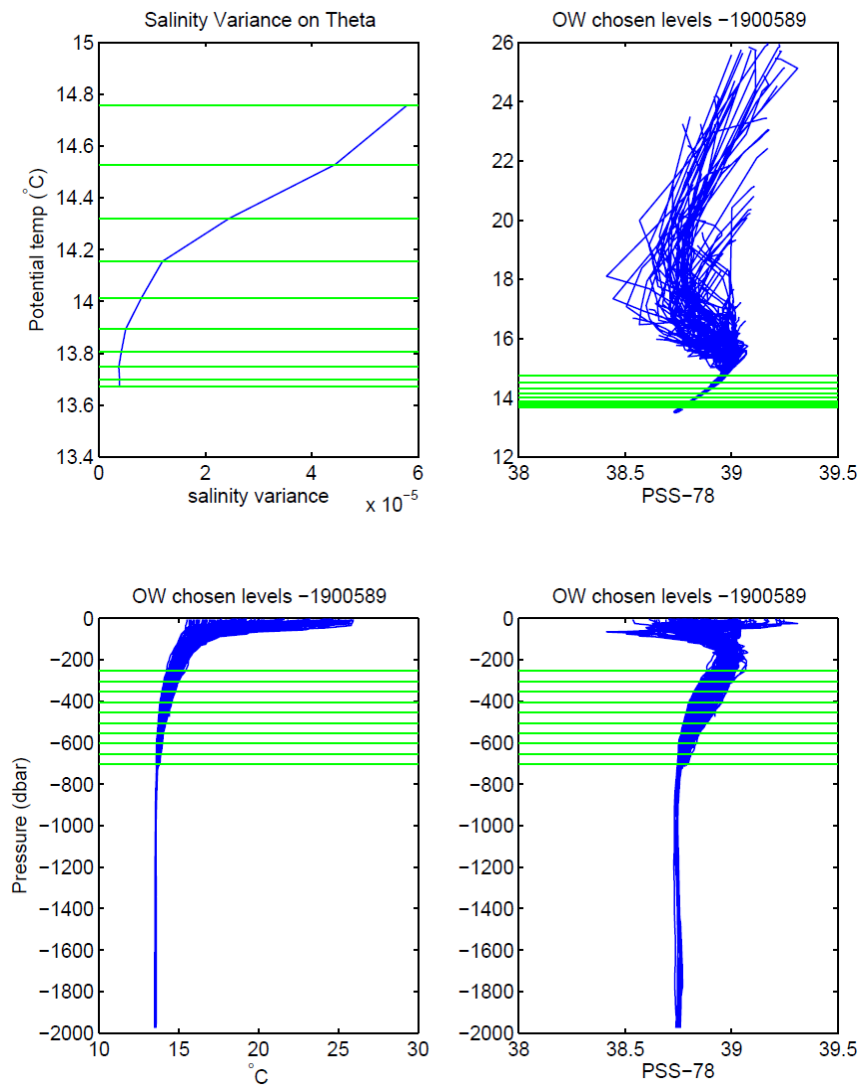
Figure 11. The 10 \theta -levels chosen for the correction.
