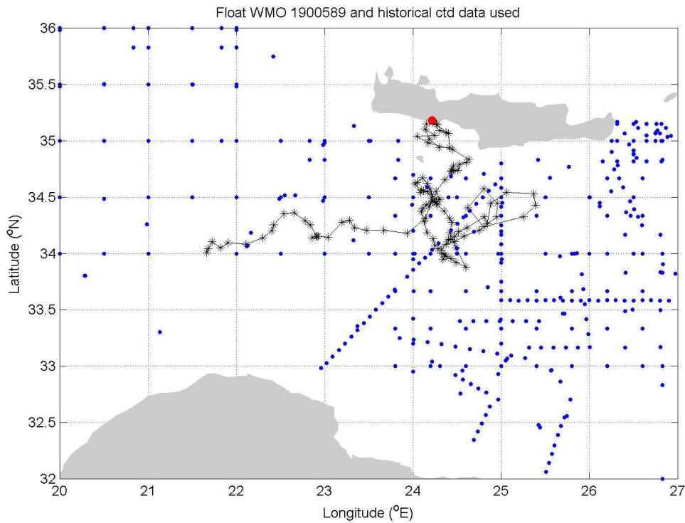
Figure 8. Float trajectory (black line; the last float position is depicted by a red dot) and locations of the historical CTD data.
