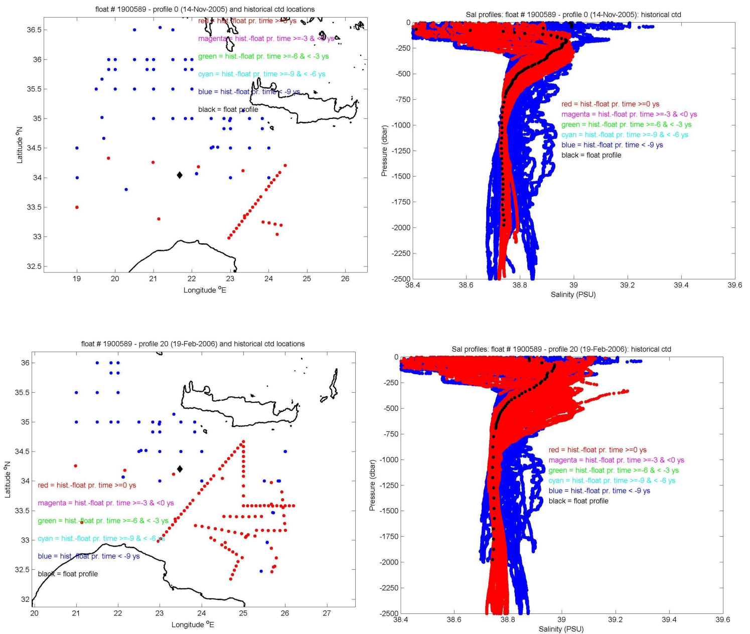
Figure 10. Location of selected float profiles and historical CTD data (left panels) and the respective salinity profiles (right panels).
