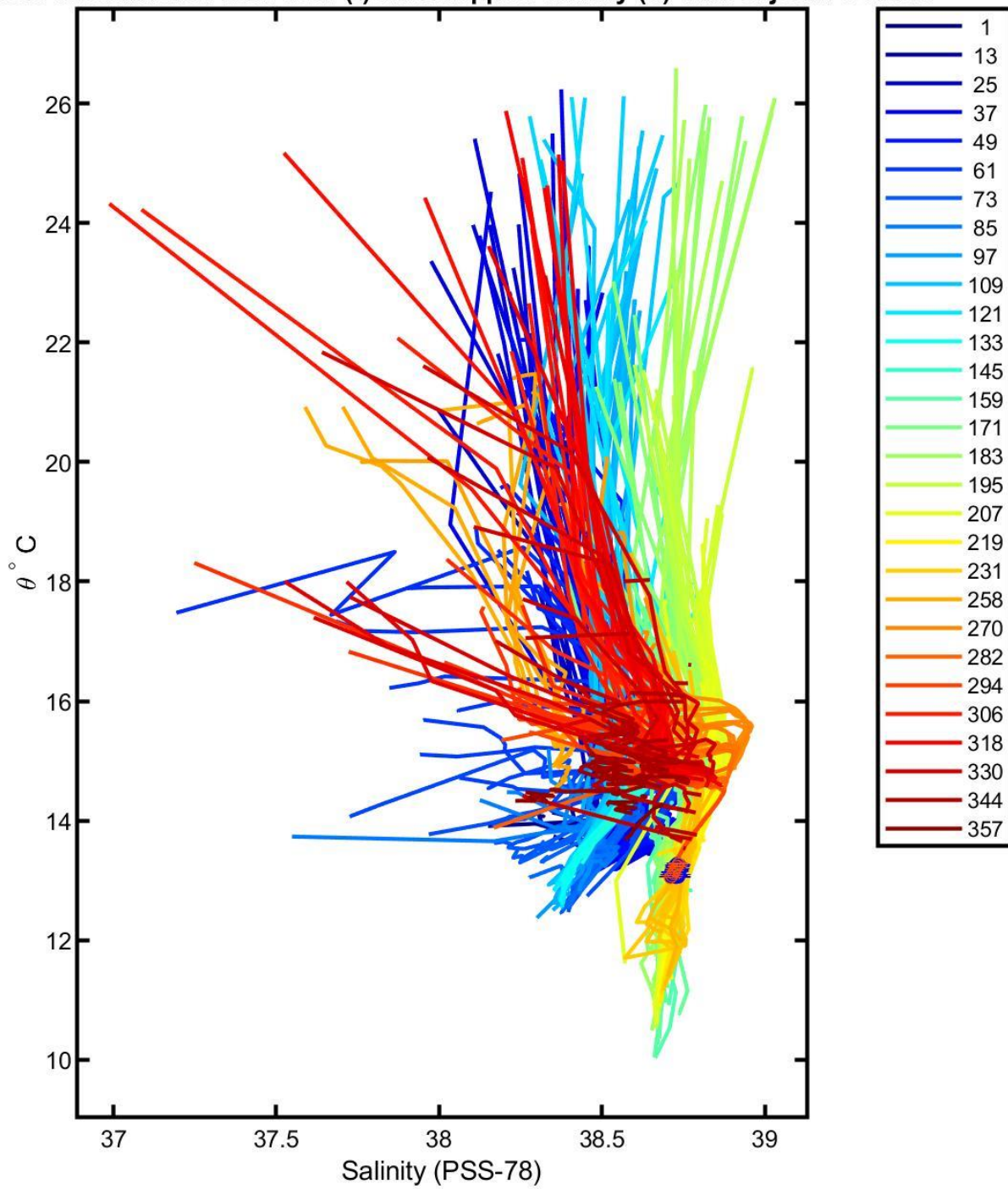
1900848 uncalibrated float data (-) and mapped salinity (o) with objective errors
