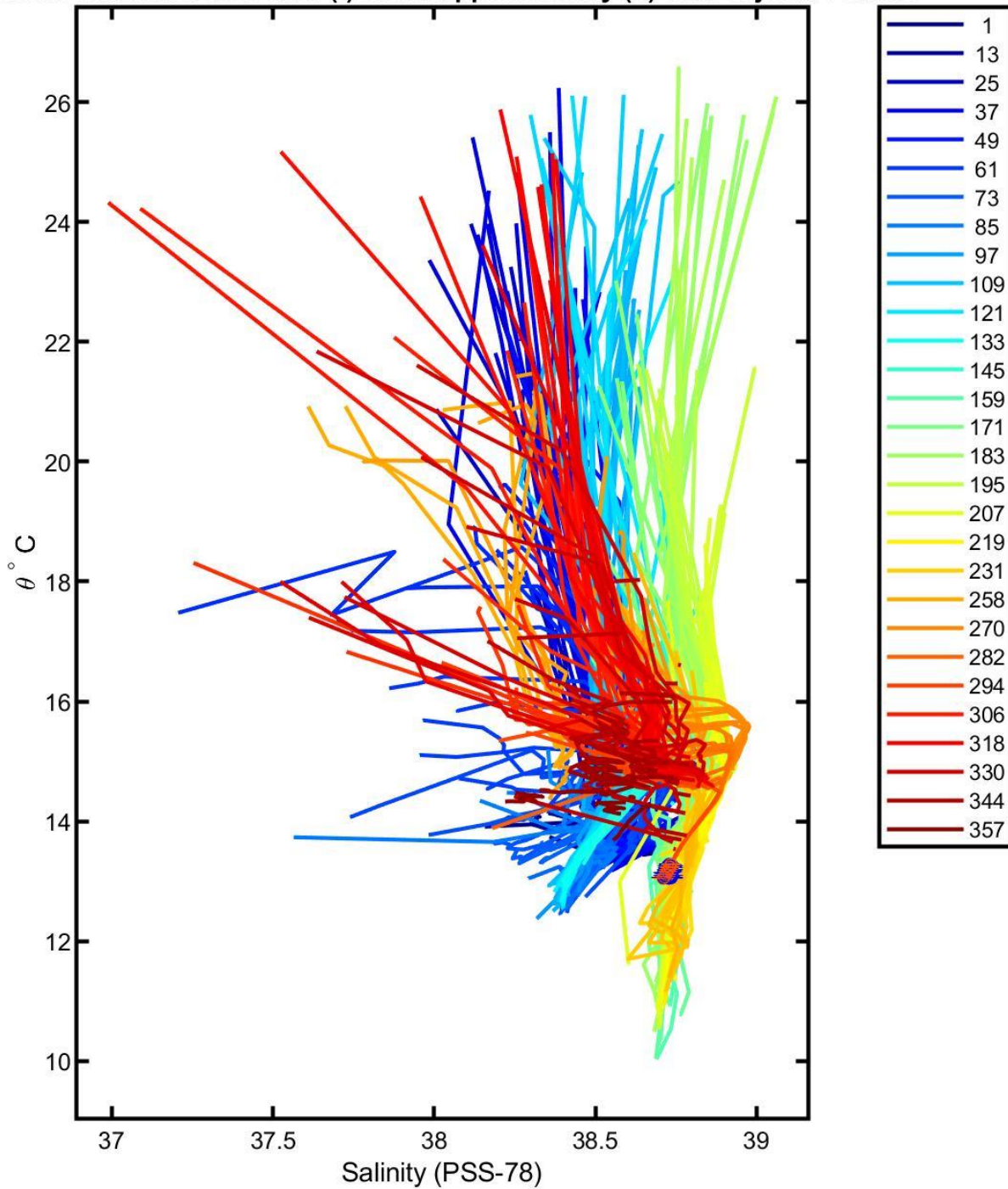
1900848 calibrated float data (-) and mapped salinity (o) with objective errors
