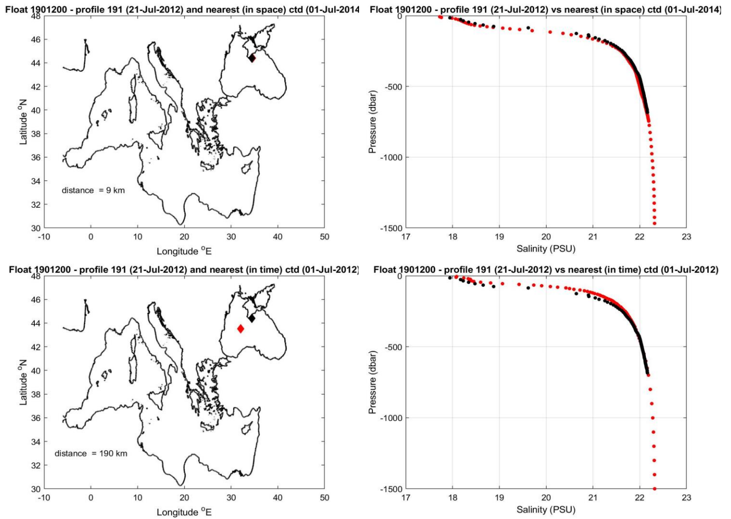
Figure 11: Float 1901200. The salinity float profile number 191 (black dots) are compared to the nearest in space (top) and in time (bottom) reference profile (red dots). The locations of the two profiles and their distance is given in the left panel.
