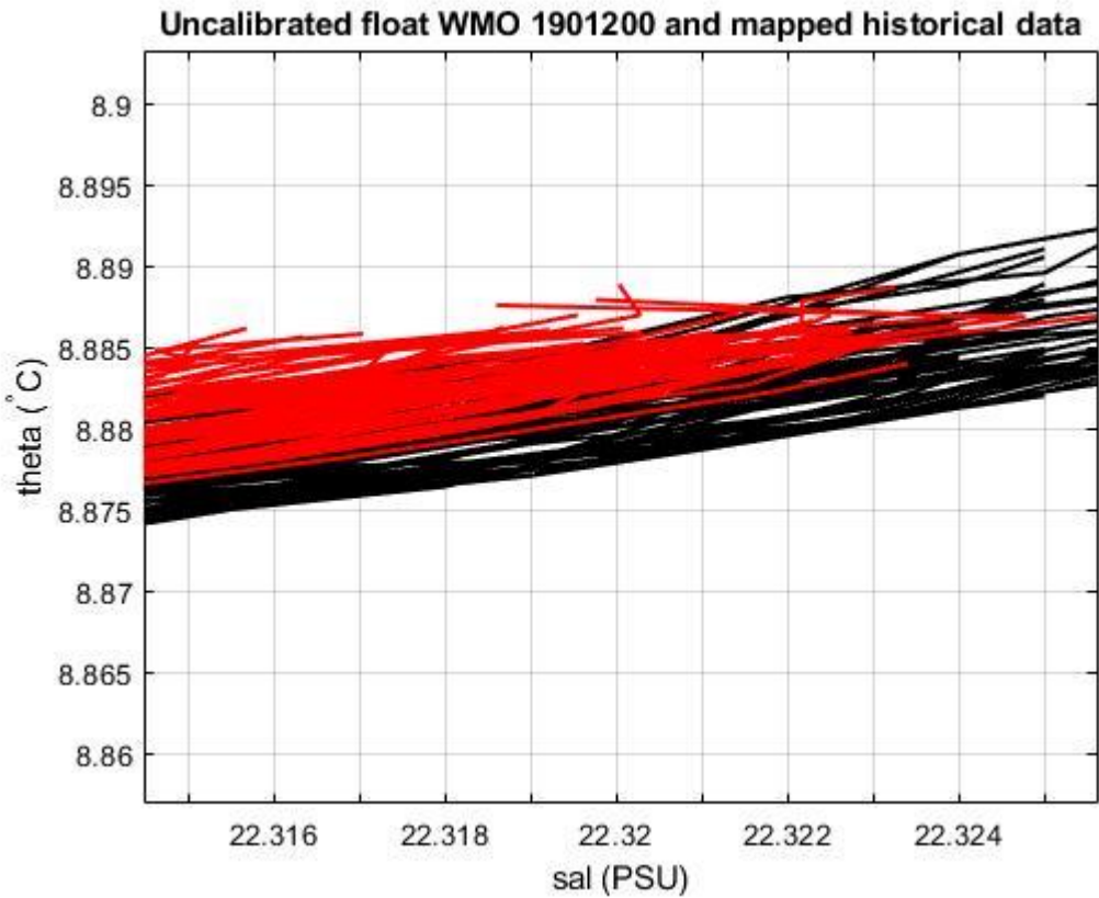
Figure 19: Float 1901200. Uncalibrated float salinity profile (black lines) and mapped historical data (red lines) in the most uniform part of the \theta -S curve.
