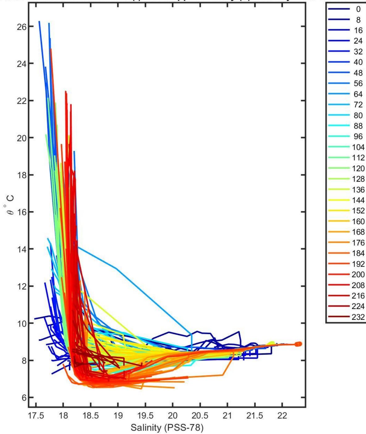
1901200 uncalibrated float data (-) and mapped salinity (o) with objective errors
