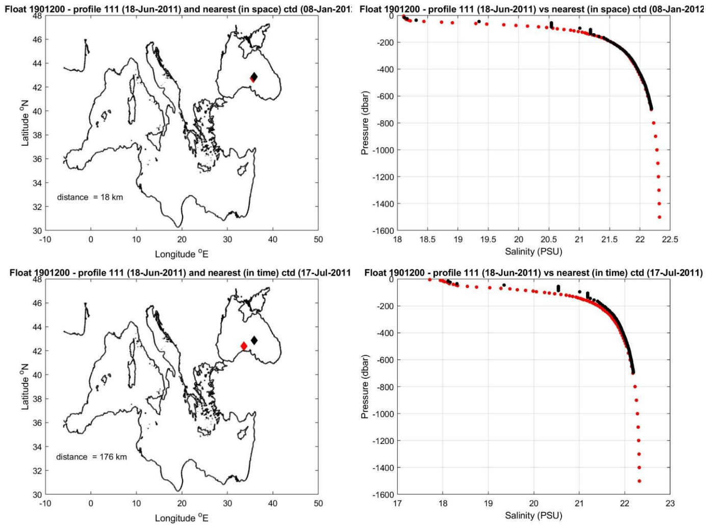
Figure 10: Float 1901200. The salinity float profile number 111 (black dots) are compared to the nearest in space (top) and in time (bottom) reference profile (red dots). The locations of the two profiles and their distance is given in the left panel.
