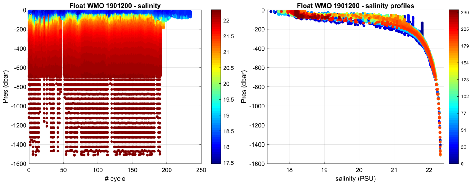
Figure 3: Float 1901200. Time series of Argo float potential salinity (PSS-78) on the left, and salinity profiles color-coded per cycle number on the right.
