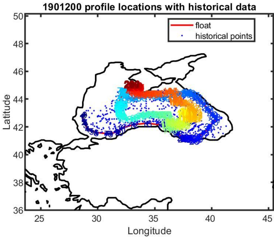
Figure 13: Float 1901200. Location of the float profiles (red line with colored numbers) and the reference data selected for mapping (blue dots).
