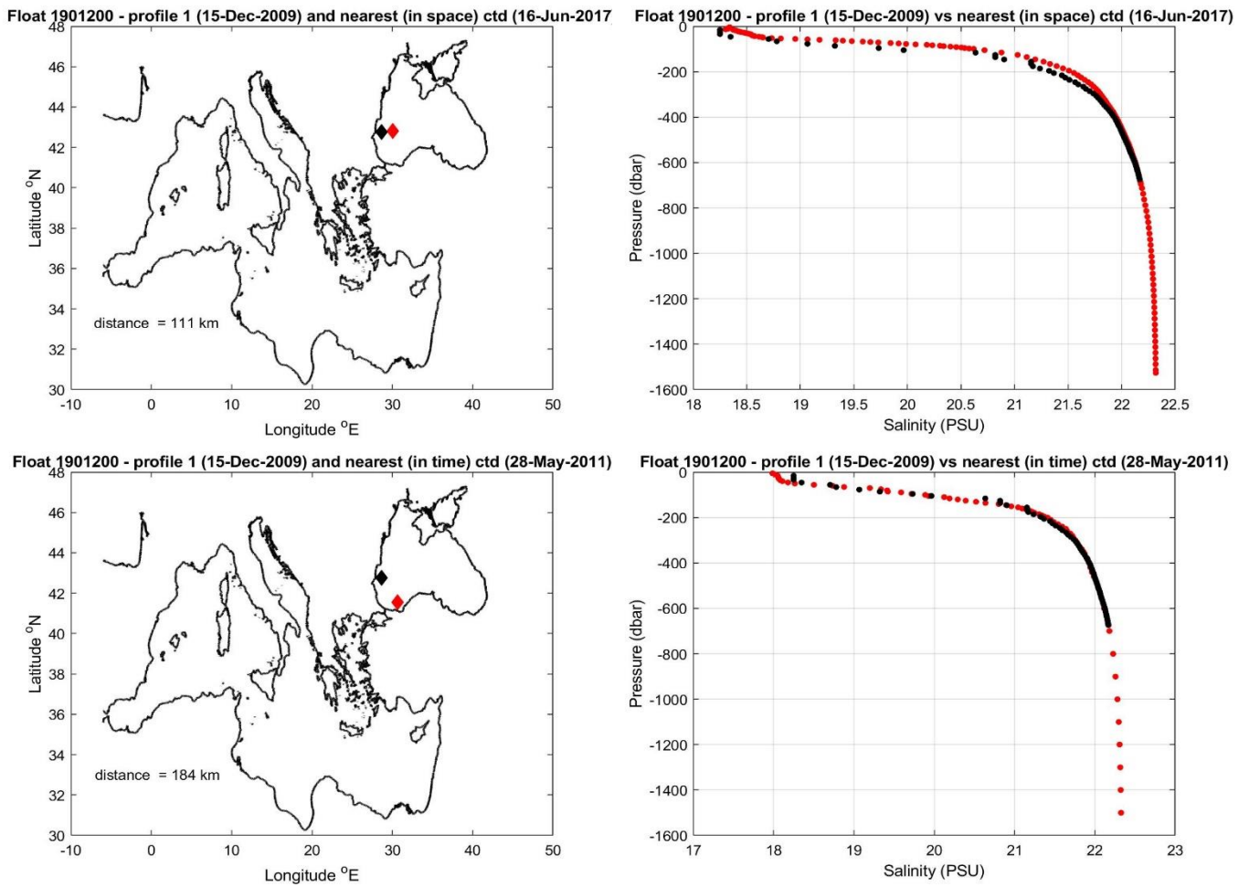
Figure 9: Float 1901200. The salinity float profile number 1 (black dots) are compared to the nearest in space (top) and in time (bottom) reference profile (red dots). The locations of the two profiles and their distance is given in the left panel.
