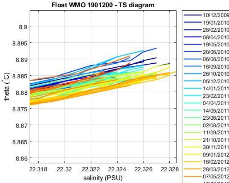
Figure 5: Float 1901200. Area of the \theta -S diagram (color-coded per cycle number) where the \theta -S relationship is more uniform.
