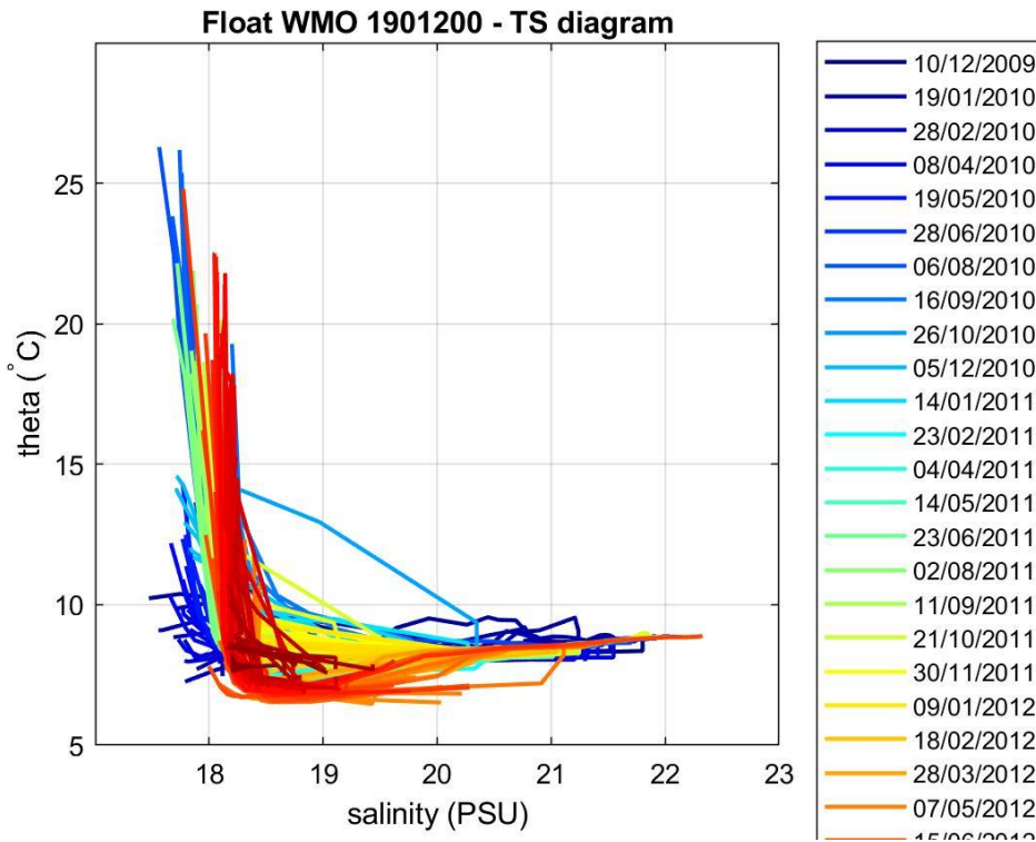
Figure 4: Float 1901200. \theta -S diagram color-coded per cycle number.
