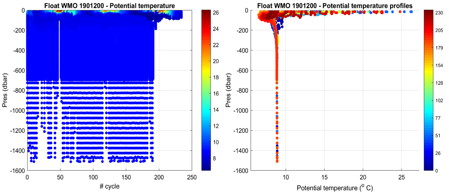
Figure 2: Float 1901200. Time series of Argo float potential temperature (°C) on the left, and potential temperature profiles color-coded per cycle number on the right.
