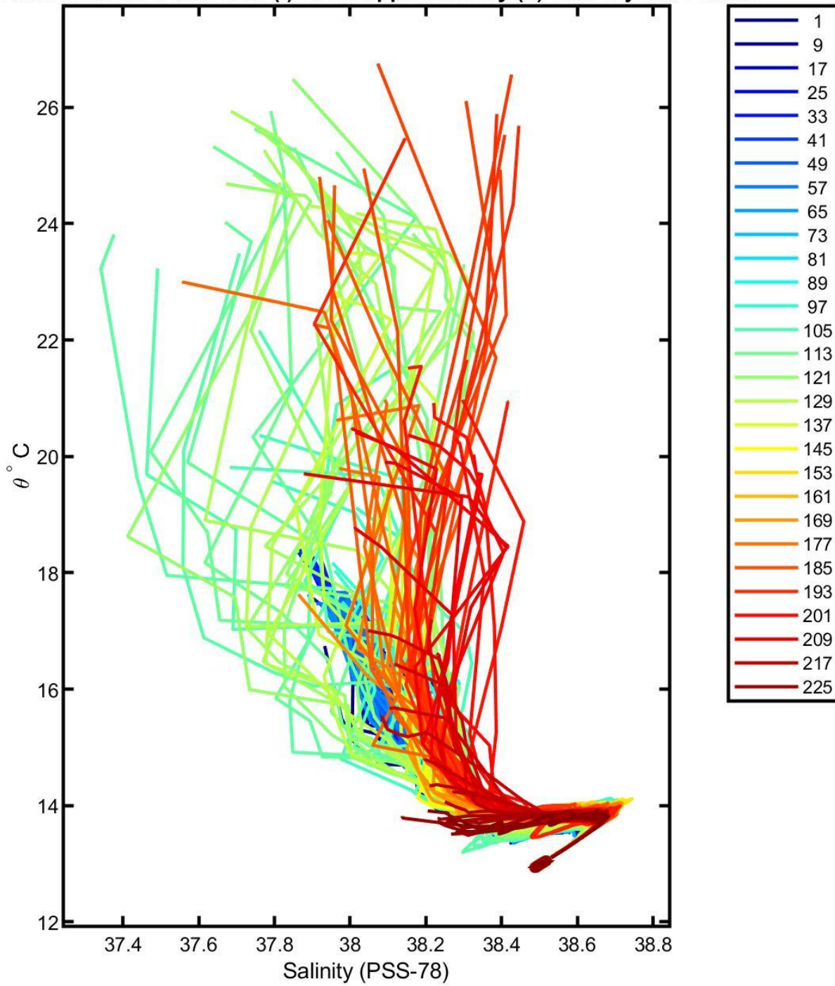
1902605 calibrated float data (-) and mapped salinity (o) with objective errors
