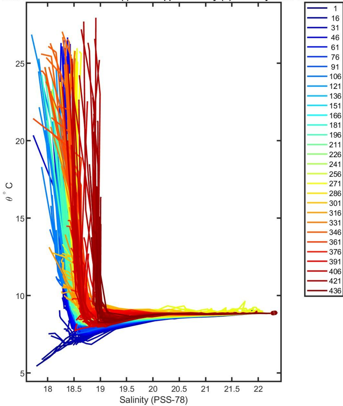
3901852 uncalibrated float data (-) and mapped salinity (o) with objective errors
