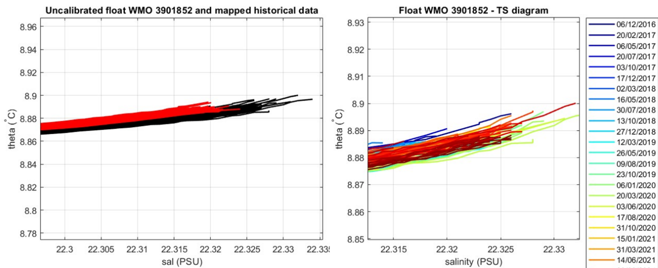
Figure 7: Comparison between float 3901852 and historical CTD on the left and \theta -S diagram color-coded per cycle number on the right, in the most uniform part of the \theta -S curve.
