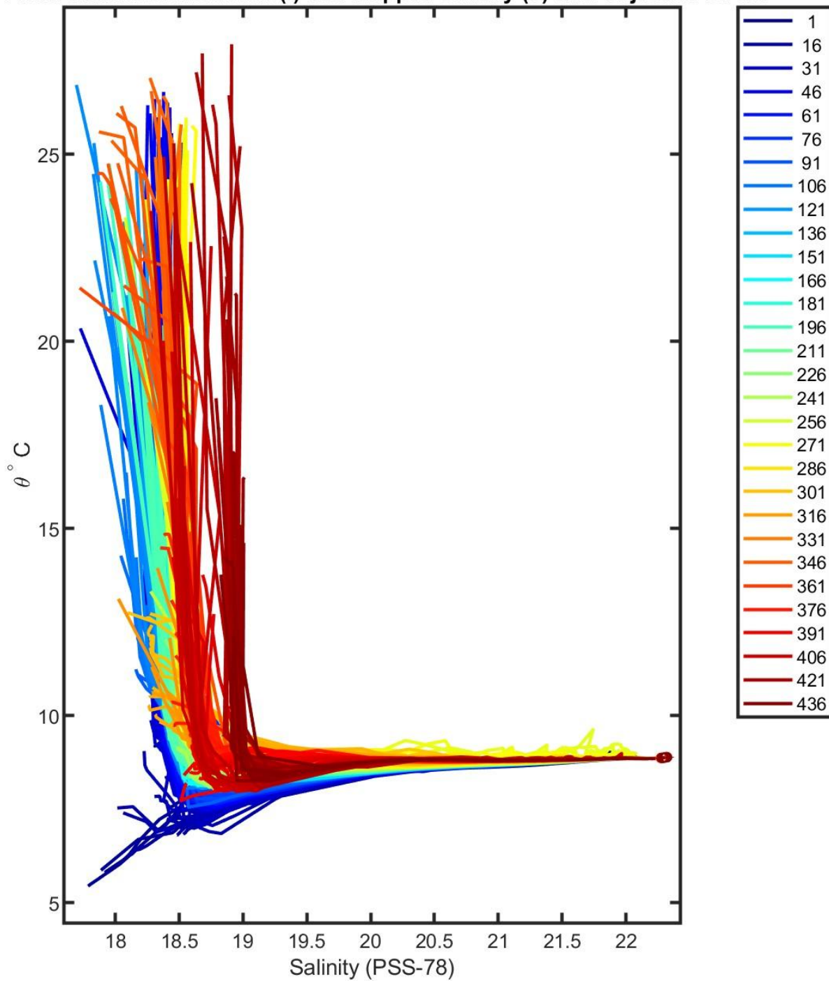
3901852 calibrated float data (-) and mapped salinity (o) with objective errors
