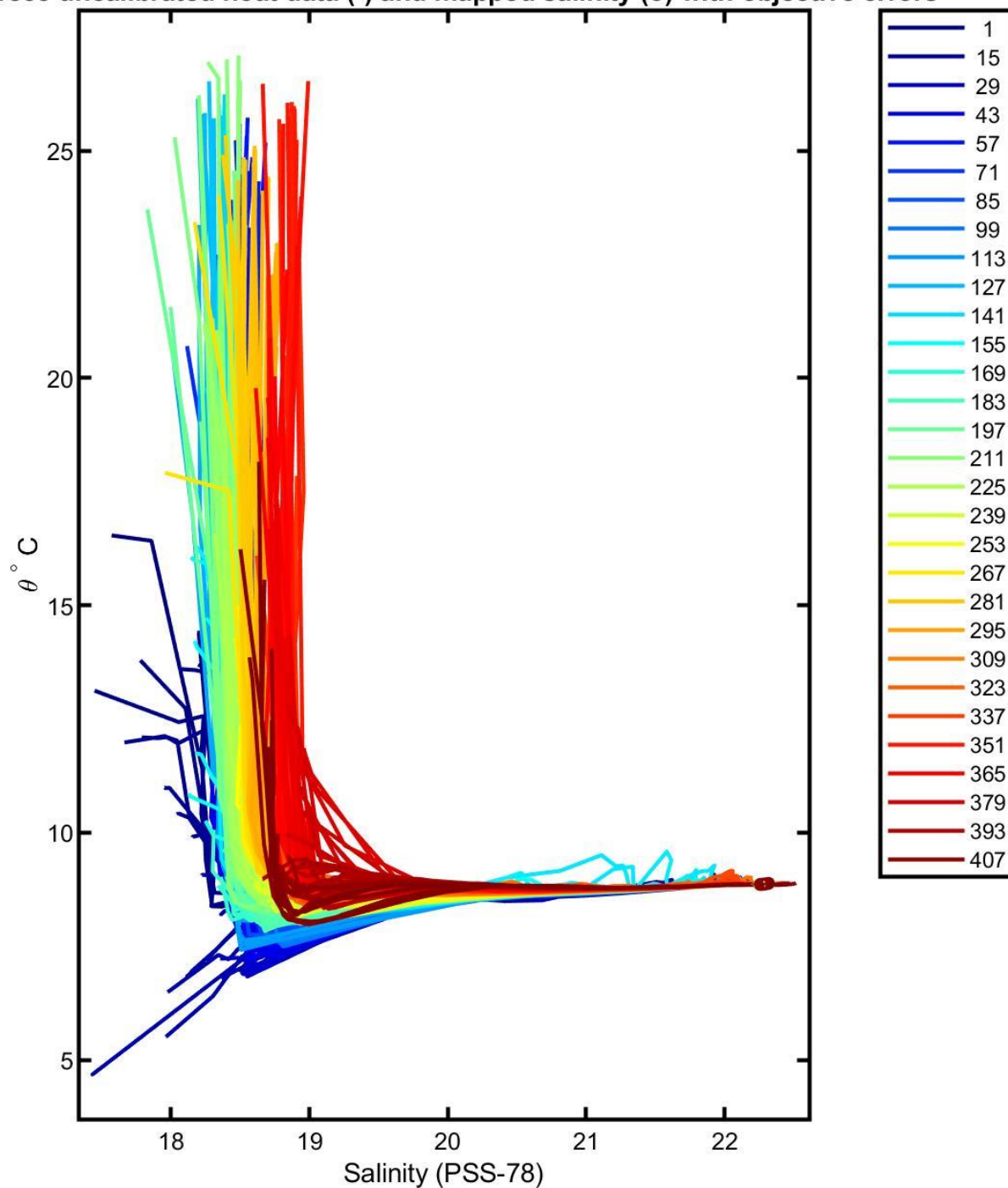
3901855 uncalibrated float data (-) and mapped salinity (o) with objective errors
