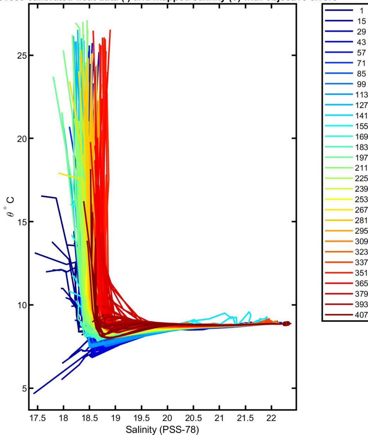
3901855 calibrated float data (-) and mapped salinity (o) with objective errors
