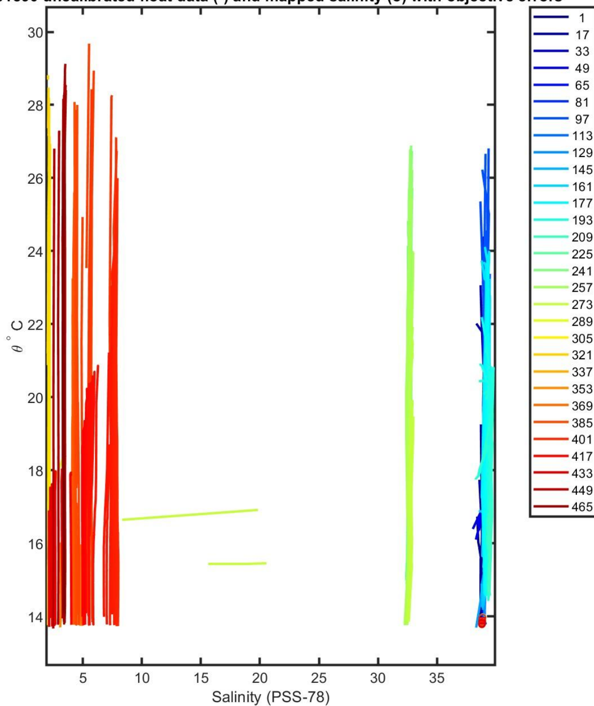
3901890 uncalibrated float data (-) and mapped salinity (o) with objective errors
