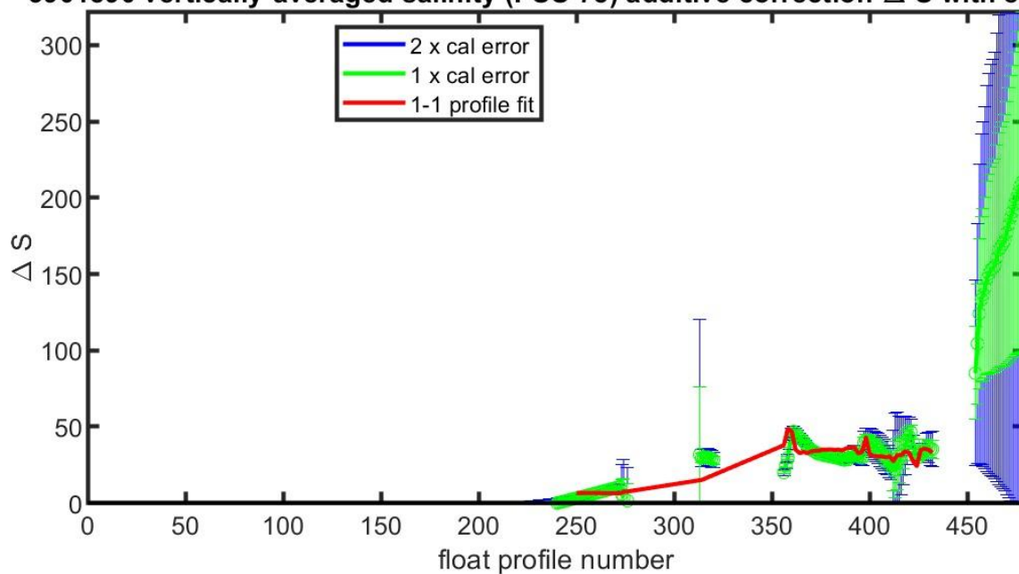
3901890 vertically-averaged salinity (PSS-78) additive correction \Delta S with errors
