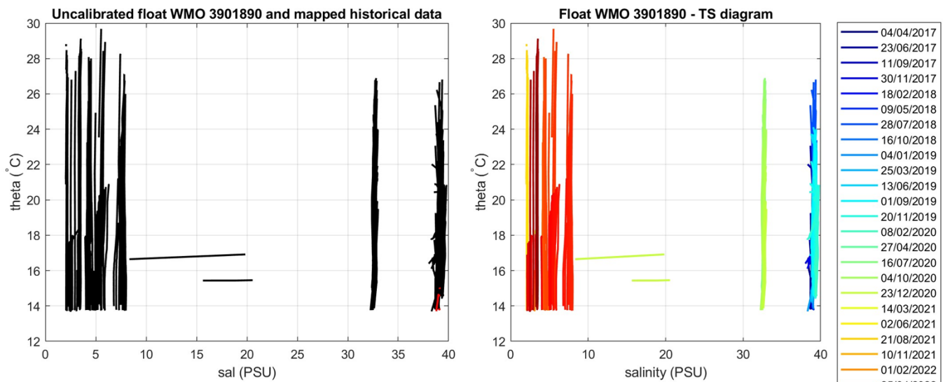
Figure 7: Comparison between float 3901890 and historical CTD on the left and \theta -S diagram color-coded per cycle number on the right, in the most uniform part of the \theta -S curve.
