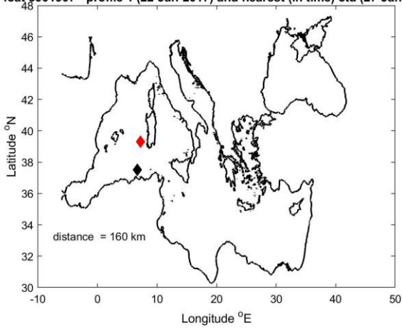
Float 3901907 - profile 1 (22-Jan-2017) and nearest (in time) ctd (27-Jan-2017)
