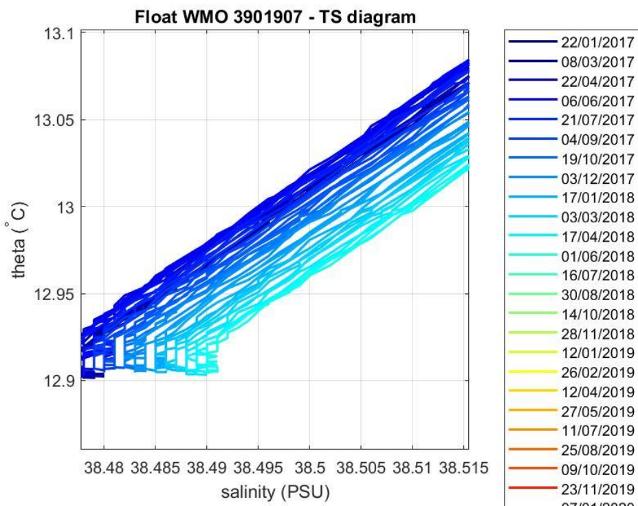
Figure 5: Float 3901907. Area of the \theta -S diagram (color-coded per cycle number) where the \theta -S relationship is more uniform.
