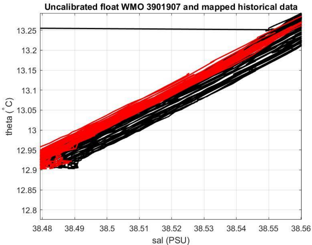
Figure 19: Float 3901907. Uncalibrated float salinity profile (black lines) and mapped historical data (red lines) in the most uniform part of the \theta -S curve.
