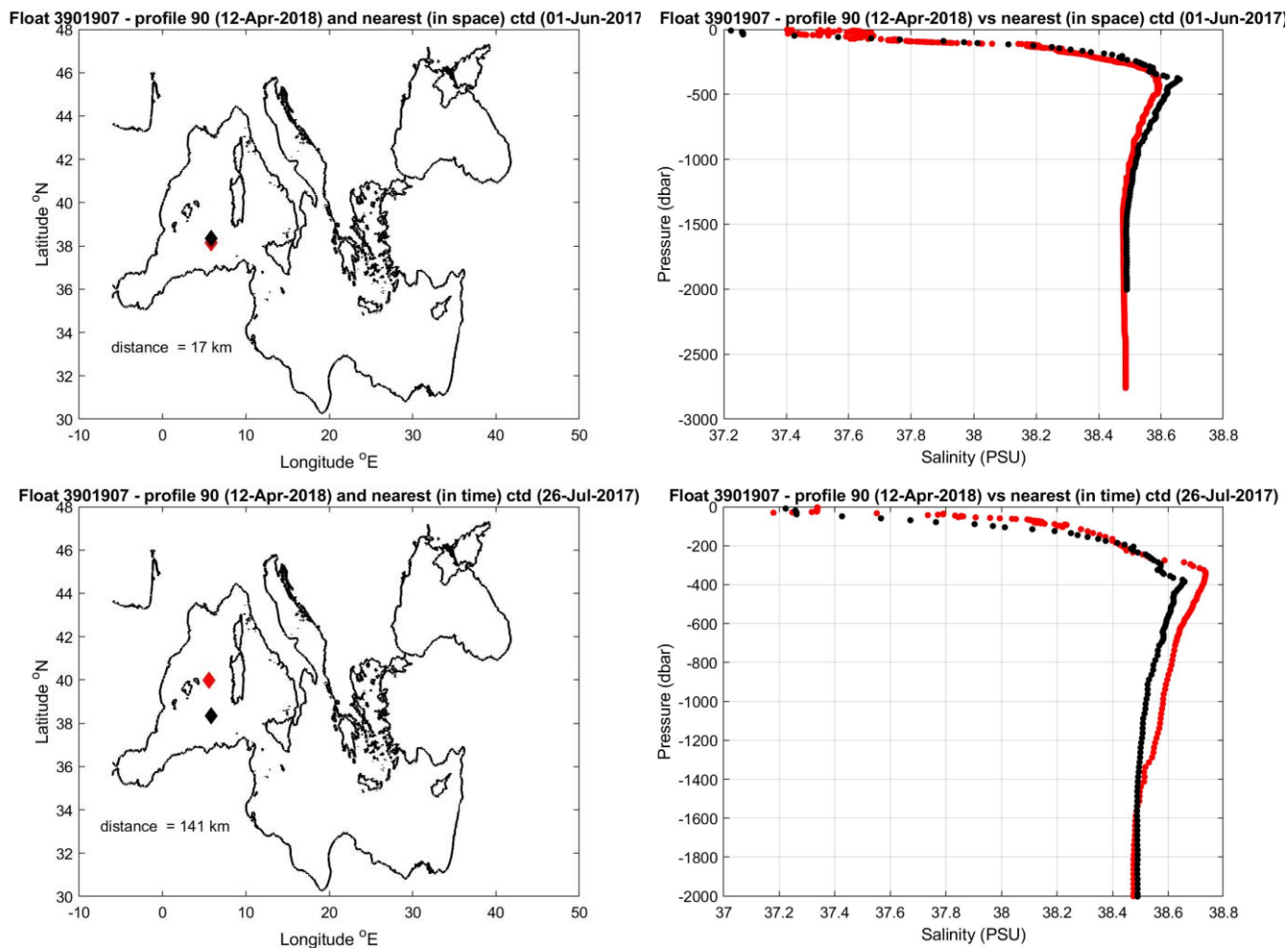
Figure 11: Float 3901907. The salinity float profile number 90 (black dots) are compared to the nearest in space (top) and in time (bottom) reference profile (red dots). The locations of the two profiles and their distance is given in the left panel.
