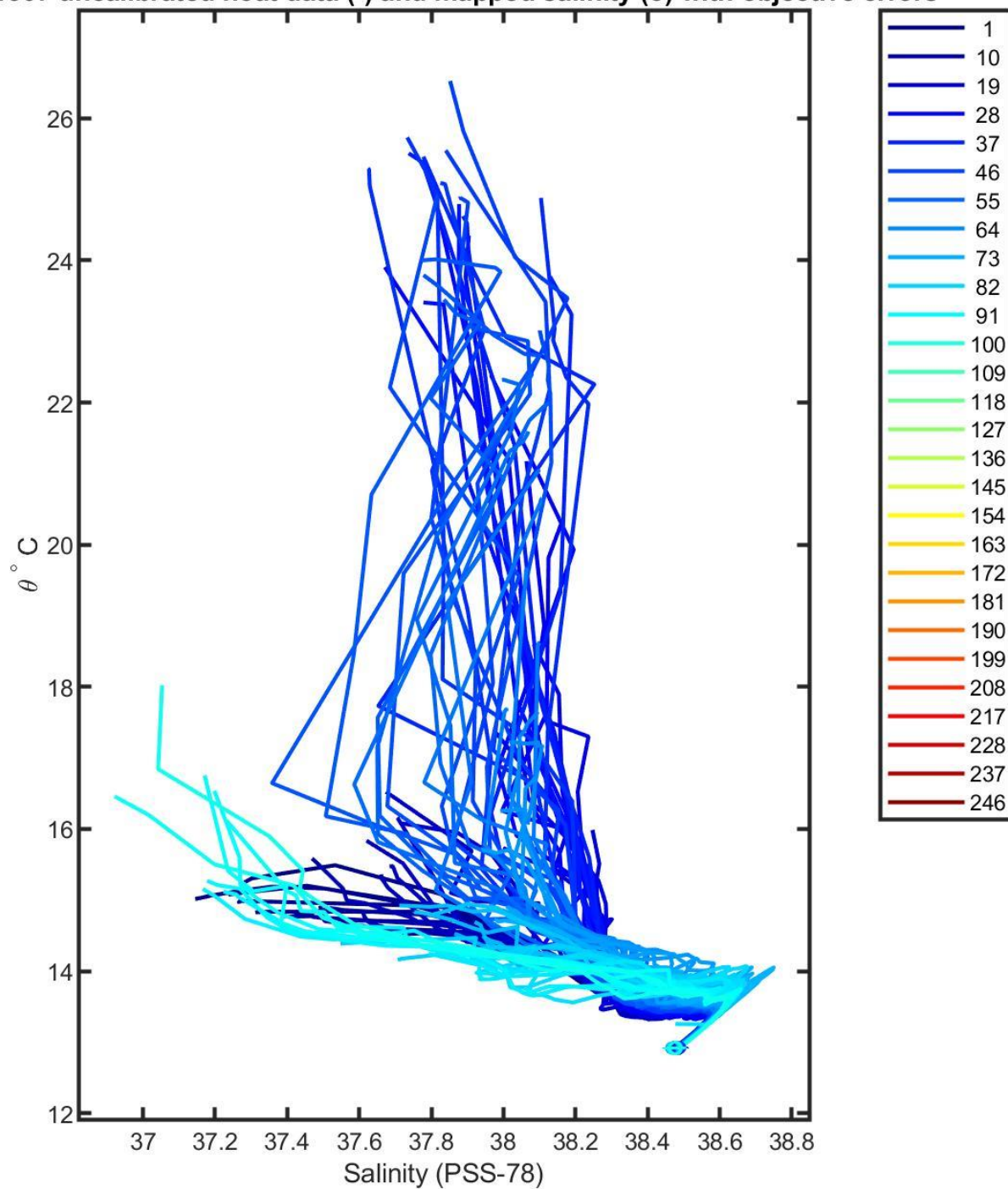
3901907 uncalibrated float data (-) and mapped salinity (o) with objective errors
