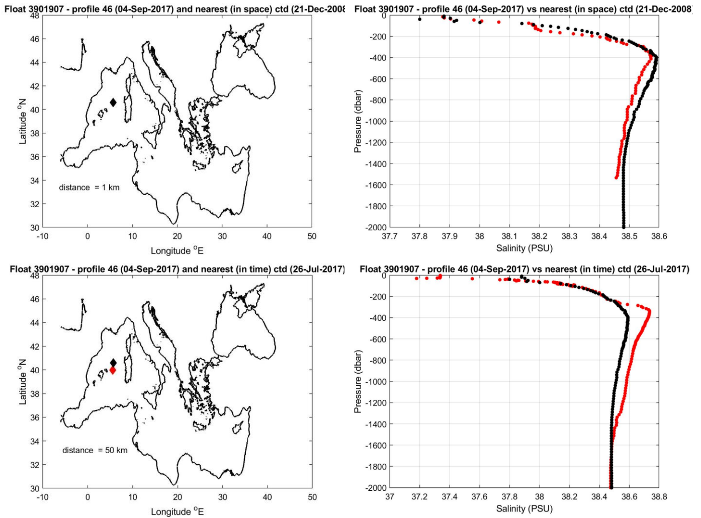
Figure 10: Float 3901907. The salinity float profile number 46 (black dots) are compared to the nearest in space (top) and in time (bottom) reference profile (red dots). The locations of the two profiles and their distance is given in the left panel.
