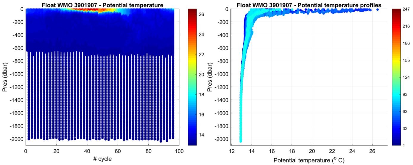
Figure 2: Float 3901907. Time series of Argo float potential temperature ( ^{\circ}\text{C} ) on the left, and potential temperature profiles color-coded per cycle number on the right.
