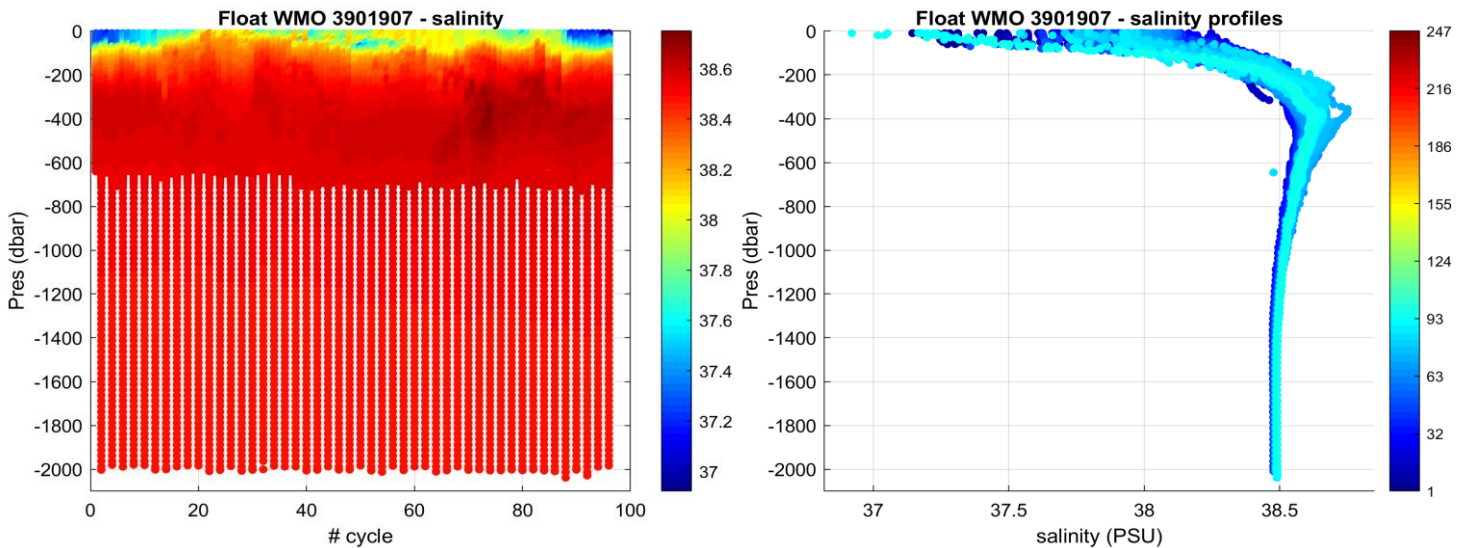
Figure 3: Float 3901907. Time series of Argo float potential salinity (PSS-78) on the left, and salinity profiles color-coded per cycle number on the right.
