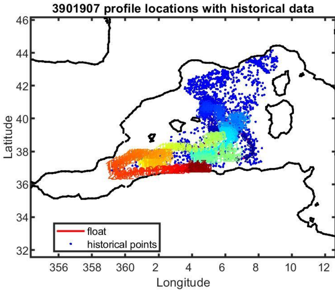
Figure 13: Float 3901907. Location of the float profiles (red line with colored numbers) and the reference data selected for mapping (blue dots).
