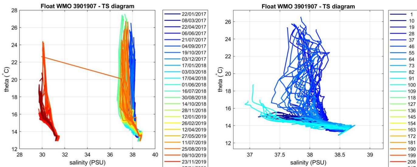
Figure 4: Float 3901907. \theta -S diagram color-coded per cycle number. On the left all profiles, on the right profiles with PSAL QC 1.
