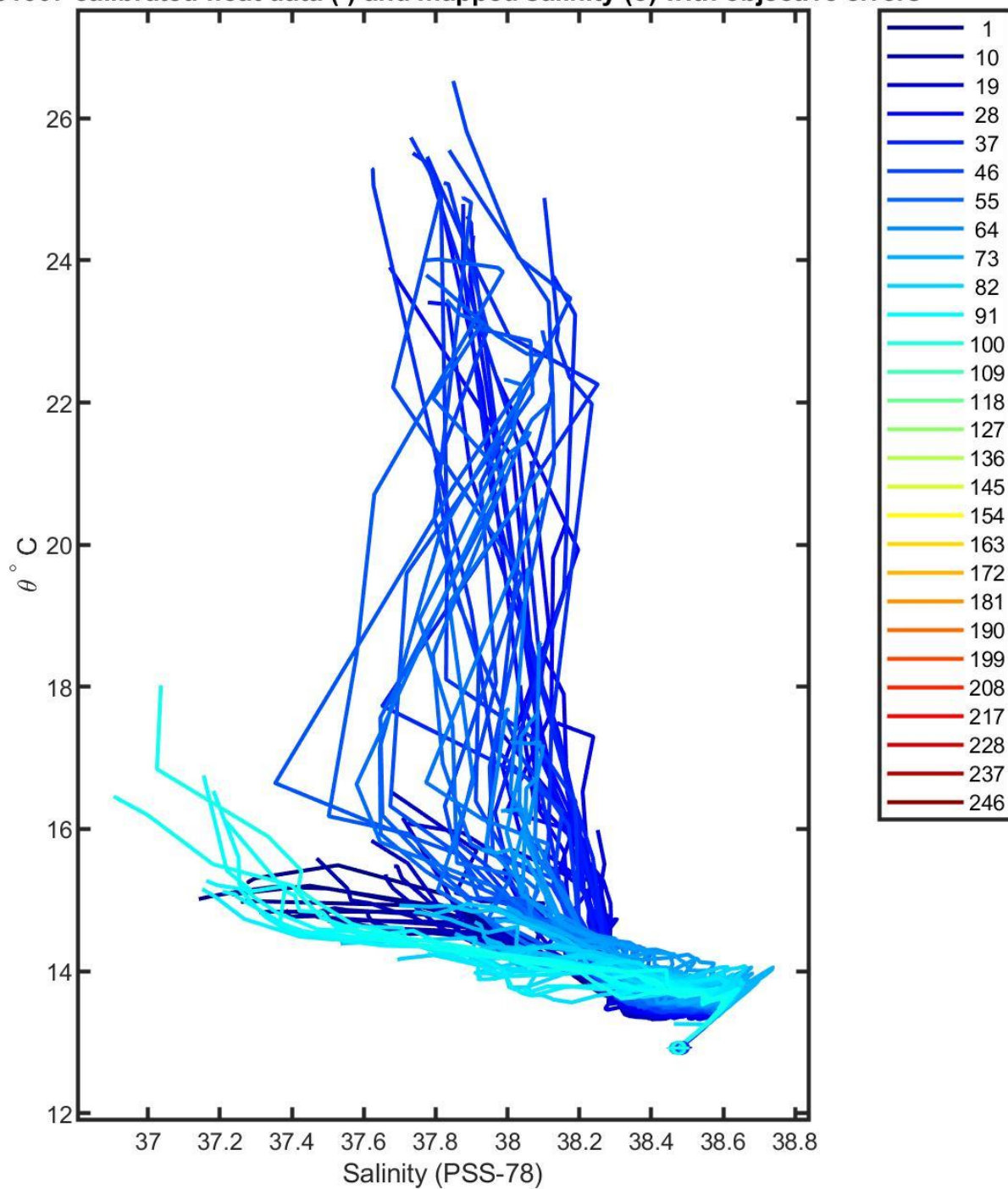
3901907 calibrated float data (-) and mapped salinity (o) with objective errors
