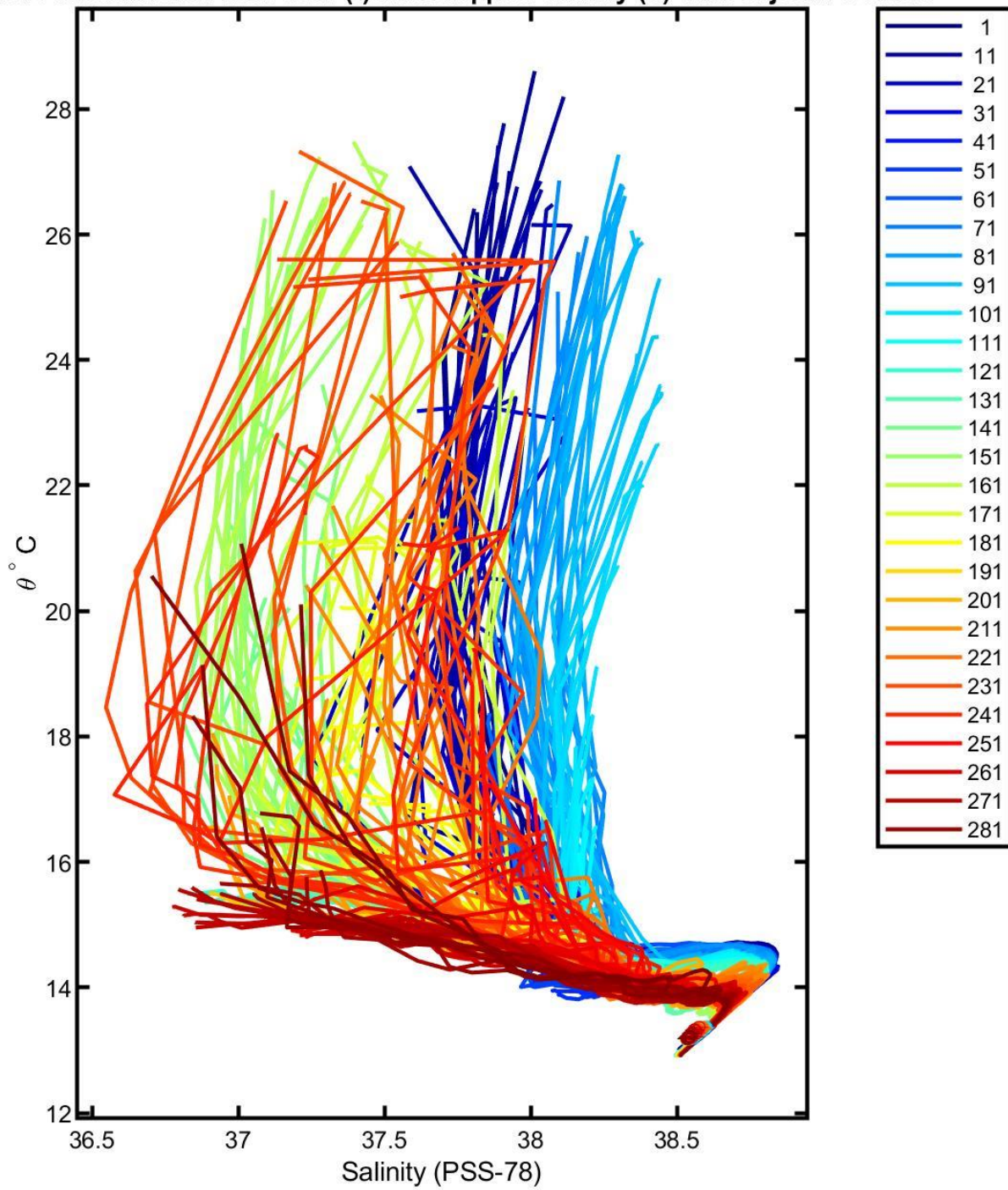
3901975 uncalibrated float data (-) and mapped salinity (o) with objective errors
