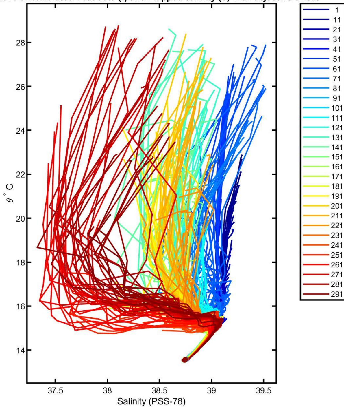
3901976 uncalibrated float data (-) and mapped salinity (o) with objective errors
