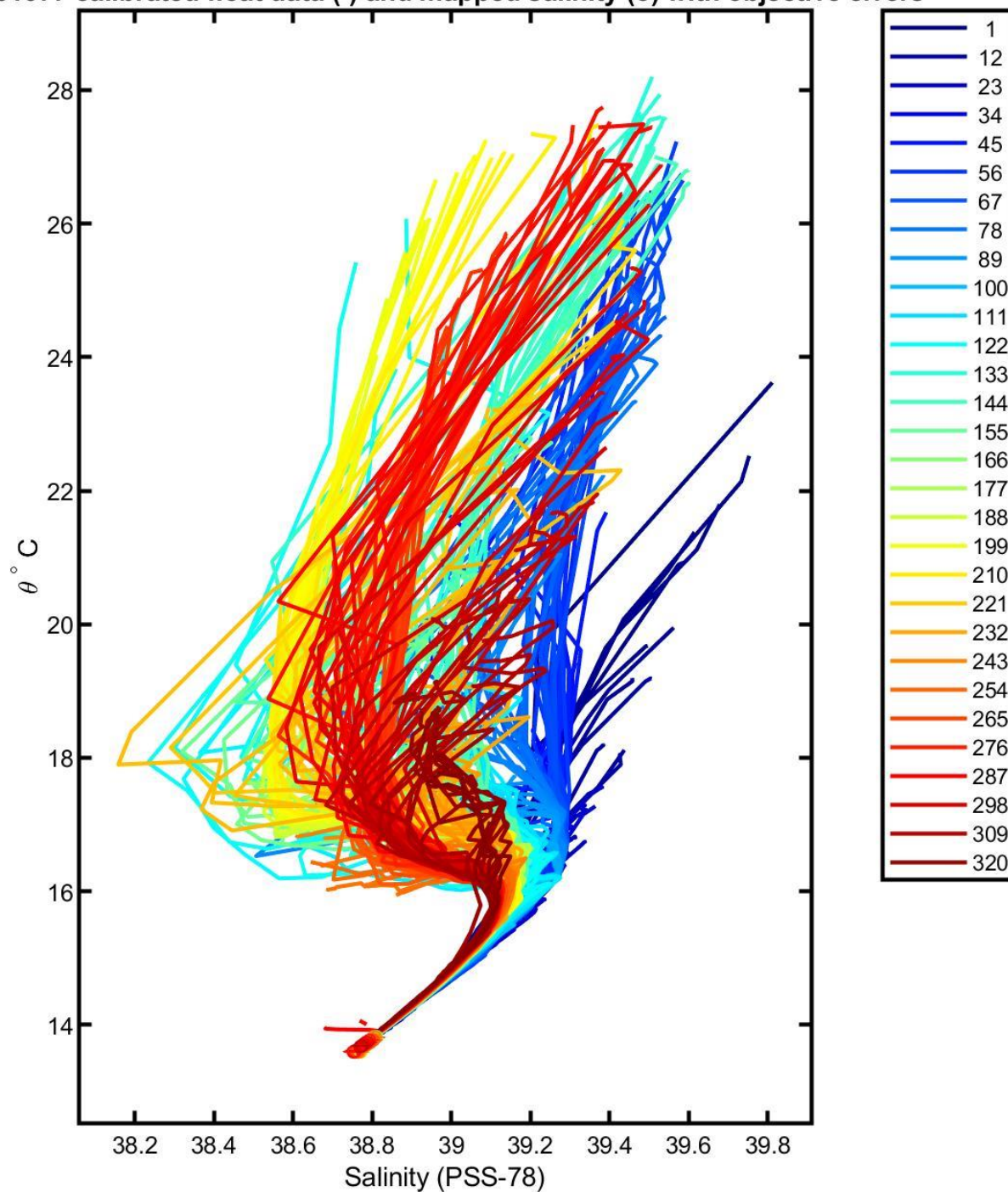
3901977 calibrated float data (-) and mapped salinity (o) with objective errors
