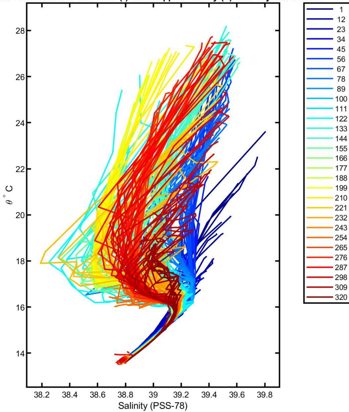
3901977 uncalibrated float data (-) and mapped salinity (o) with objective errors
