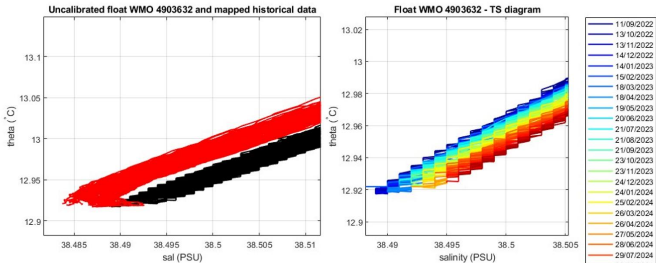
Figure 7: Comparison between float 4903632 and historical CTD on the left and \theta -S diagram color-coded per cycle number on the right, in the most uniform part of the \theta -S curve.
