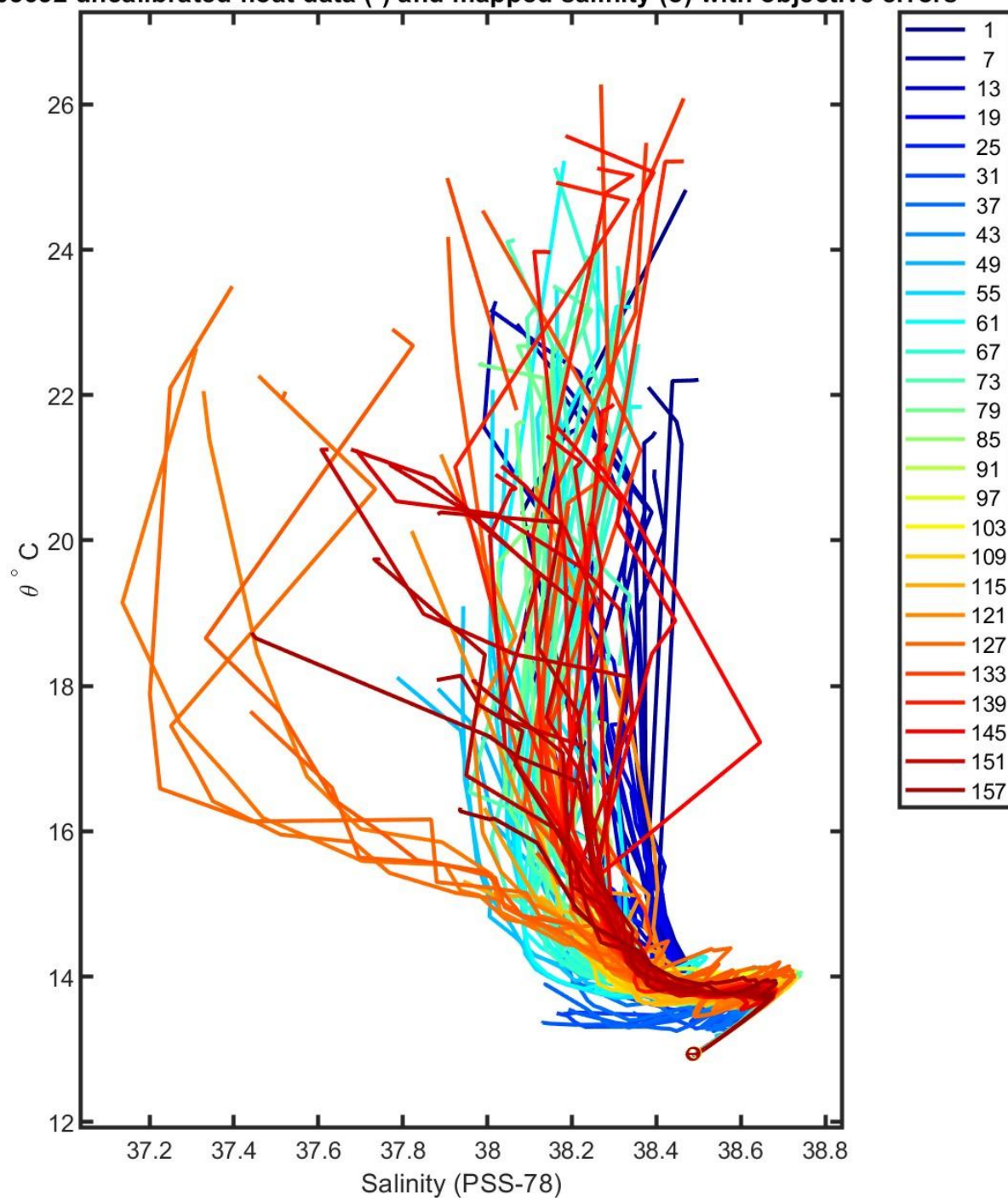
4903632 uncalibrated float data (-) and mapped salinity (o) with objective errors
