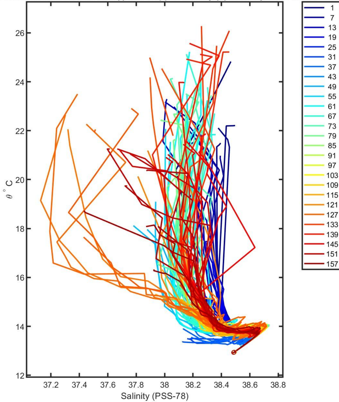
4903632 calibrated float data (-) and mapped salinity (o) with objective errors
