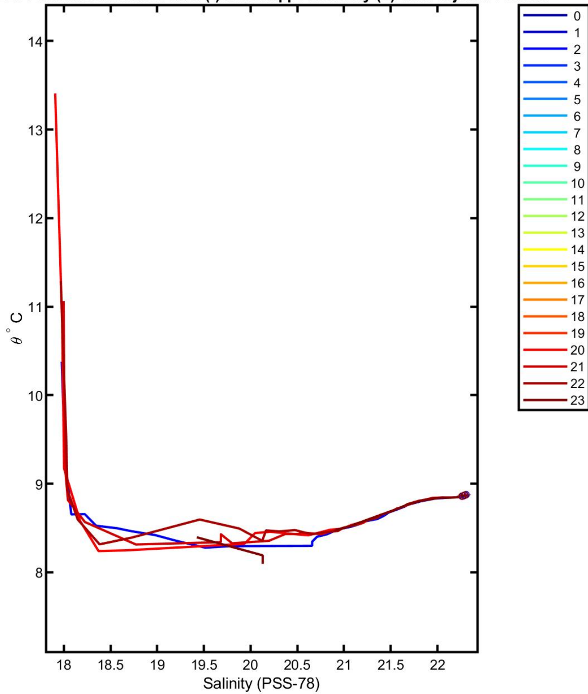
5902291 uncalibrated float data (-) and mapped salinity (o) with objective errors
