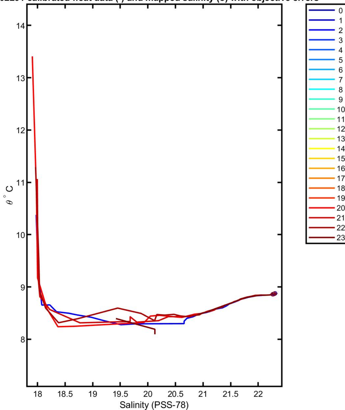
5902291 calibrated float data (-) and mapped salinity (o) with objective errors
