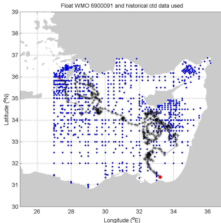
Figure 8. Float trajectory (black line; the first (last) float position is depicted by a red asterisk (dot)) and locations of the historical CTD data.
