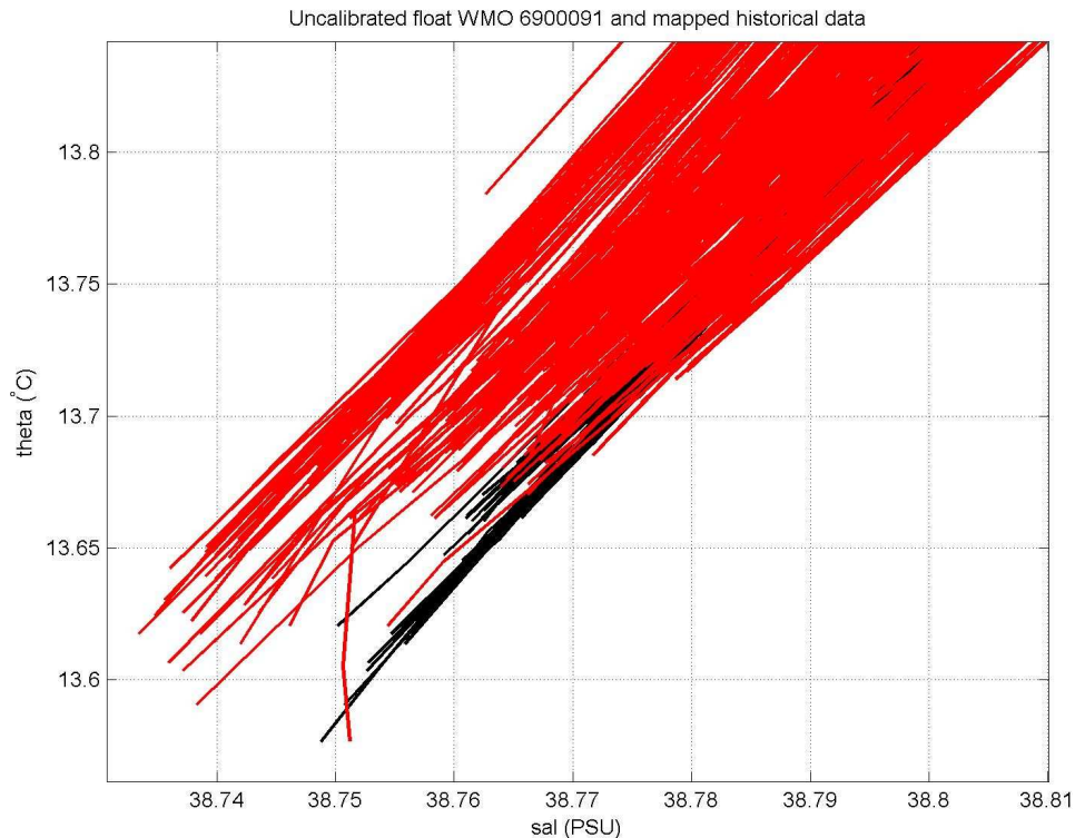
Figure 15. Uncalibrated float SAL_RC profiles (black lines) and mapped historical data (red lines) in the most uniform part of the \theta -S curve.
