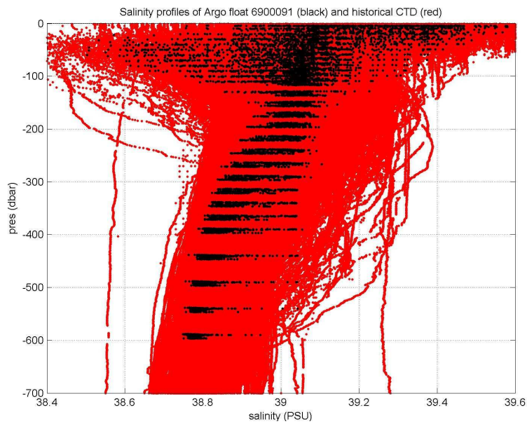
Figure 9. SAL_RC profiles of the Argo float (black lines) and historical CTD (red lines).
