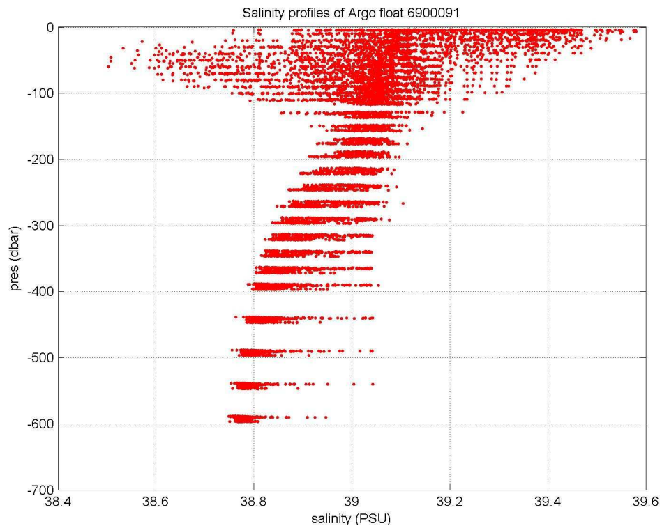
Figure 6. SAL_RC profiles as they are in real time correction mode at Coriolis Data Centre.
