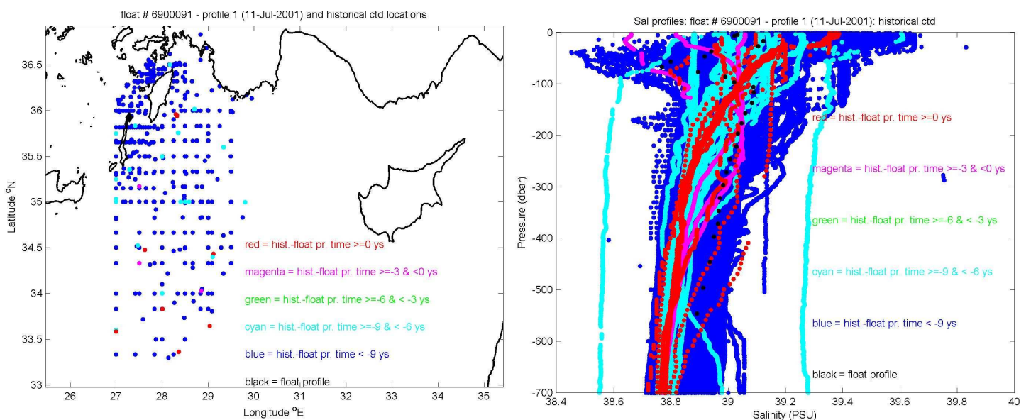
Figure 10. Location of selected float SAL_RC profiles and historical CTD data (left panels) and the respective salinity profiles (right panels).
