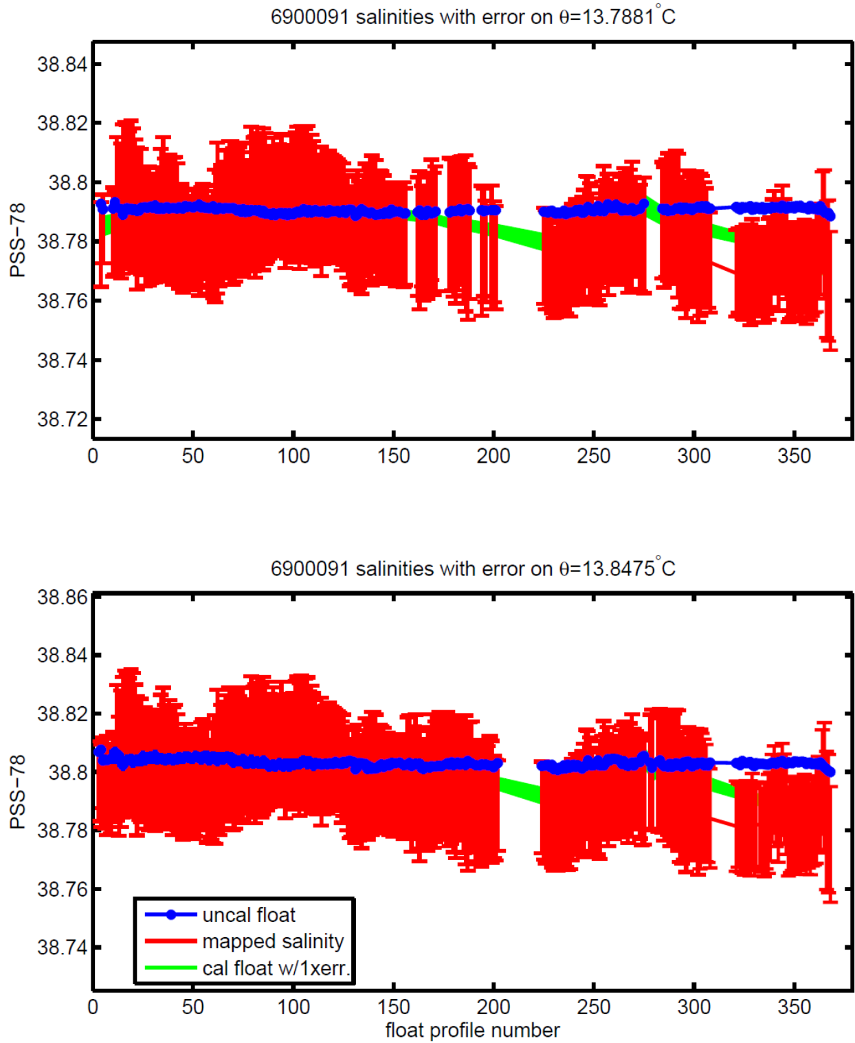
Figure 12. Comparison between the float SAL_RC data and the mapped salinity, on \theta -levels.
