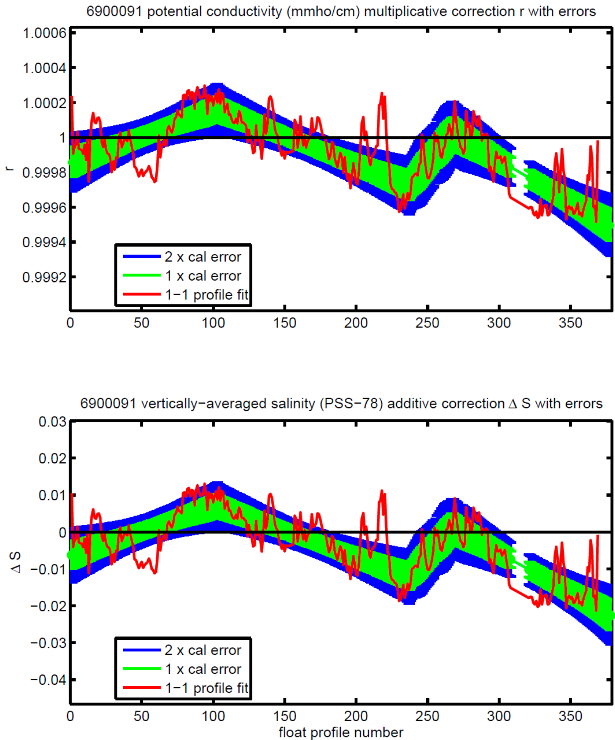
Figure 14. Correction proposed by the OW method.
