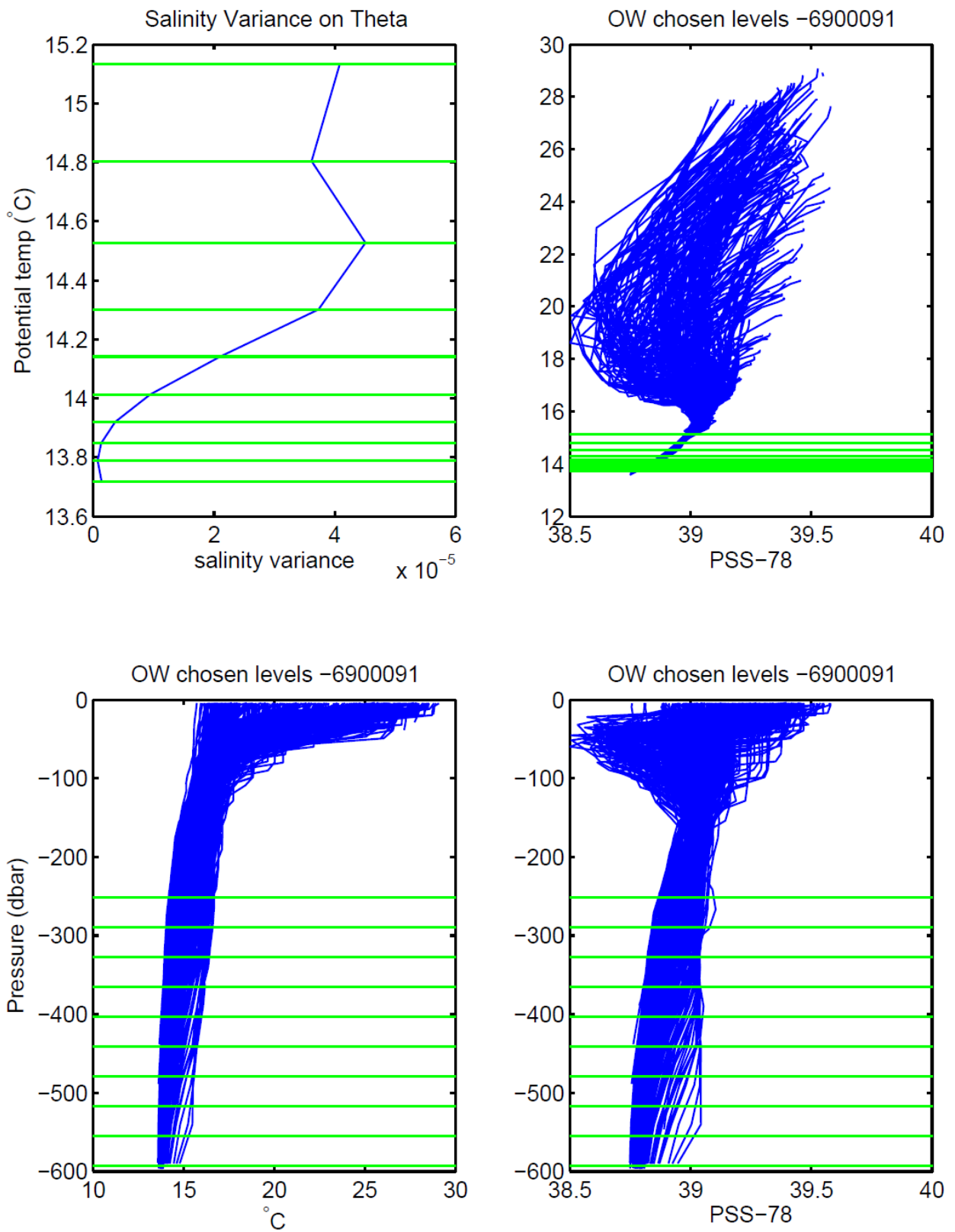
Figure 11. The 10 \theta -levels chosen for the correction.
