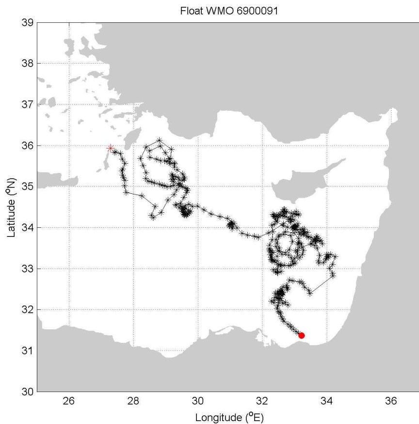
Figure 1. Float trajectory (the red asterisk (dot) represents the first (last) float position).
