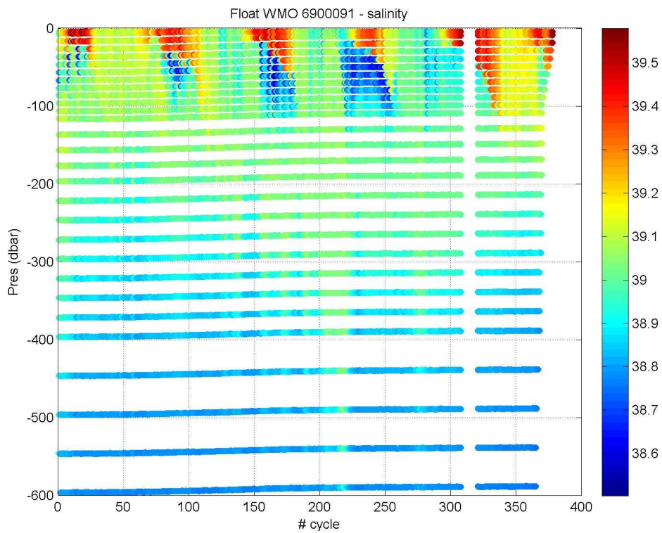
Figure 2. SAL_RC section along the float trajectory.
