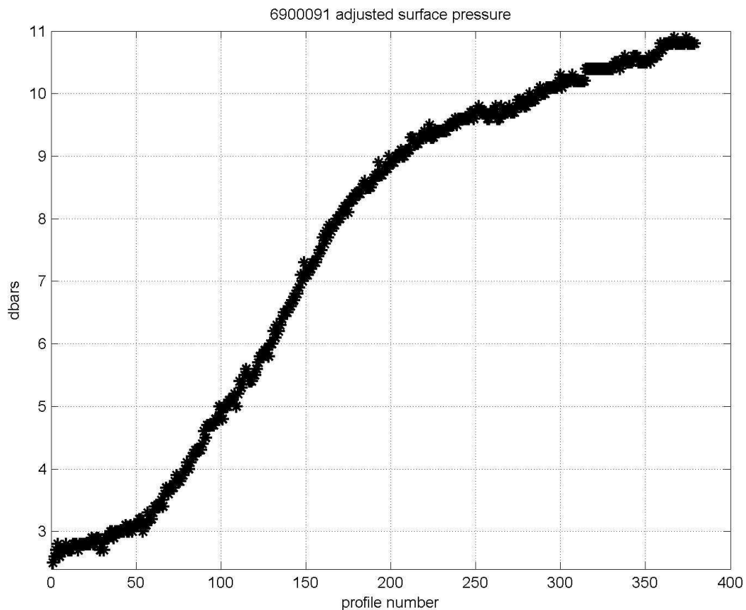
Figure 4. Adjusted surface pressure values versus time.
