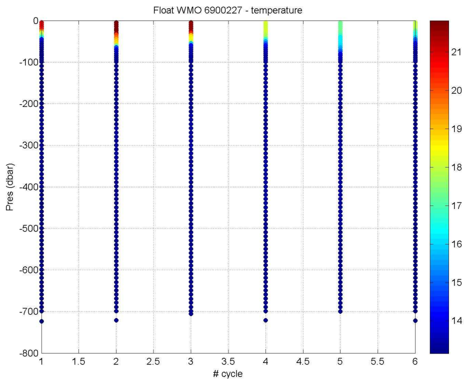
Figure 3. Temperature (° C) section along the float trajectory.
