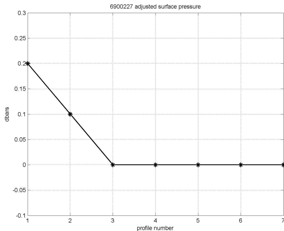
Figure 4. Surface pressure values versus time.
