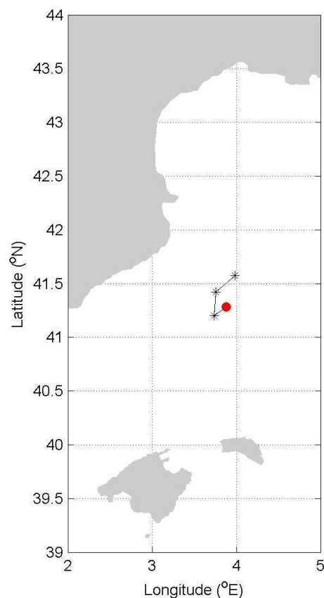
Figure 1. Float trajectory (the red dot represents the last float position).
