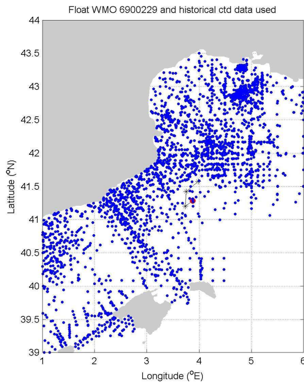
Figure 8. Float trajectory (black line; the last float position is depicted by a red dot) and locations of the historical CTD data.
