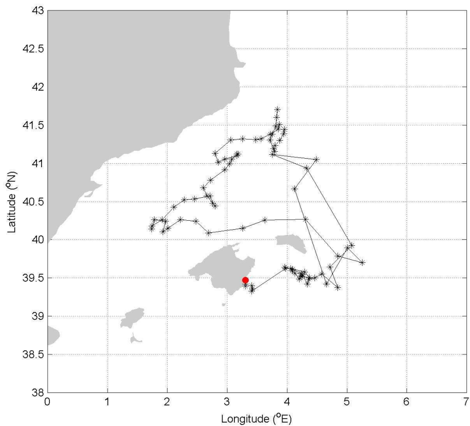
Figure 1. Float trajectory (the red dot represents the last float position).
