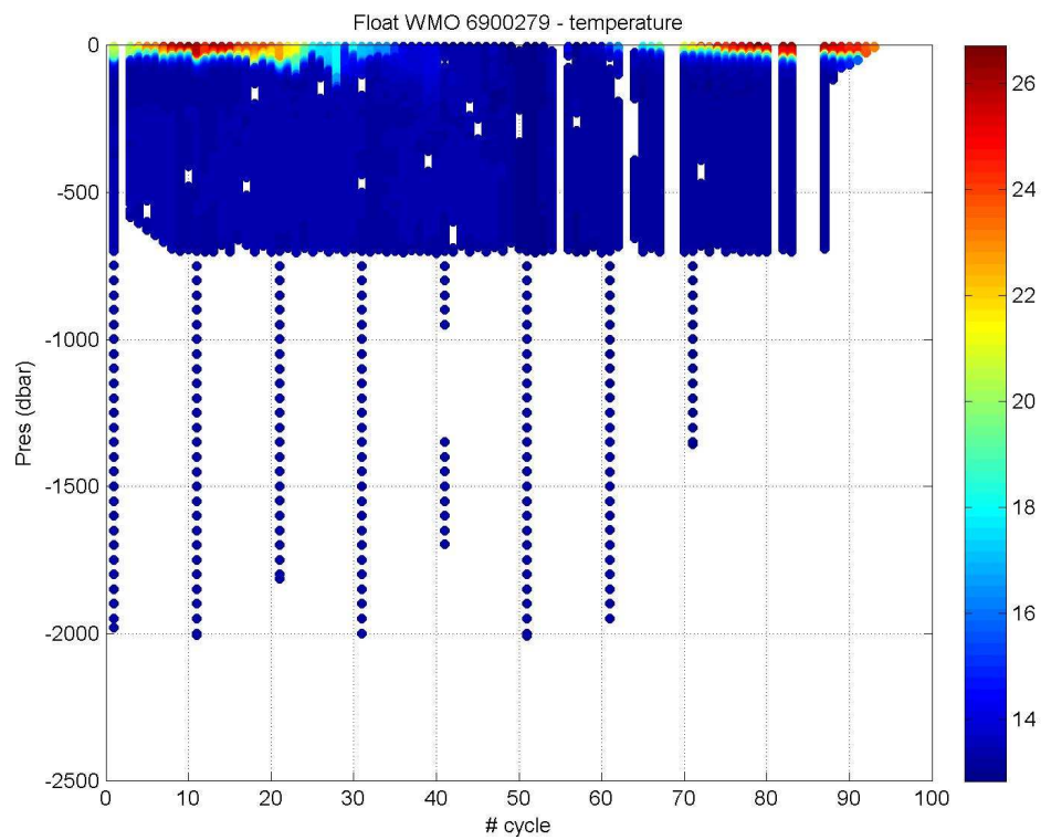
Figure 3. Temperature (° C) section along the float trajectory.
