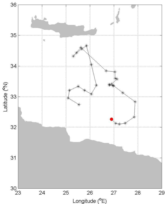
Figure 1. Float trajectory (the red dot represents the last float position).
