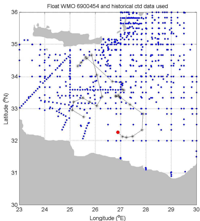
Figure 8. Float trajectory (black line; the last float position is depicted by a red dot) and locations of the historical CTD data.
