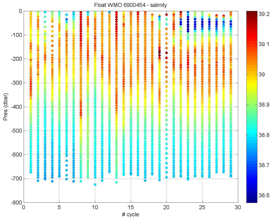
Figure 2. Salinity section along the float trajectory.
