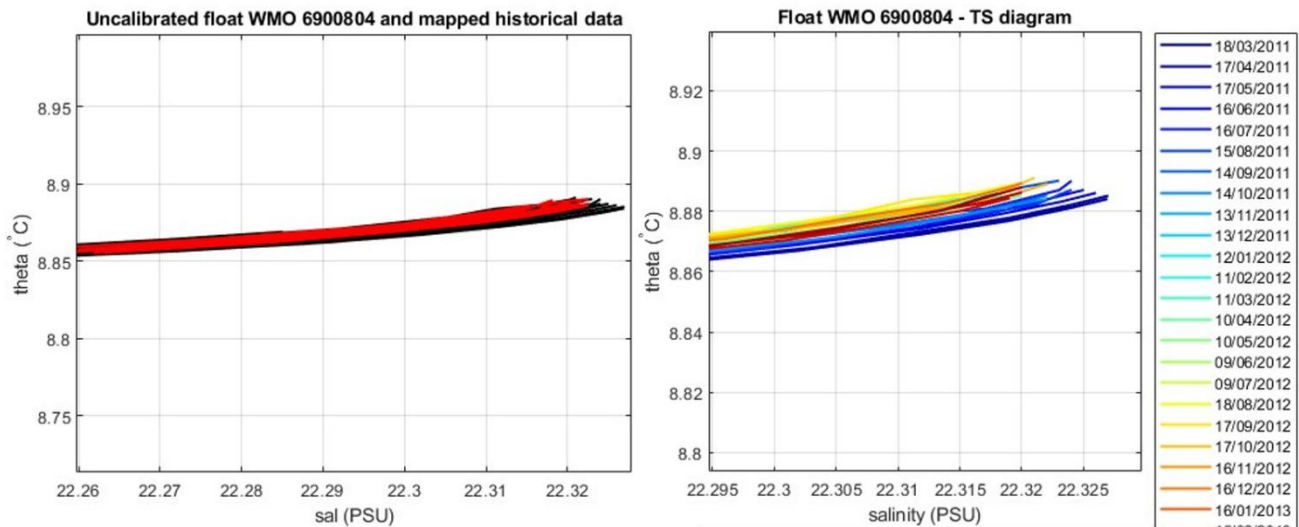
Figure 7: Comparison between float 6900804 and historical CTD on the left and \theta -S diagram color-coded per cycle number on the right, in the most uniform part of the \theta -S curve.
