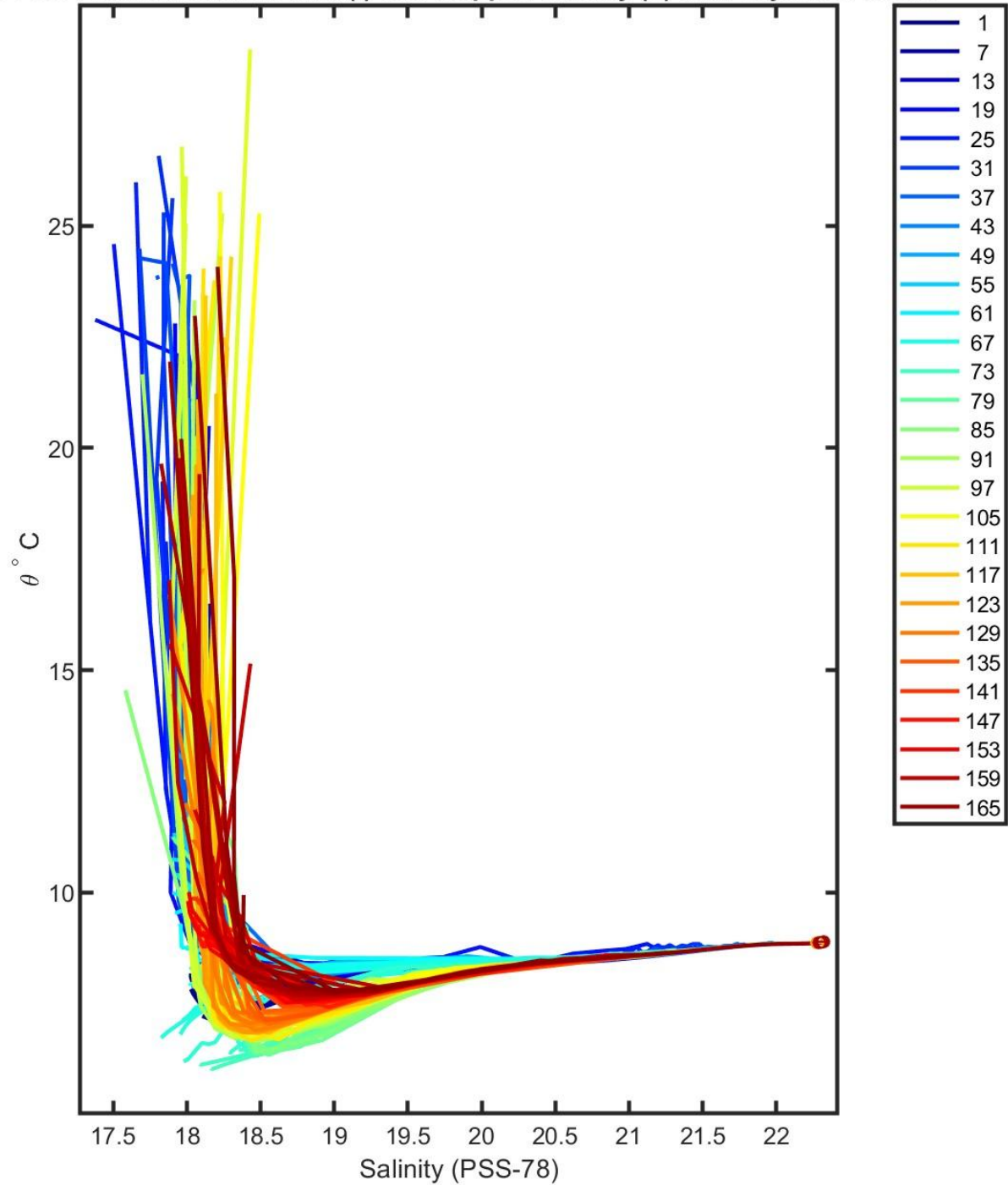
6900804 calibrated float data (-) and mapped salinity (o) with objective errors
