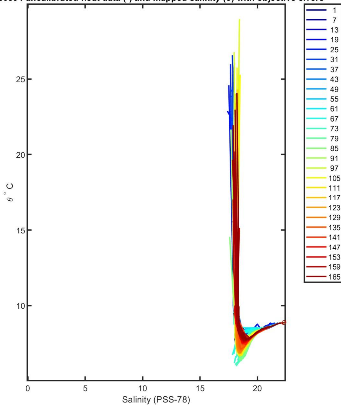
6900804 uncalibrated float data (-) and mapped salinity (o) with objective errors
