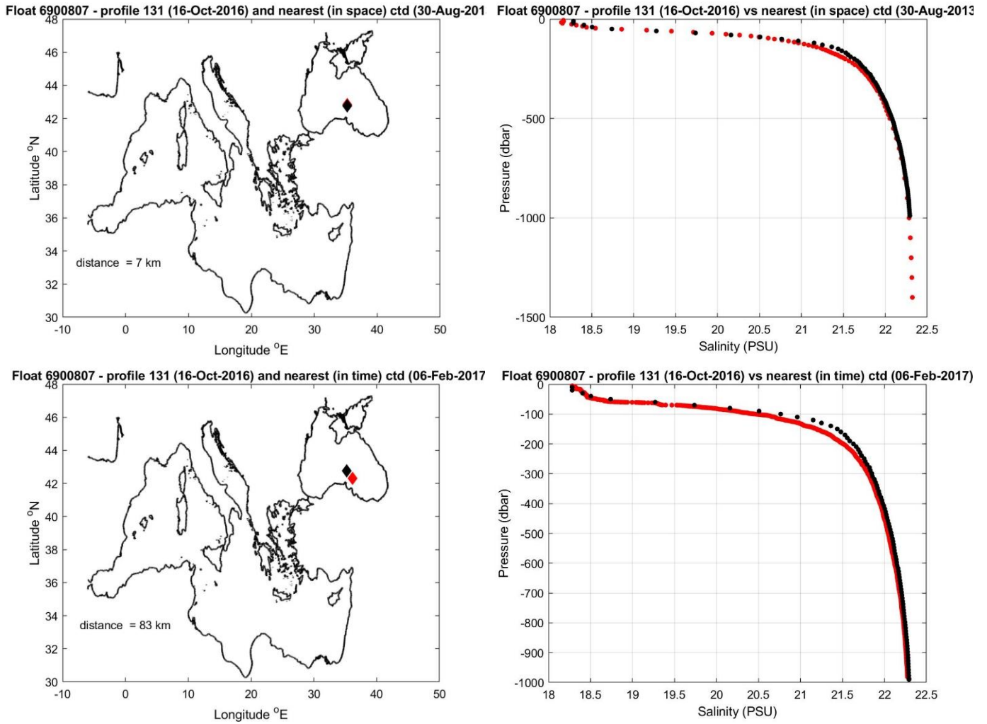
Figure 9: Float 6900807. The salinity float profile number 131 (black dots) are compared to the nearest in space (top) and in time (bottom) reference profile (red dots). The locations of the two profiles and their distance is given in the left panel.
