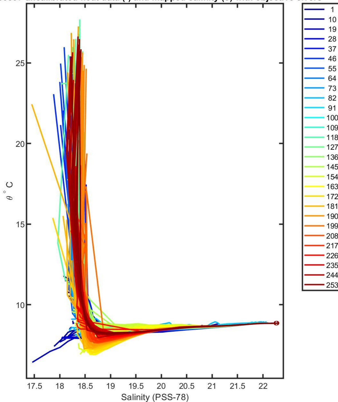
6900807 uncalibrated float data (-) and mapped salinity (o) with objective errors
