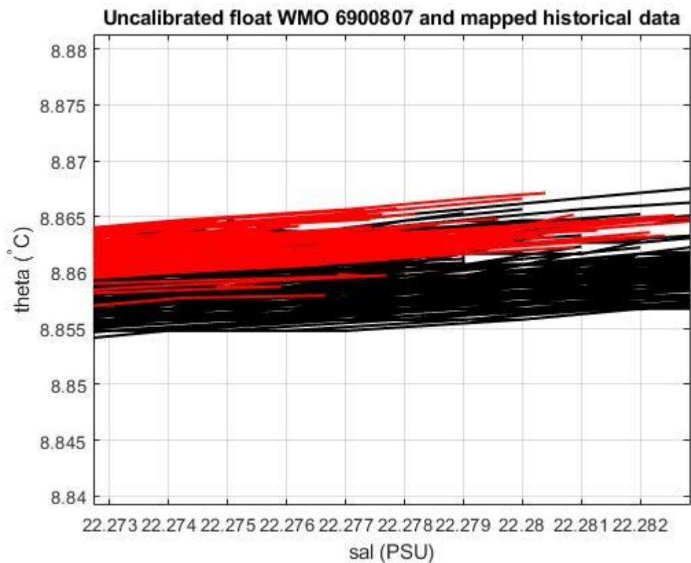
Figure 18: Float 6900807. Uncalibrated float salinity profile (black lines) and mapped historical data (red lines) in the most uniform part of the \theta -S curve.
