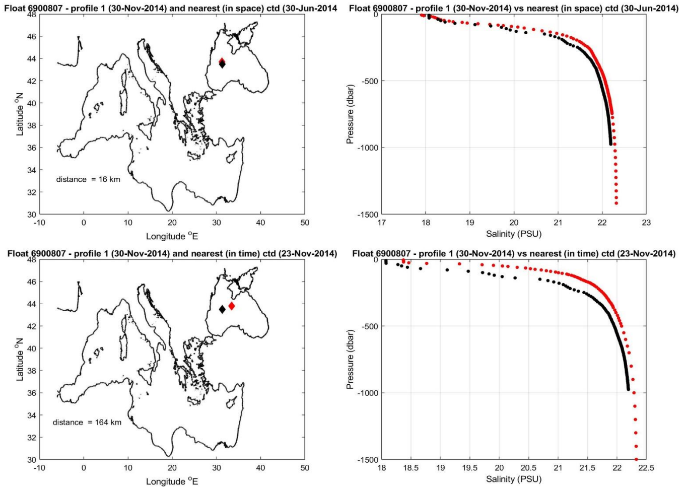
Figure 8: Float 6900807. The salinity float profile number 1 (black dots) are compared to the nearest in space (top) and in time (bottom) reference profile (red dots). The locations of the two profiles and their distance is given in the left panel.
