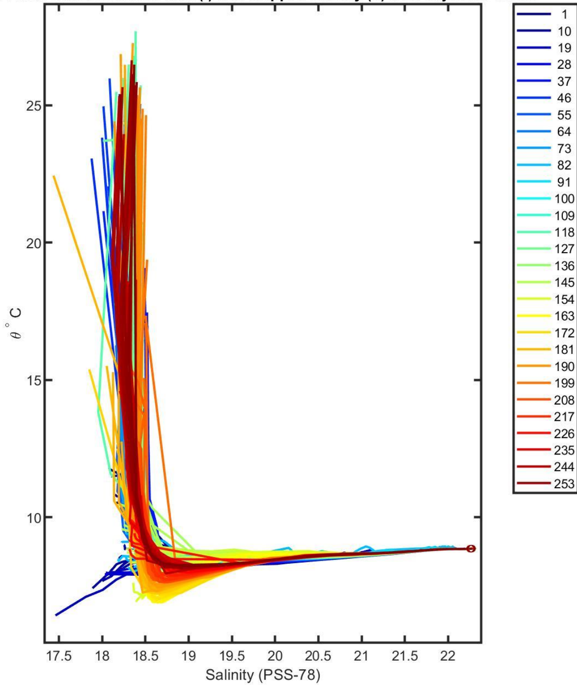
6900807 calibrated float data (-) and mapped salinity (o) with objective errors
