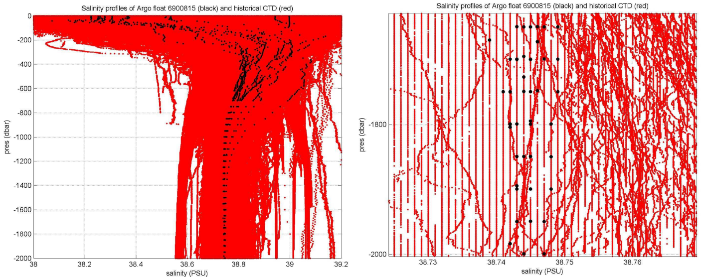
Figure 9. Salinity profiles of the Argo float (black lines) and historical CTD (red lines). A zoom of the deepest part of the float profiles is presented in the right panel.
