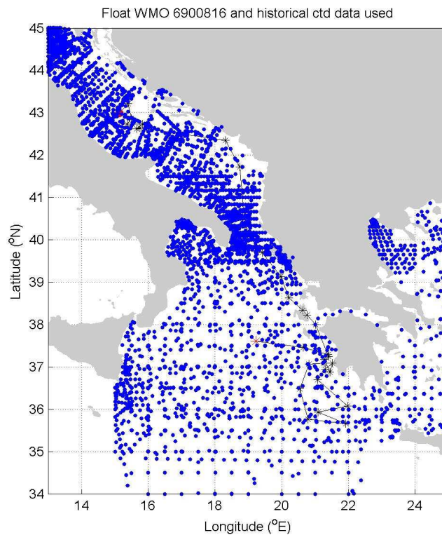
Figure 8. Float trajectory (black line; the last float position is depicted by a red dot) and locations of the historical CTD data.
