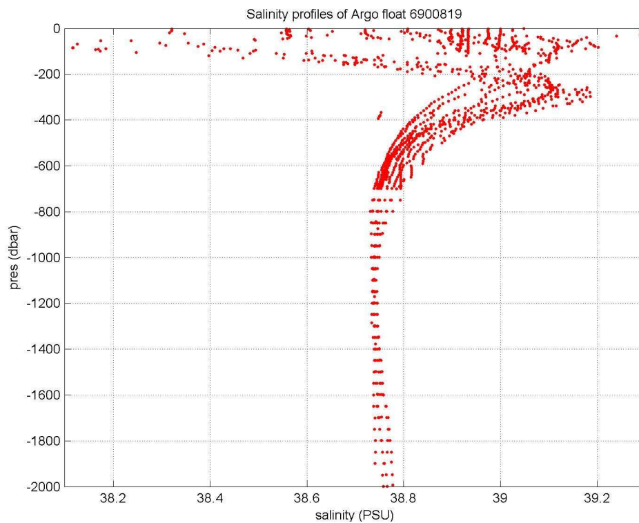
Figure 6. Salinity profiles as they are in real time correction mode at Coriolis Data Centre.
