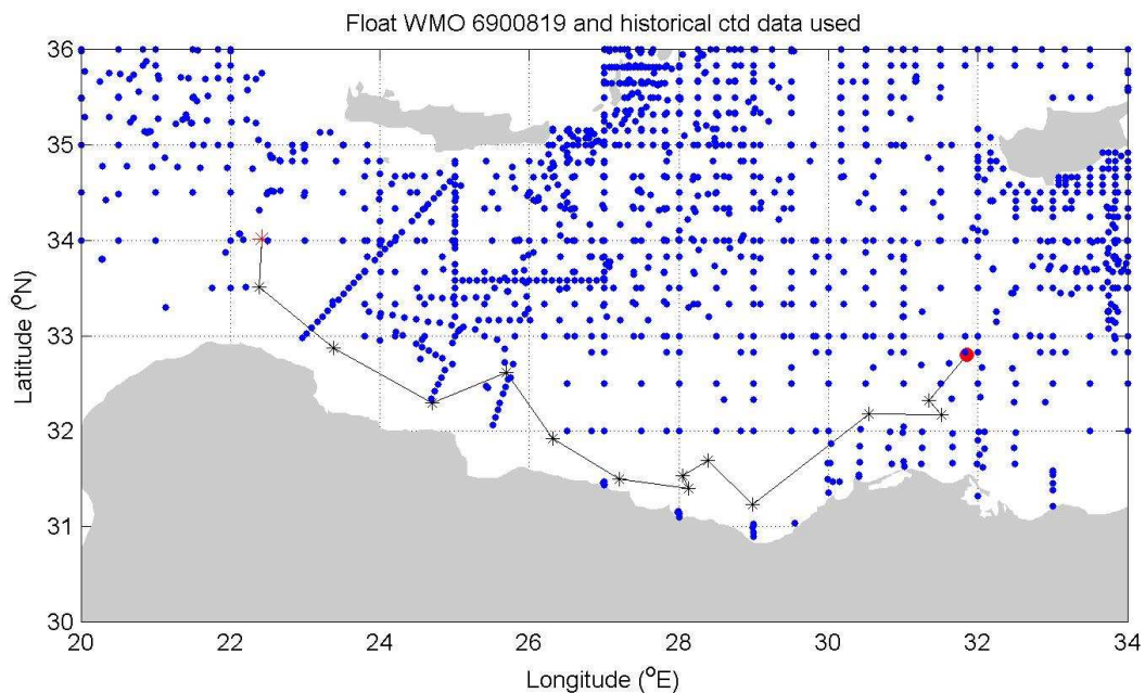
Figure 8. Float trajectory (black line; the last float position is depicted by a red dot) and locations of the historical CTD data.
