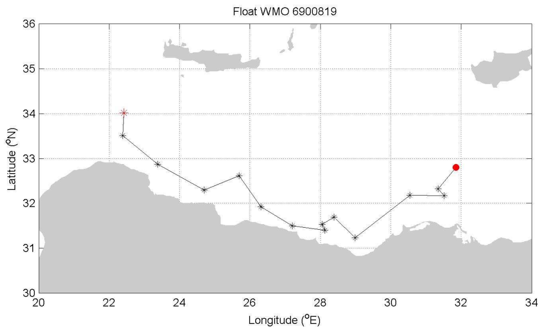
Figure 1. Float trajectory (the red dot represents the last float position).
