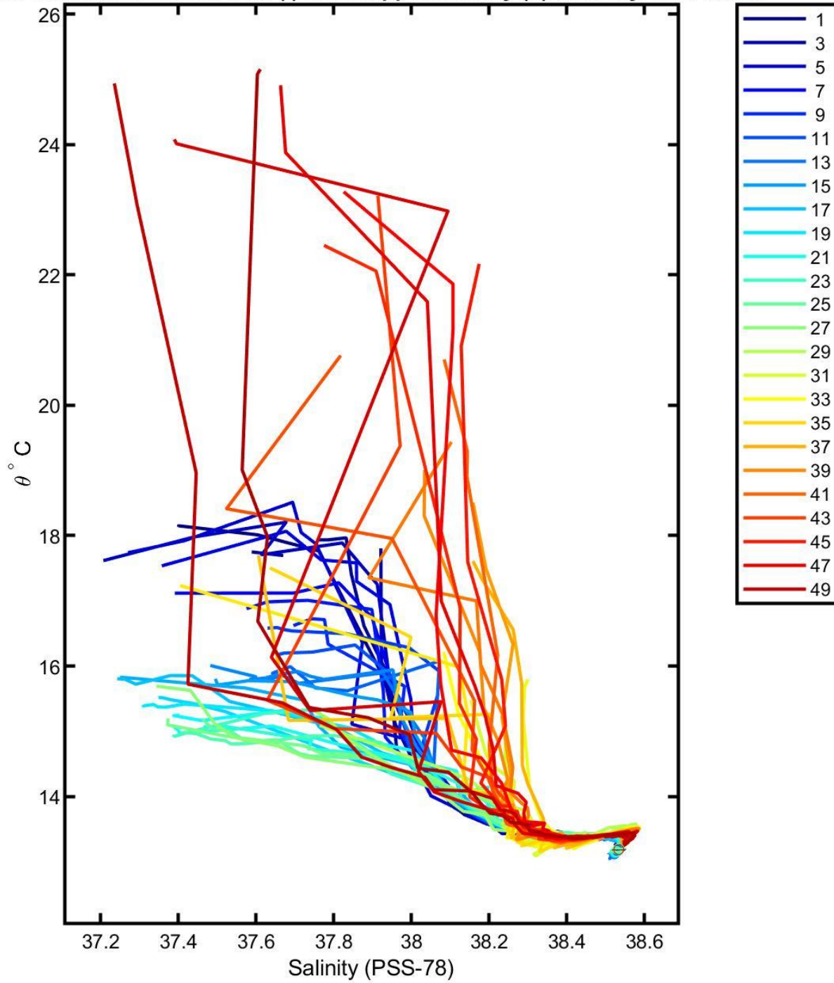
6901244 calibrated float data (-) and mapped salinity (o) with objective errors
