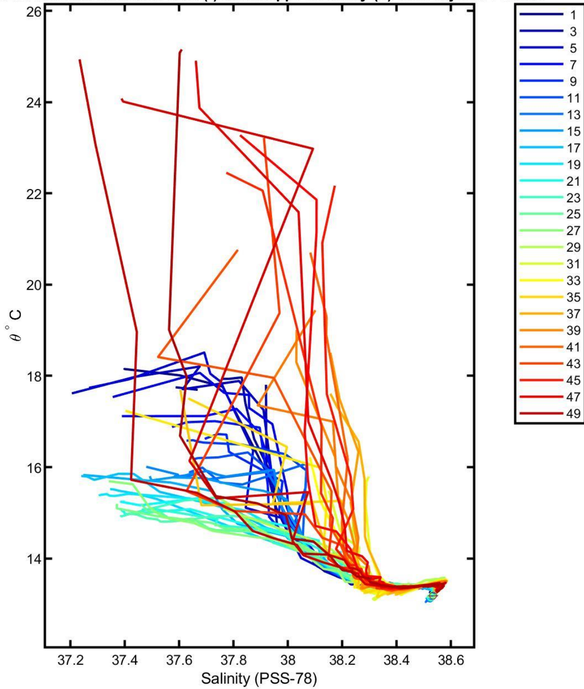
6901244 uncalibrated float data (-) and mapped salinity (o) with objective errors
