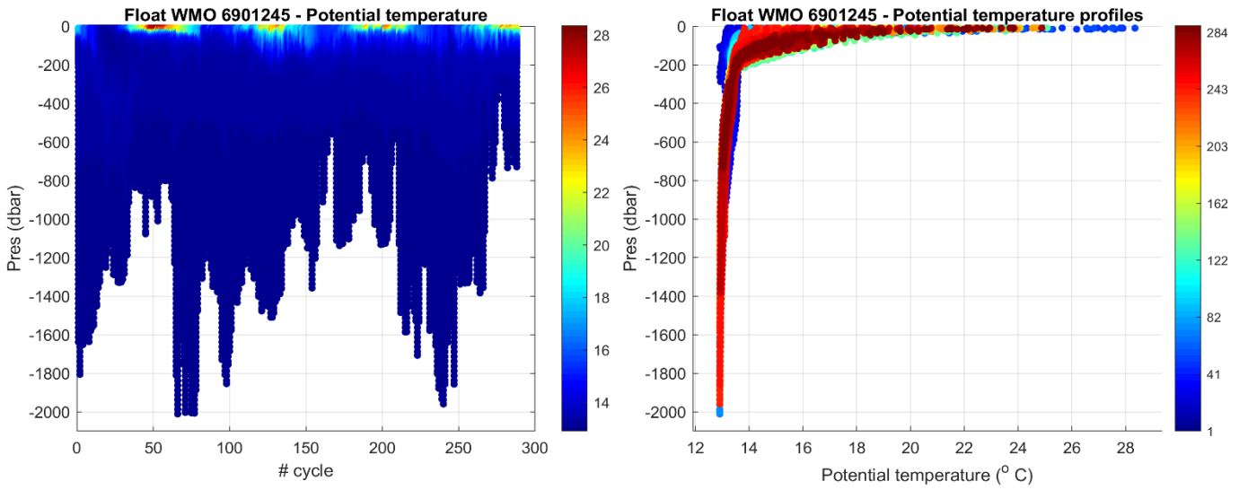
Figure 2: Float 6901245. Time series of Argo float potential temperature ( ^{\circ}\text{C} ) on the left, and potential temperature profiles color-coded per cycle number on the right.
