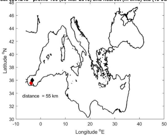
Float 6901245 - profile 100 (30-Mar-2016) and nearest (in time) ctd (19-Jun-2015)
