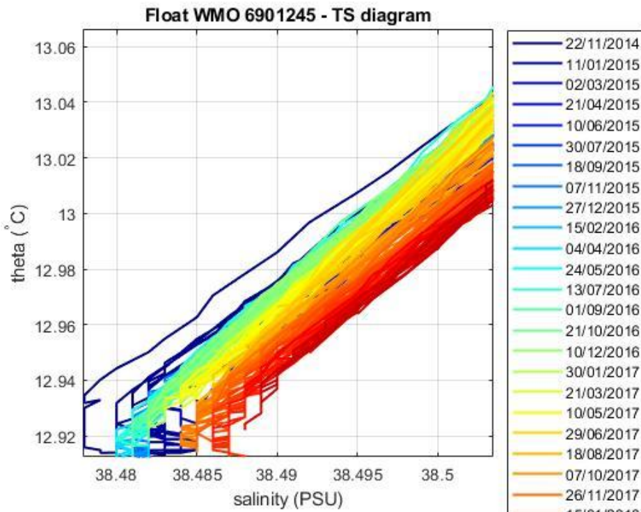
Figure 4: Float 6901245. \theta -S diagram color-coded per cycle number.
