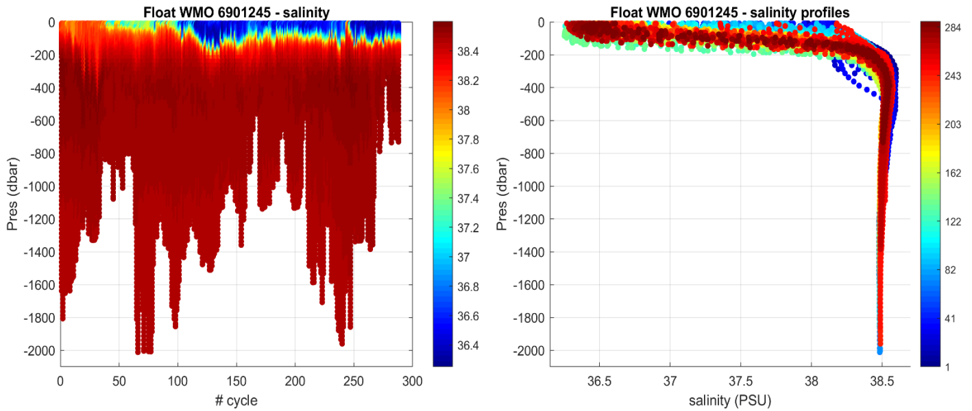
Figure 3: Float 6901245. Time series of Argo float potential salinity (PSS-78) on the left, and salinity profiles color-coded per cycle number on the right.
