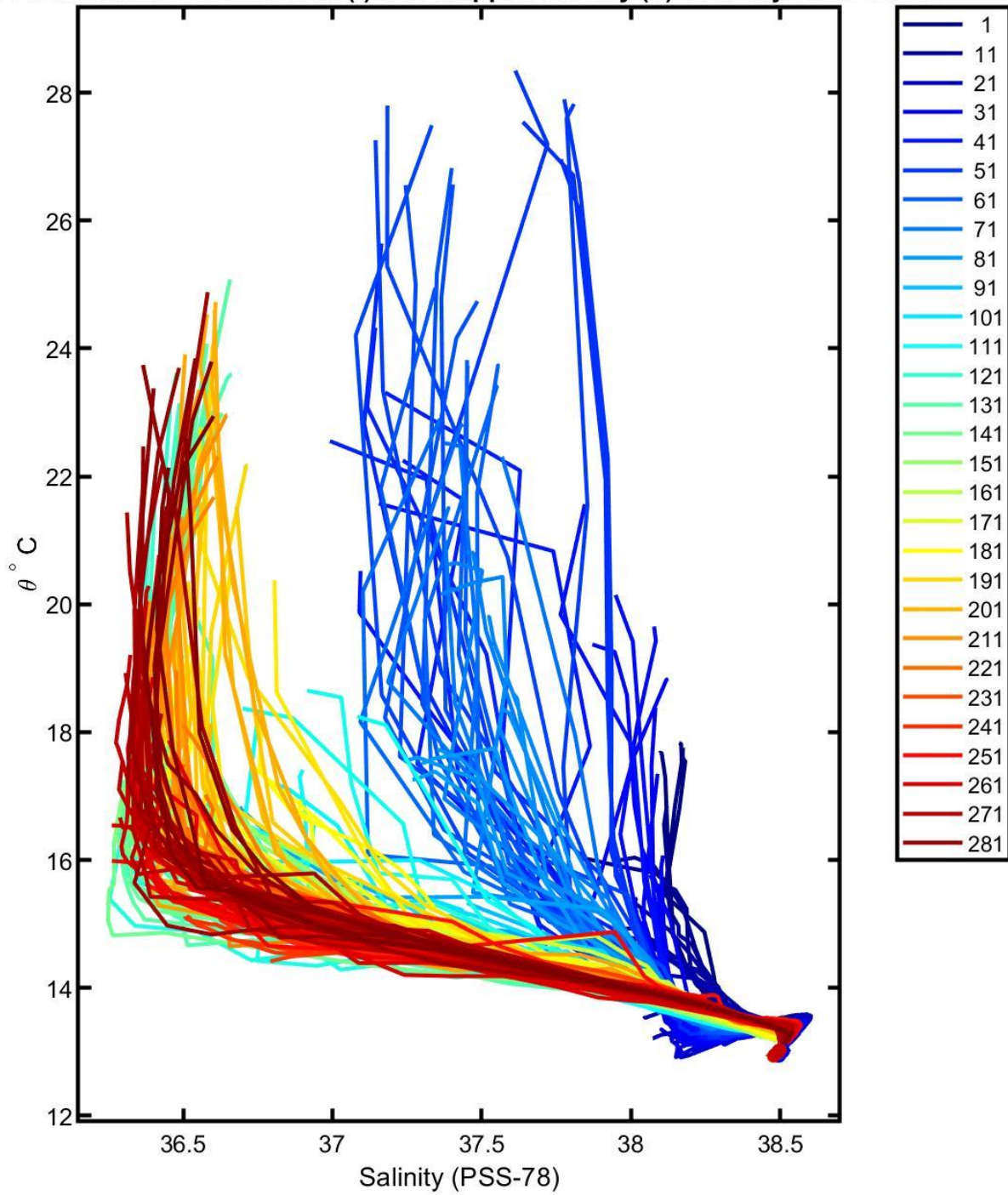
6901245 calibrated float data (-) and mapped salinity (o) with objective errors
