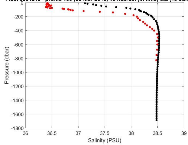
Float 6901245 - profile 100 (30-Mar-2016) vs nearest (in time) ctd (19-Jun-2015)
