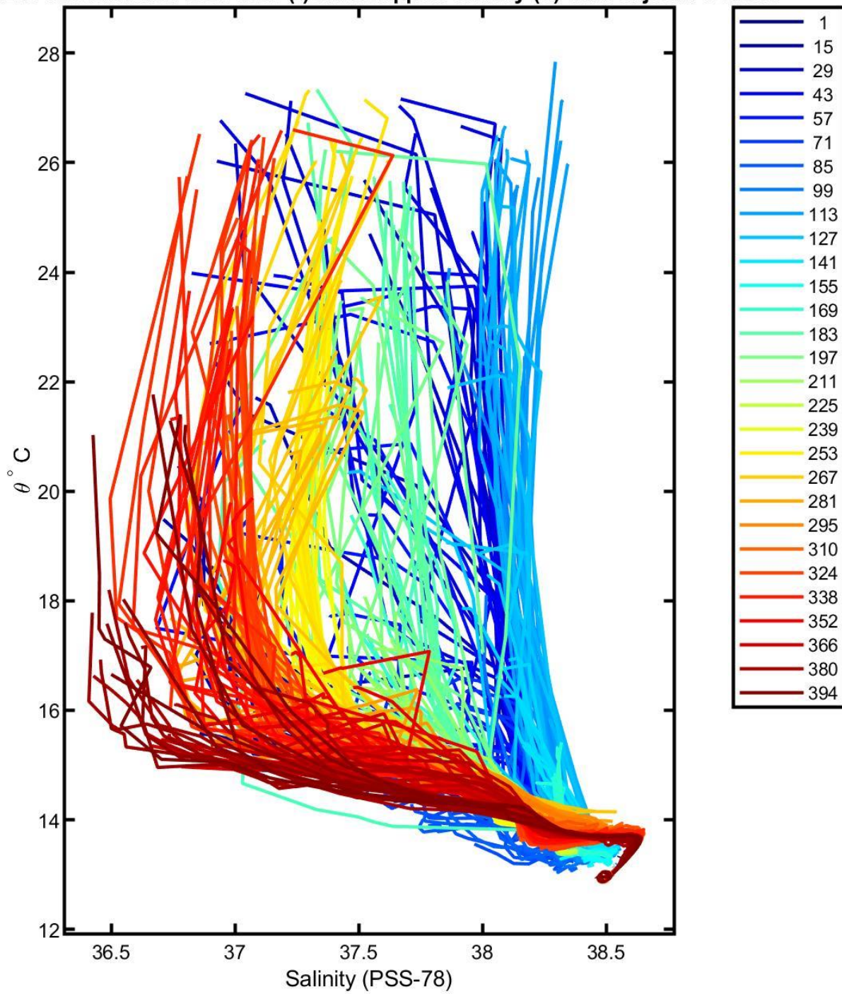
3901249 uncalibrated float data (-) and mapped salinity (o) with objective errors
