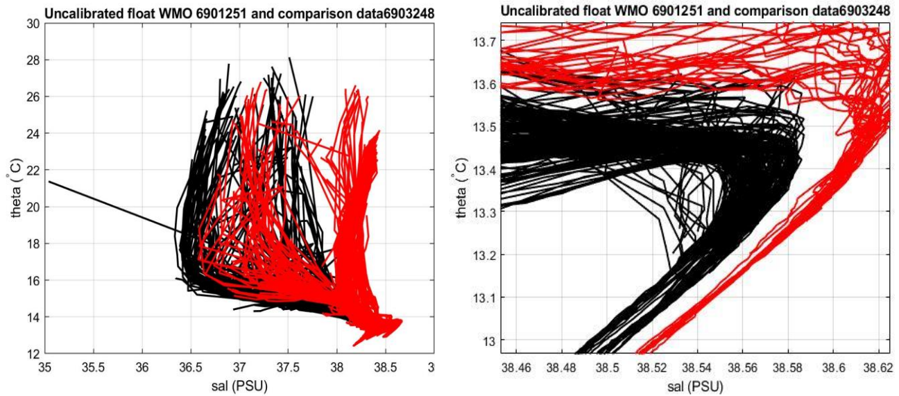
Figure 21: Float 6901251. Comparison between float 6901251 (black line) and float 6903248 (red line), on the left. On the right zoom in the most uniform part of the \theta -S curve and only for cycles from 269 to 300 (Catalan and Algerian sub basins).
