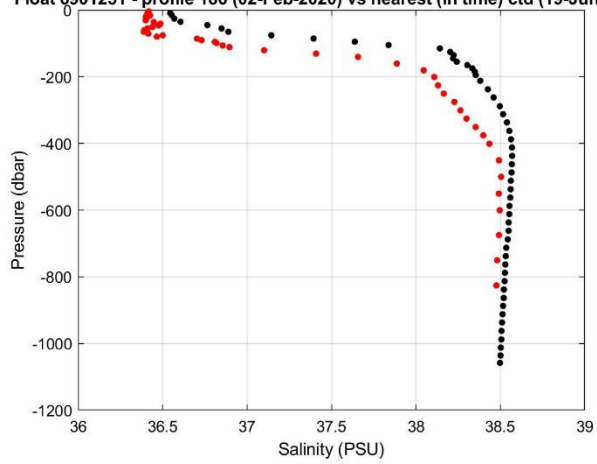
Float 6901251 - profile 186 (02-Feb-2020) vs nearest (in time) ctd (19-Jun-2015)
