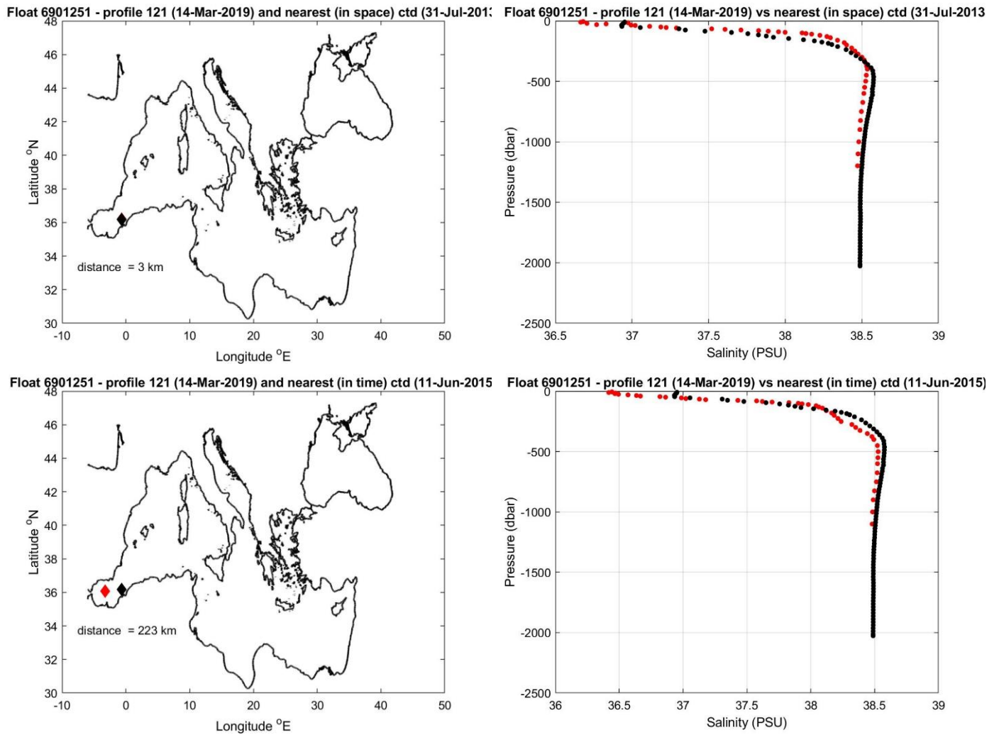
Figure 10: Float 6901251. The salinity float profile number 121 (black dots) are compared to the nearest in space (top) and in time (bottom) reference profile (red dots). The locations of the two profiles and their distance is given in the left panel.
