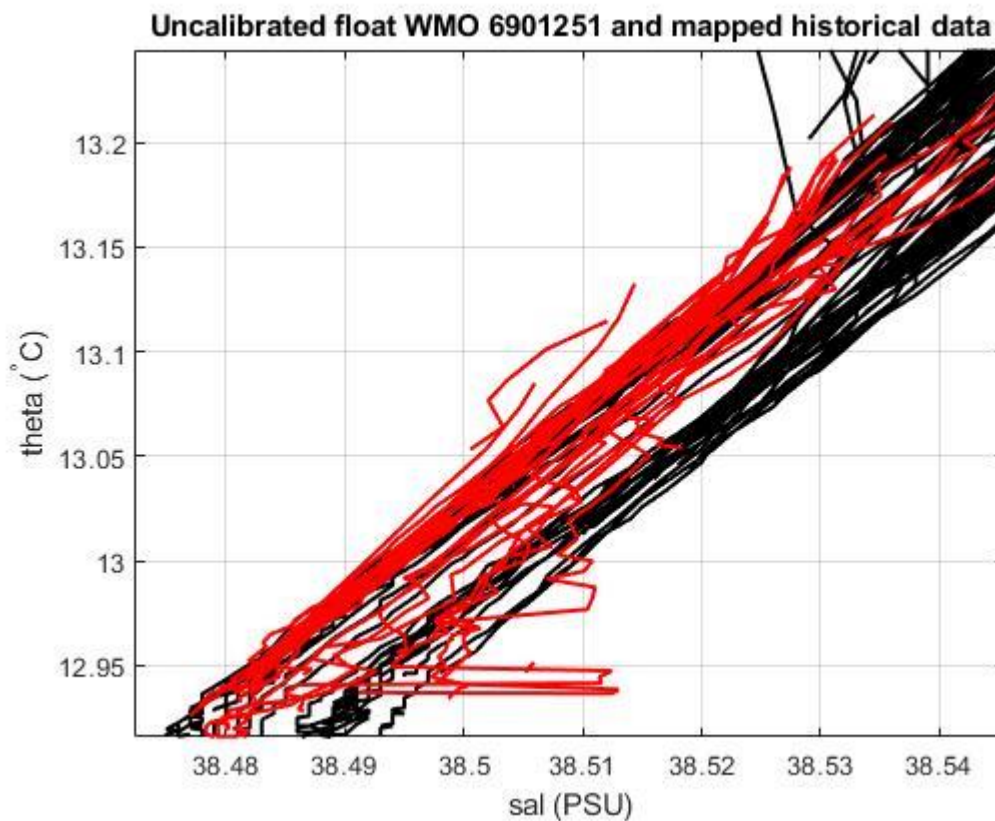
Figure 19: Float 6901251. Uncalibrated float salinity profile (black lines) and mapped historical data (red lines) in the most uniform part of the \theta -S curve.
