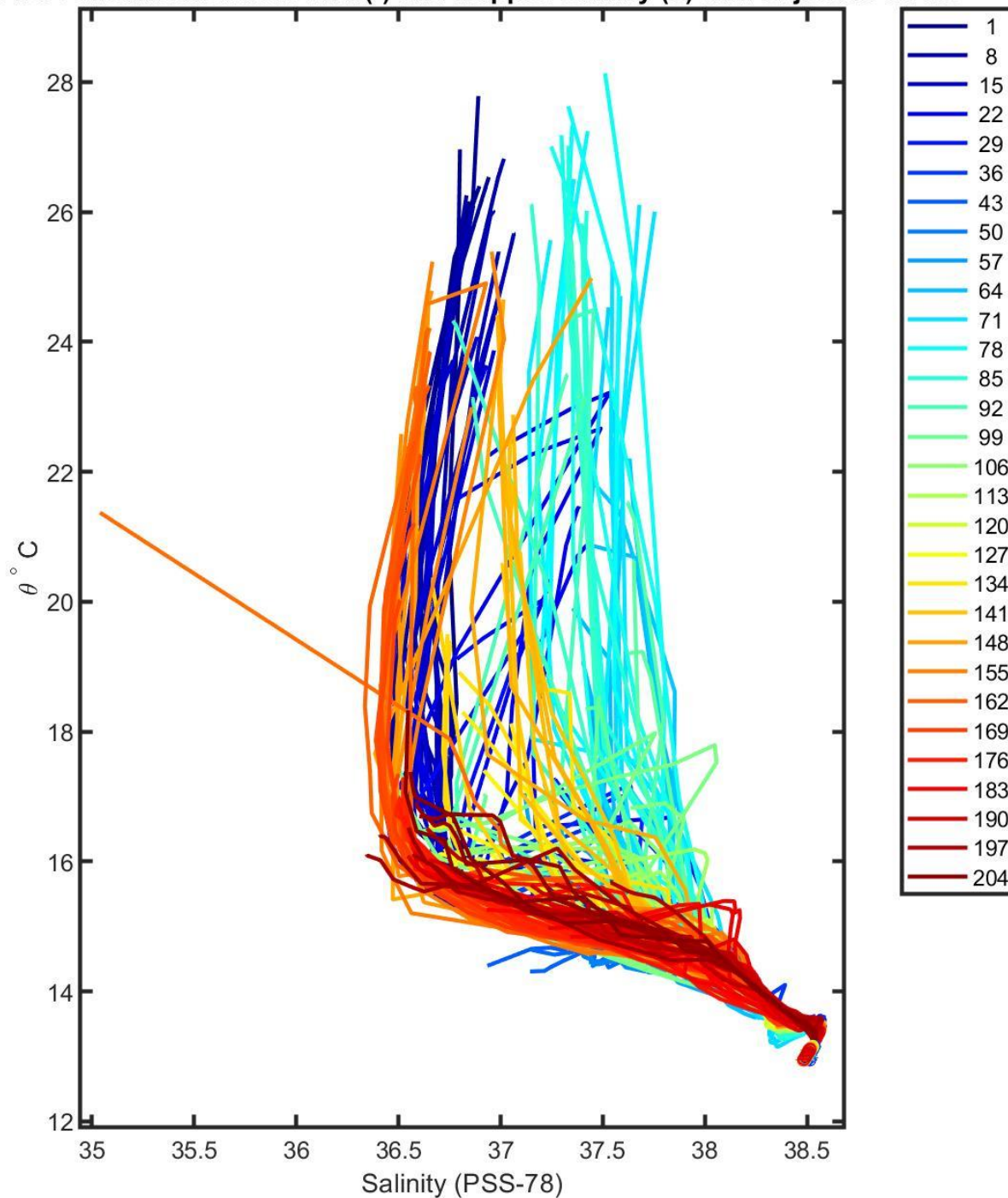
6901251 uncalibrated float data (-) and mapped salinity (o) with objective errors
