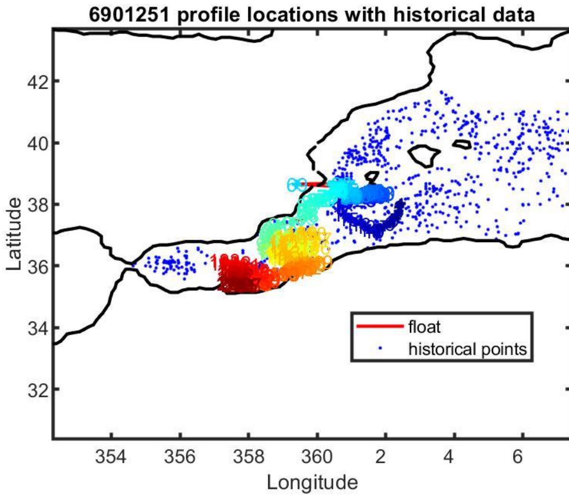
Figure 13: Float 6901251. Location of the float profiles (red line with colored numbers) and the reference data selected for mapping (blue dots).
