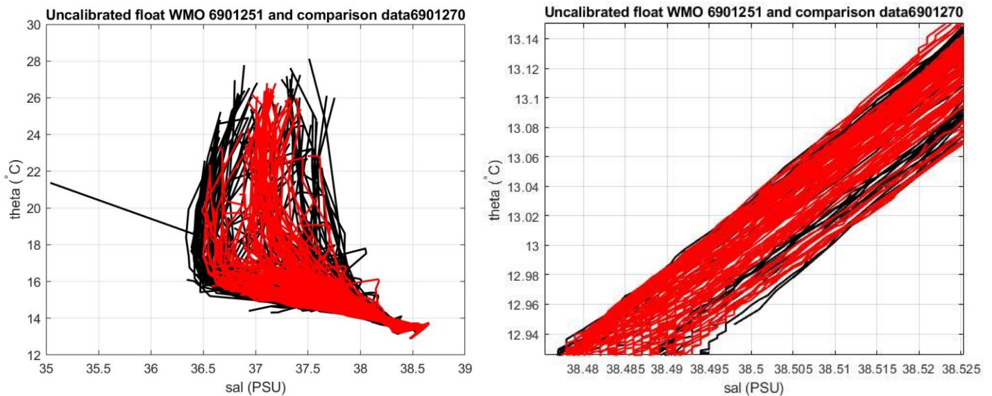
Figure 22: Float 6901251. Comparison between float 6901251 (black line) and float 6901270 (red line), on the left. On the right zoom in the most uniform part of the \theta -S curve.
