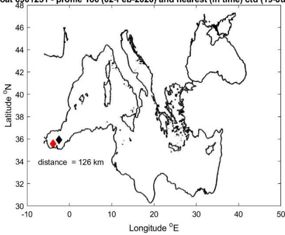
Float 6901251 - profile 186 (02-Feb-2020) and nearest (in time) ctd (19-Jun-2015)
