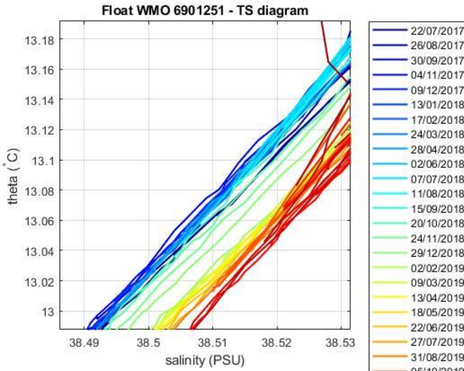
Figure 4: Float 6901251. \theta -S diagram color-coded per cycle number.
