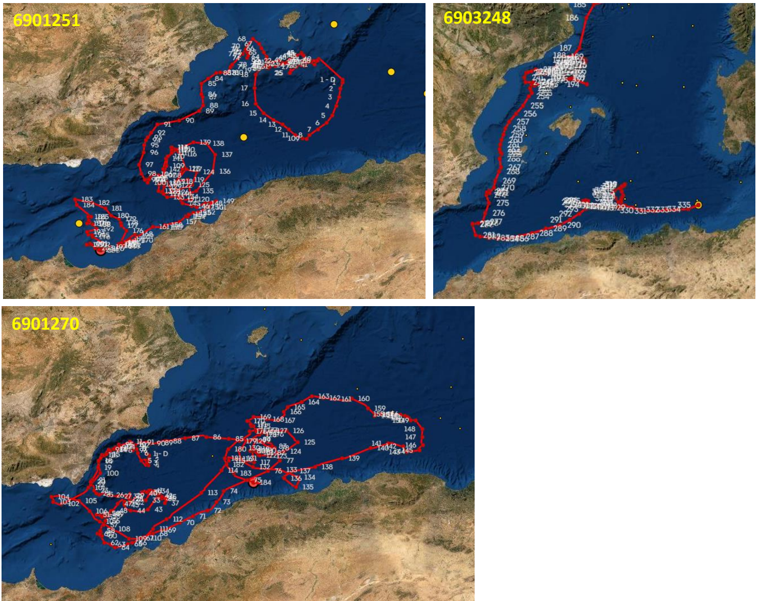
Figure 20: Float 6901251. Trajectory of the floats used for the comparison.
