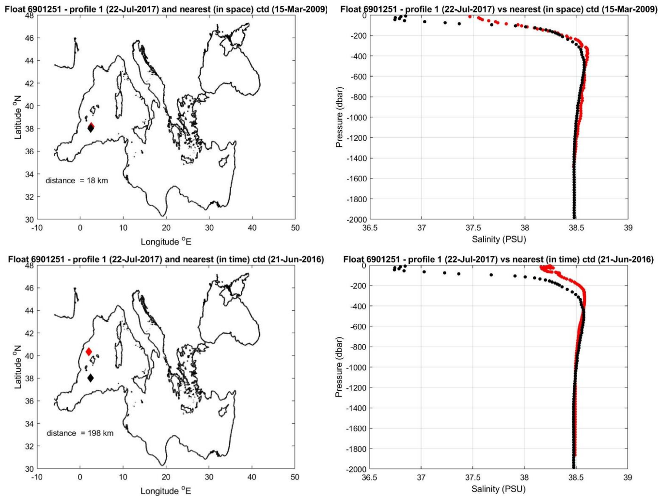
Figure 9: Float 6901251. The salinity float profile number 1 (black dots) are compared to the nearest in space (top) and in time (bottom) reference profile (red dots). The locations of the two profiles and their distance is given in the left panel.
