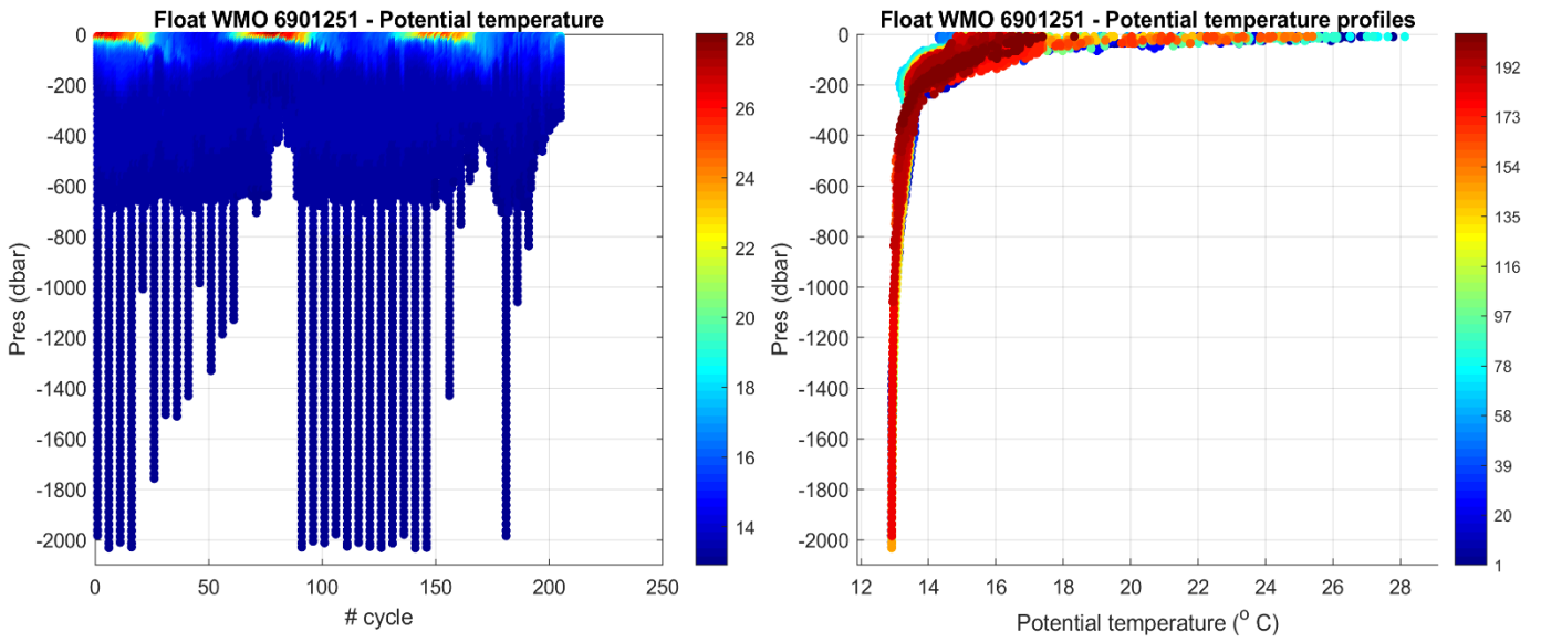
Figure 2: Float 6901251. Time series of Argo float potential temperature ( ^{\circ}\text{C} ) on the left, and potential temperature profiles color-coded per cycle number on the right.
