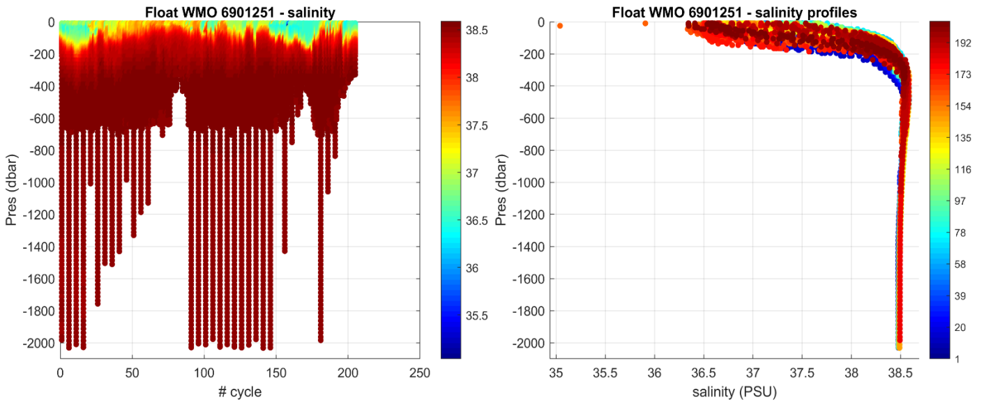
Figure 3: Float 6901251. Time series of Argo float potential salinity (PSS-78) on the left, and salinity profiles color-coded per cycle number on the right.
