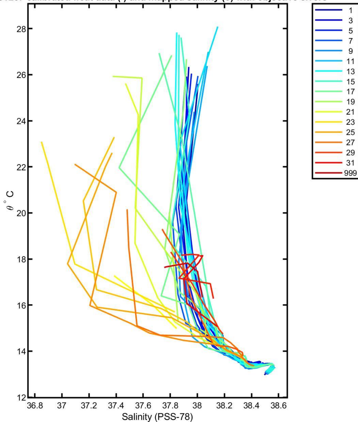
6901267 calibrated float data (-) and mapped salinity (o) with objective errors
