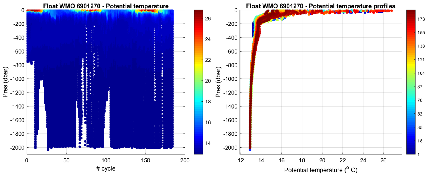
Figure 2: Float 6901270. Time series of Argo float potential temperature ( ^{\circ}\text{C} ) on the left, and potential temperature profiles color-coded per cycle number on the right.
