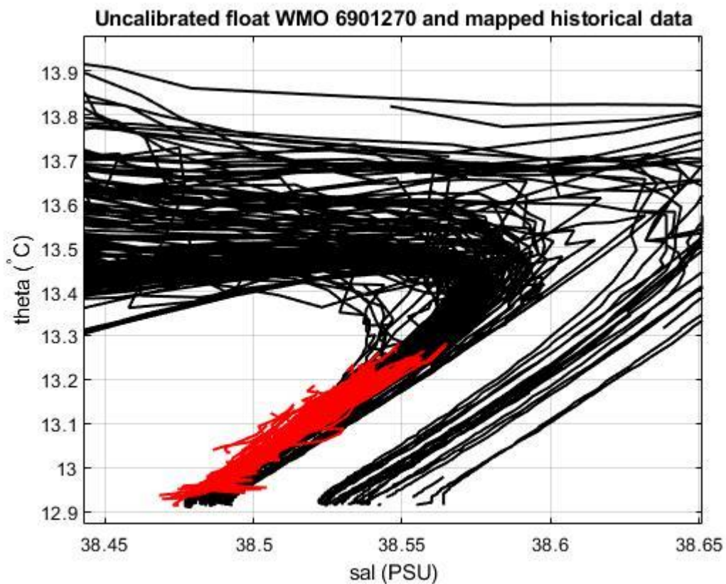
Figure 19: Float 6901270. Uncalibrated float salinity profile (black lines) and mapped historical data (red lines) in the most uniform part of the \theta -S curve.
