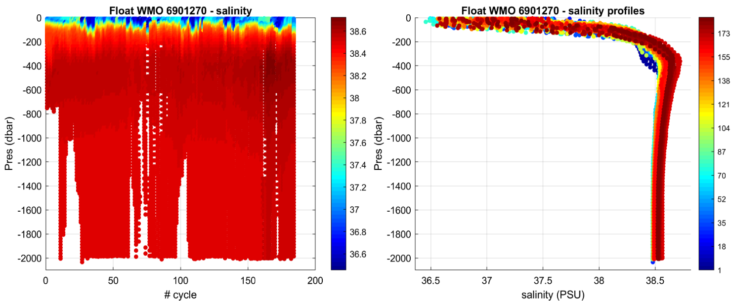
Figure 3: Float 6901270. Time series of Argo float potential salinity (PSS-78) on the left, and salinity profiles color-coded per cycle number on the right.
