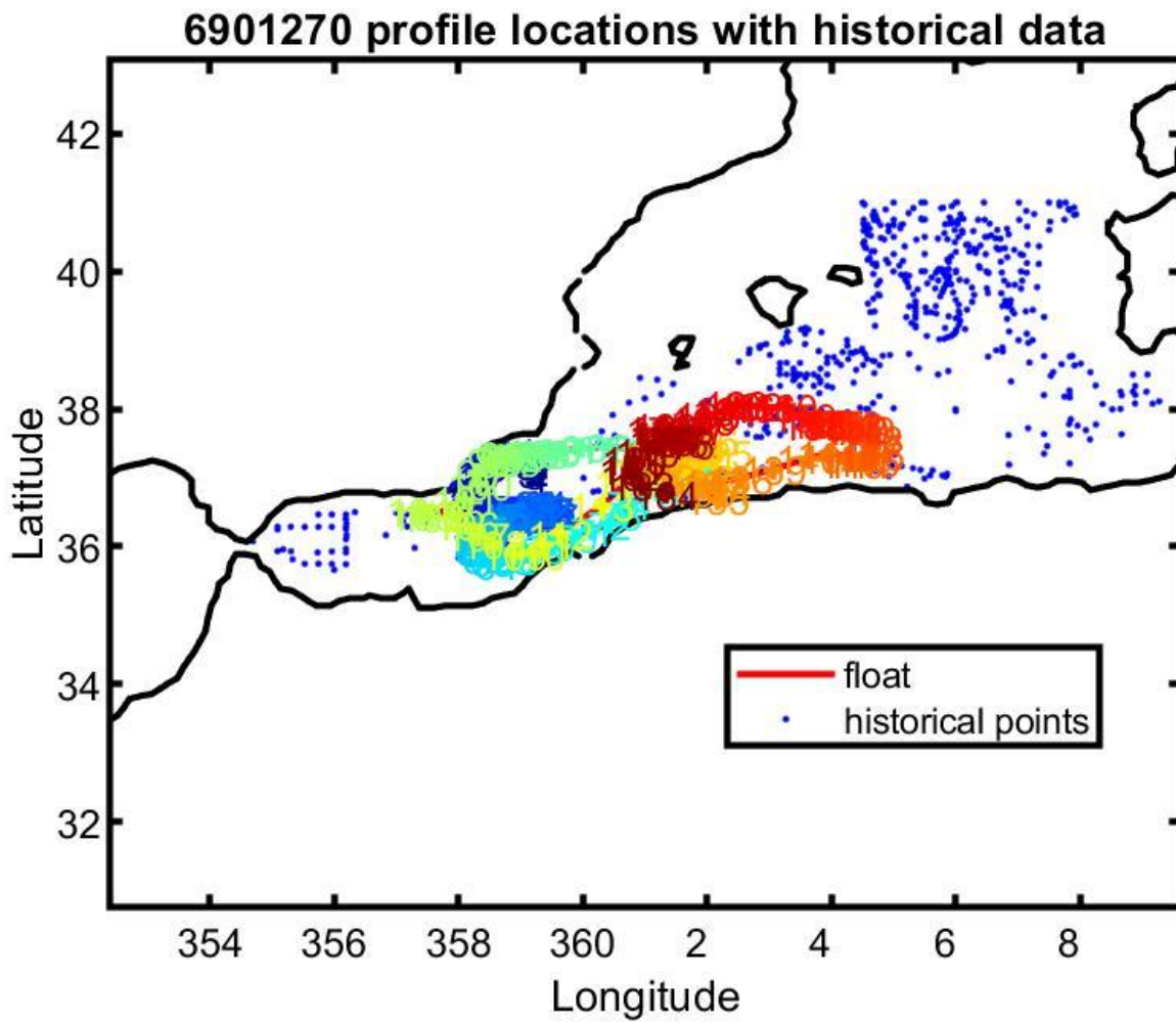
Figure 13: Float 6901270. Location of the float profiles (red line with colored numbers) and the reference data selected for mapping (blue dots).
