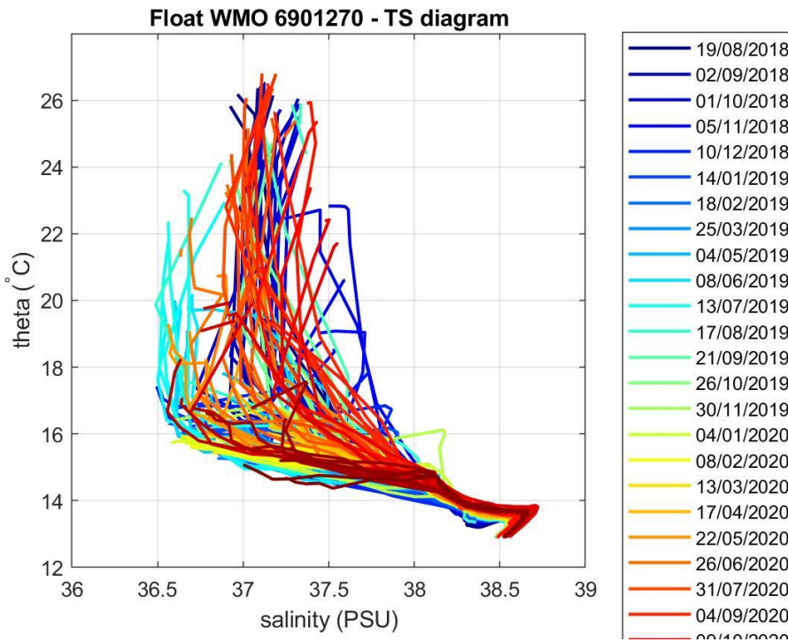
Figure 4: Float 6901270. \theta -S diagram color-coded per cycle number.
