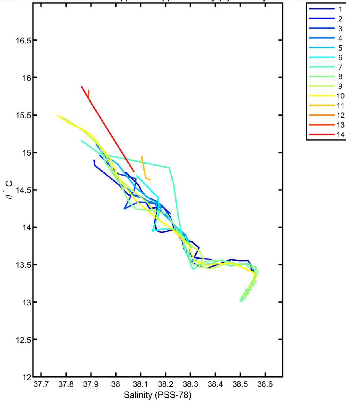
6901275 calibrated float data (-) and mapped salinity (o) with objective errors
