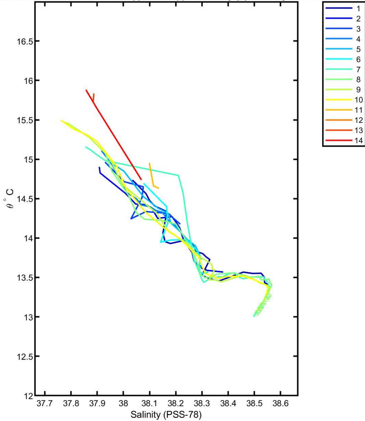
6901275 uncalibrated float data (-) and mapped salinity (o) with objective errors
