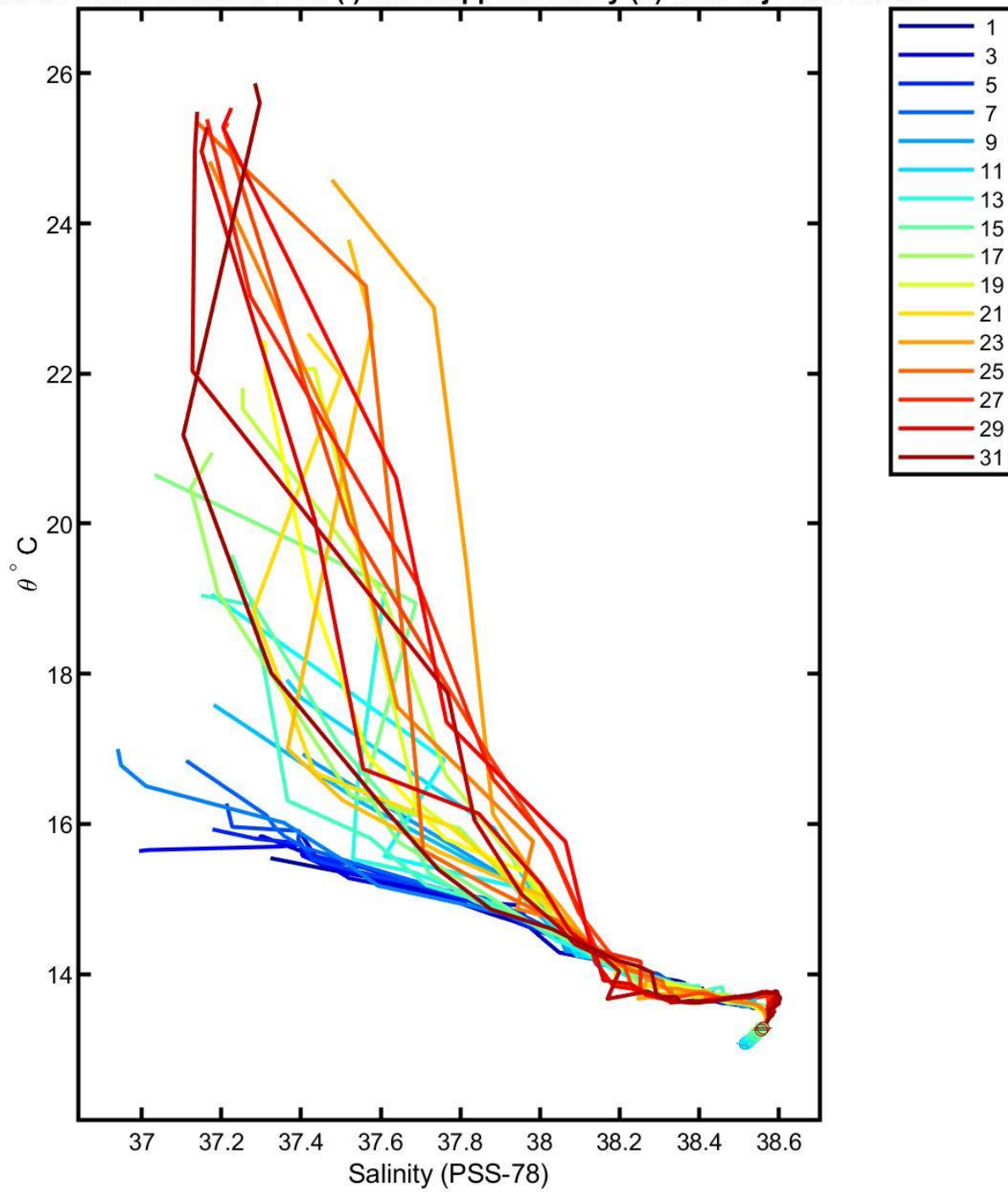
6901279 calibrated float data (-) and mapped salinity (o) with objective errors
