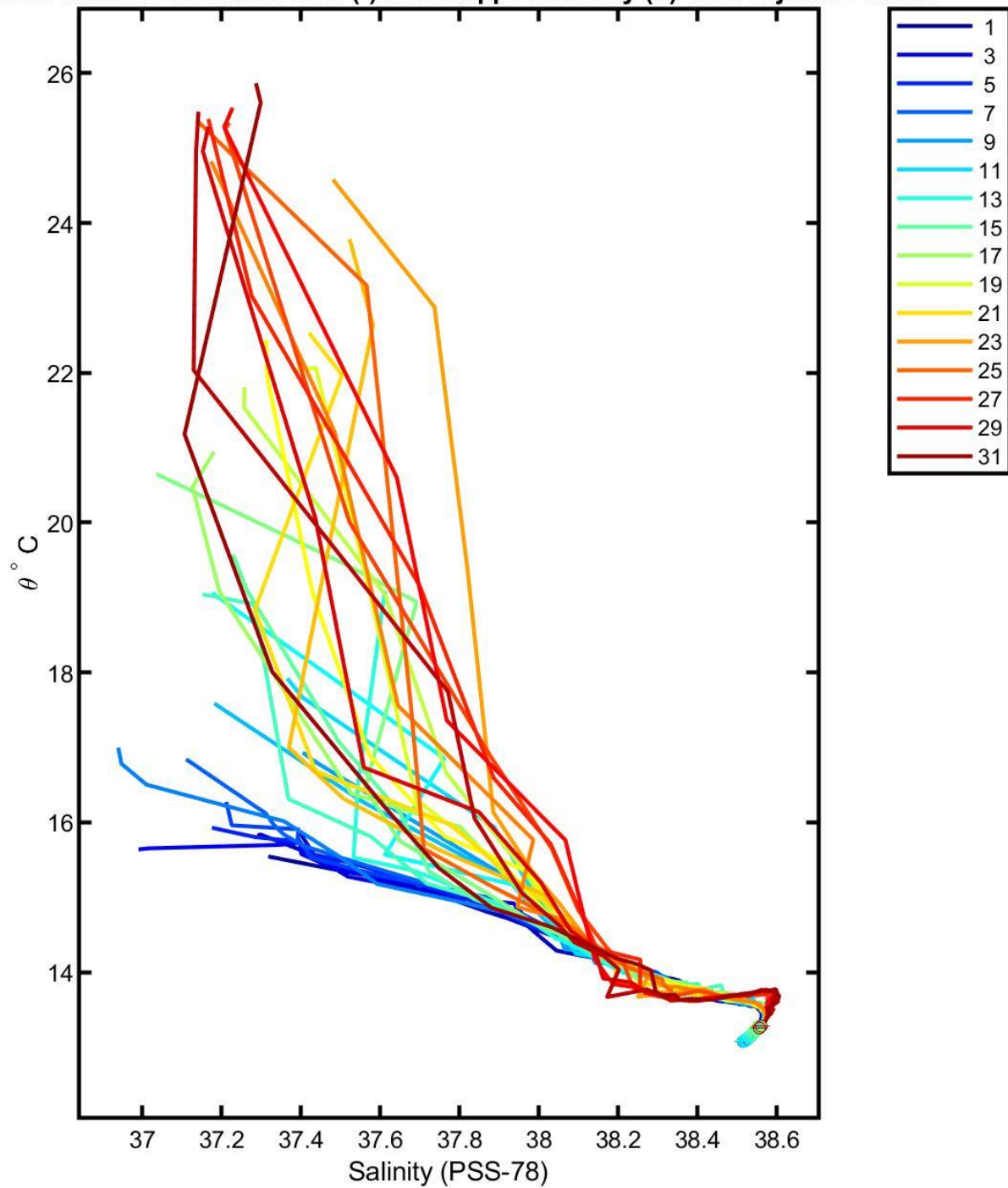
6901279 uncalibrated float data (-) and mapped salinity (o) with objective errors
