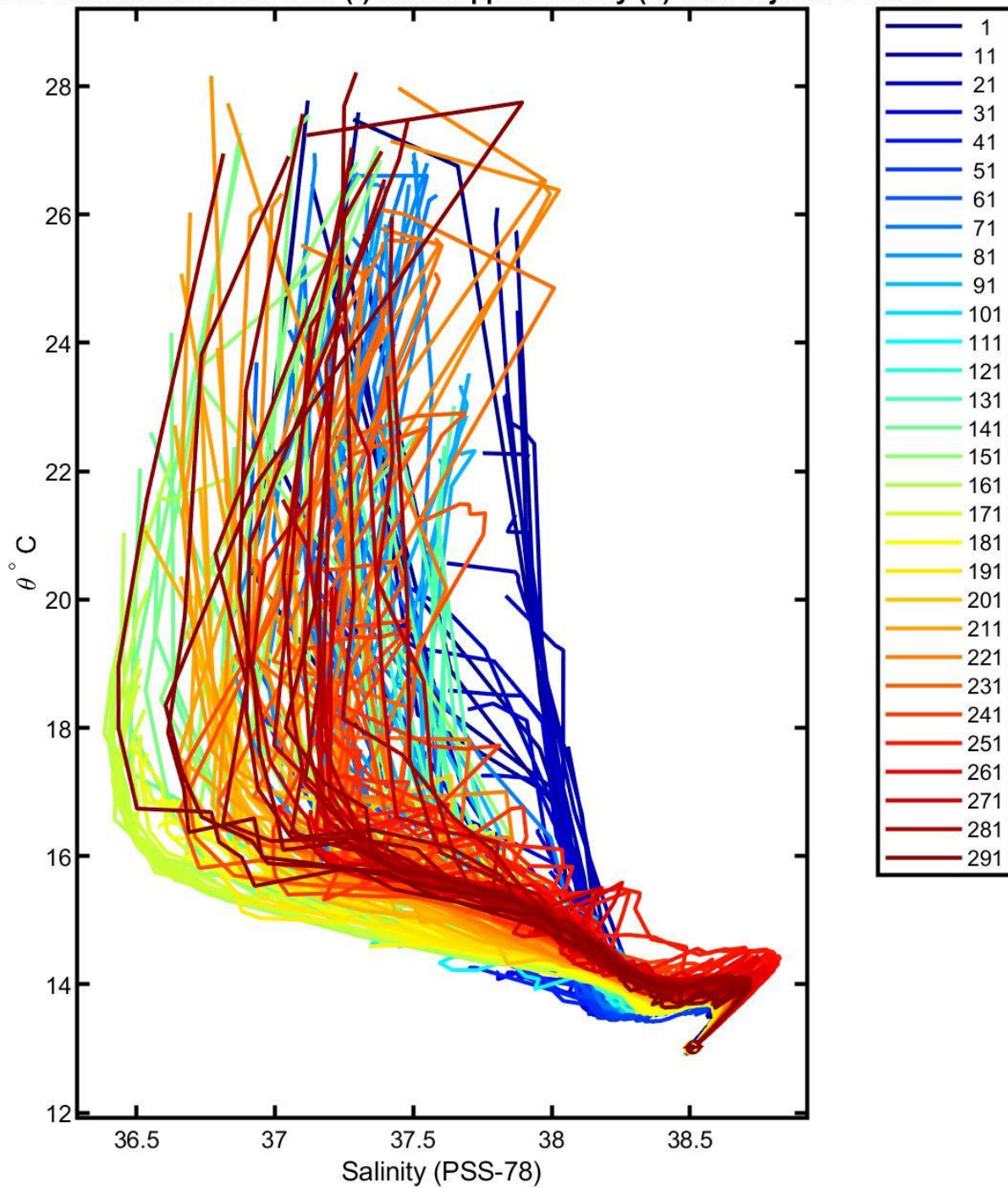
3901280 uncalibrated float data (-) and mapped salinity (o) with objective errors
