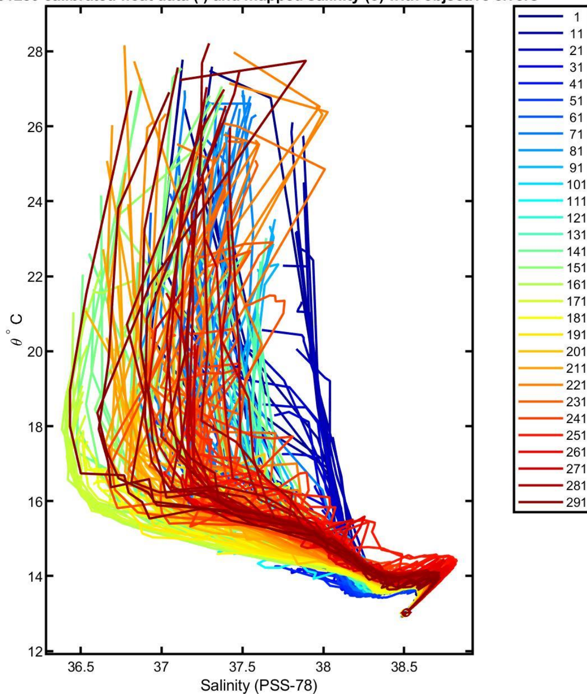
6901280 calibrated float data (-) and mapped salinity (o) with objective errors
