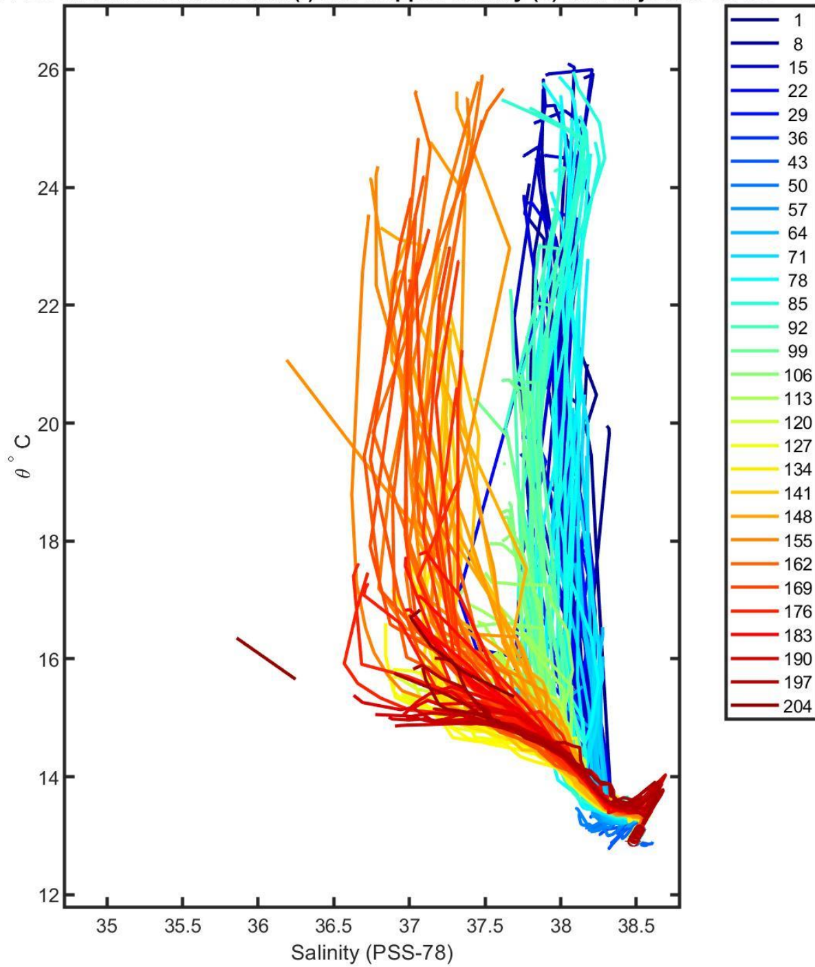
6901465 uncalibrated float data (-) and mapped salinity (o) with objective errors
