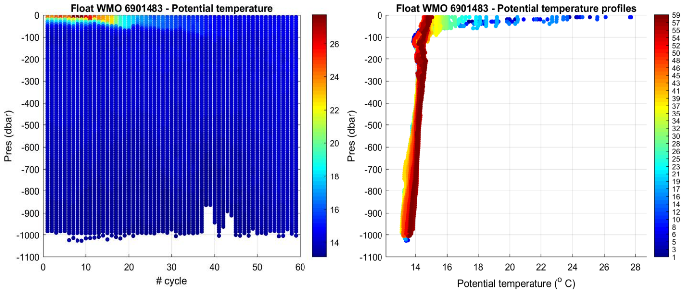
Figure 2: Float 6901483. Time series of Argo float potential temperature ( ^{\circ}\text{C} ) on the left, and potential temperature profiles color-coded per cycle number on the right.
