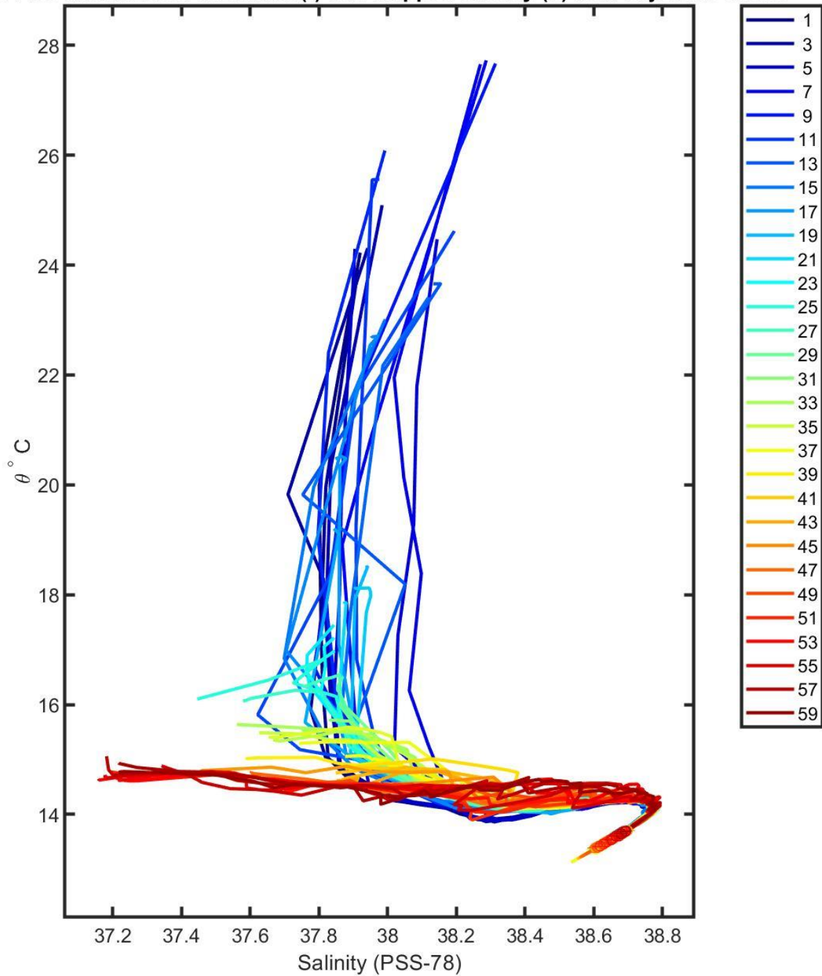
6901483 uncalibrated float data (-) and mapped salinity (o) with objective errors
