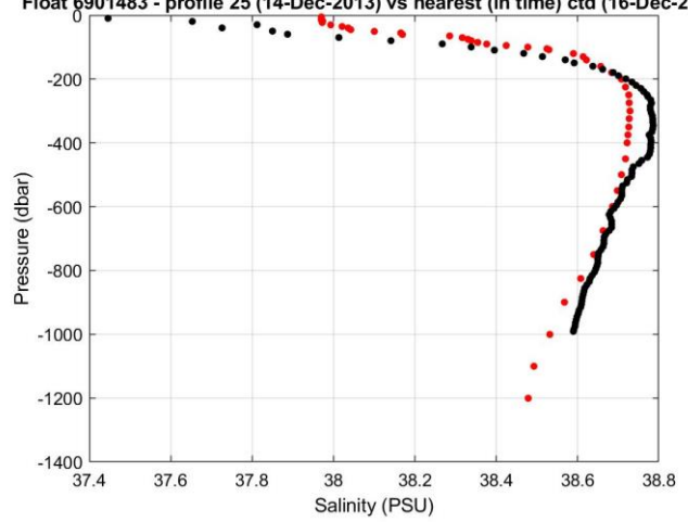
Float 6901483 - profile 25 (14-Dec-2013) vs nearest (in time) ctd (16-Dec-2013)
