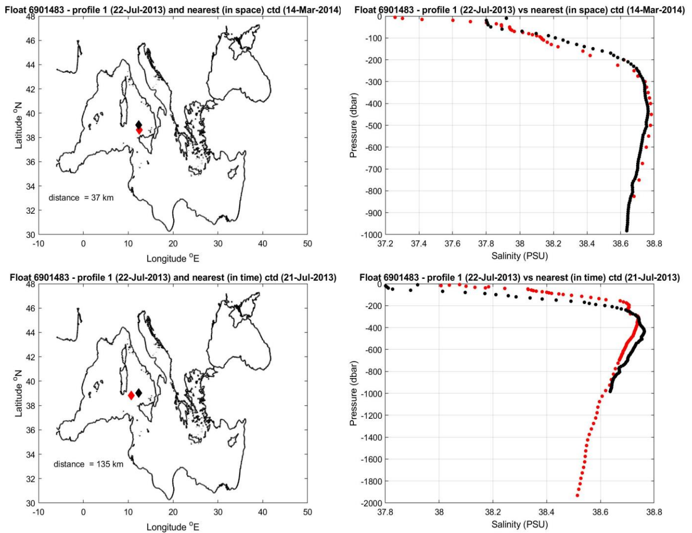
Figure 9: Float 6901483. The salinity float profile number 1 (black dots) are compared to the nearest in space (top) and in time (bottom) reference profile (red dots). The locations of the two profiles and their distance is given in the left panel.
