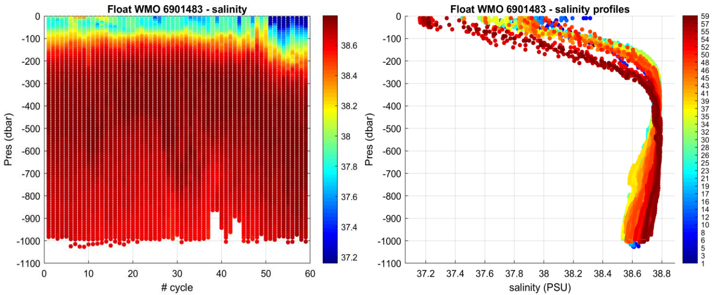
Figure 3: Float 6901483. Time series of Argo float potential salinity (PSS-78) on the left, and salinity profiles color-coded per cycle number on the right.
