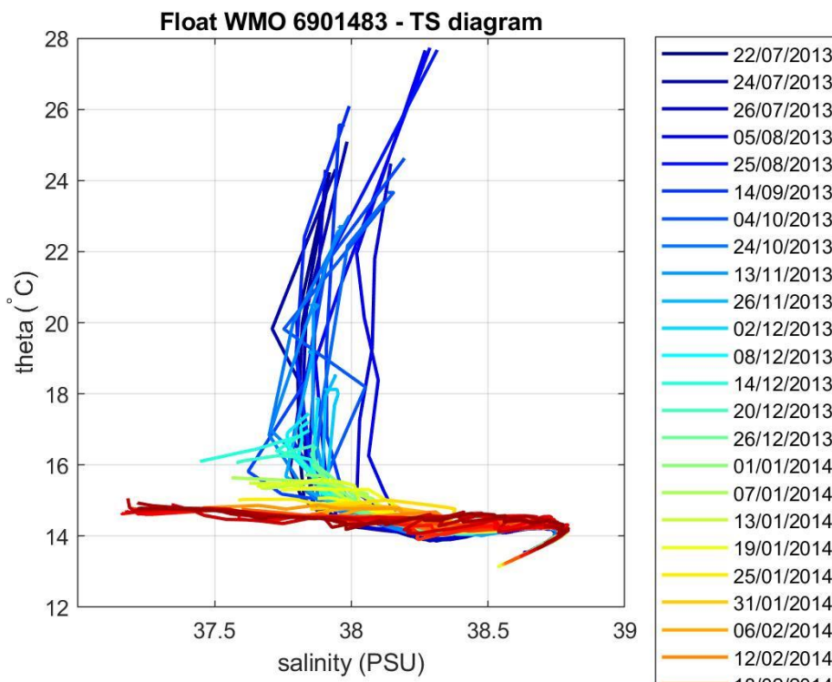
Figure 4: Float 6901483. \theta -S diagram color-coded per cycle number.
