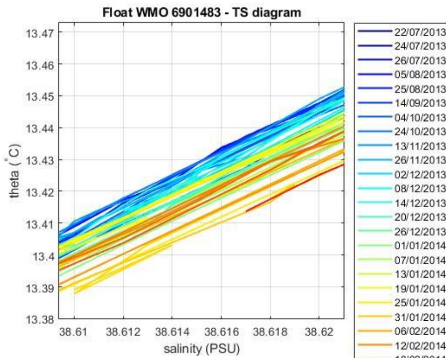
Figure 5: Float 6901483. Area of the \theta -S diagram (color-coded per cycle number) where the \theta -S relationship is more uniform.
