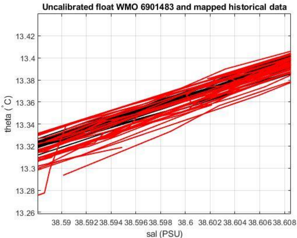
Figure 19: Float 6901483. Uncalibrated float salinity profile (black lines) and mapped historical data (red lines) in the most uniform part of the \theta -S curve.
