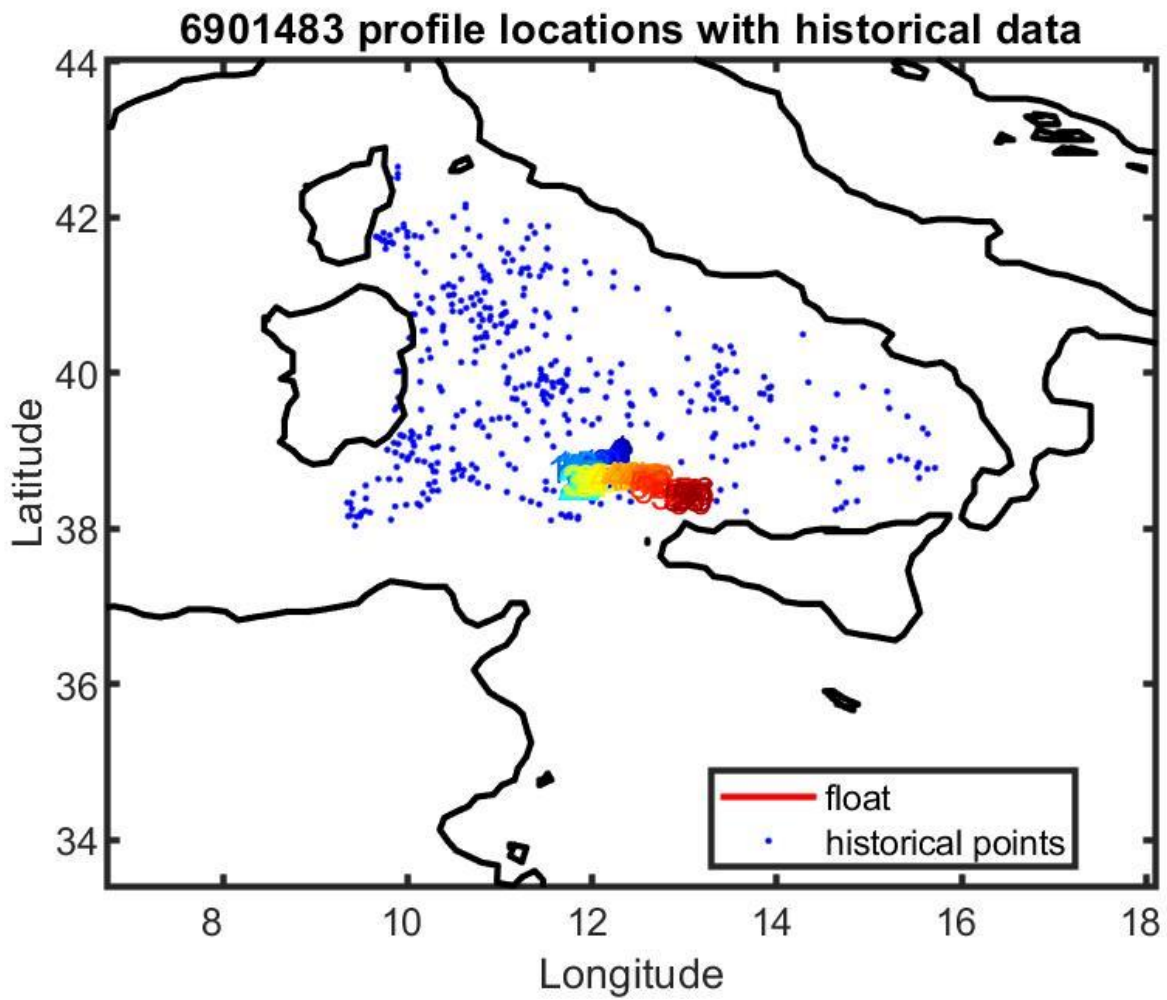
Figure 13: Float 6901483. Location of the float profiles (red line with colored numbers) and the reference data selected for mapping (blue dots).
