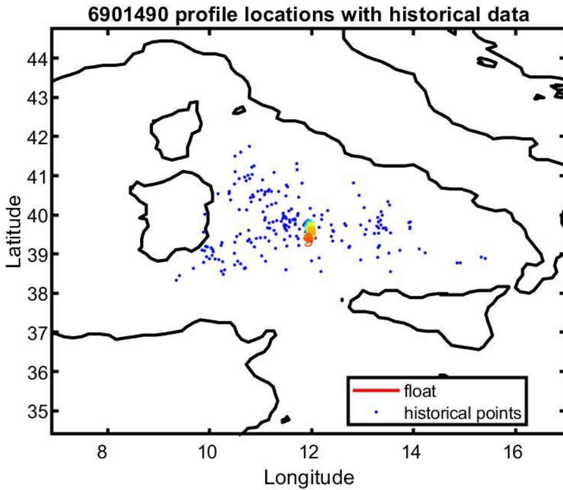
Figure 13: Float 6901490. Location of the float profiles (red line with colored numbers) and the reference data selected for mapping (blue dots).
