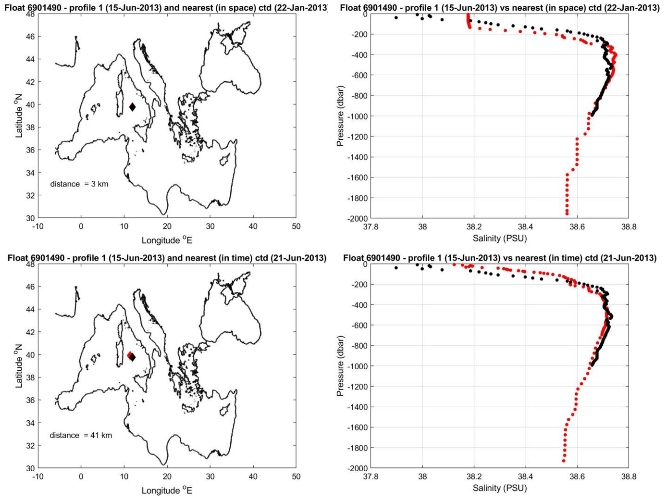
Figure 9: Float 6901490. The salinity float profile number 1 (black dots) are compared to the nearest in space (top) and in time (bottom) reference profile (red dots). The locations of the two profiles and their distance is given in the left panel.
