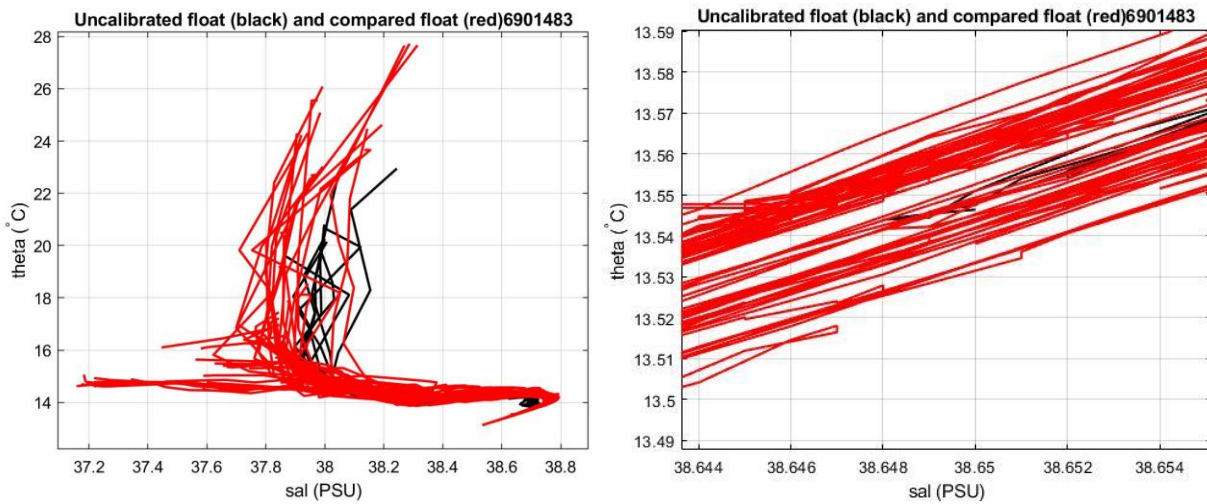
Figure 20: Float 6901490. Comparison between float 6901490 (black line) and 6901483 (red line), in the most uniform part of the \theta -S curve.
