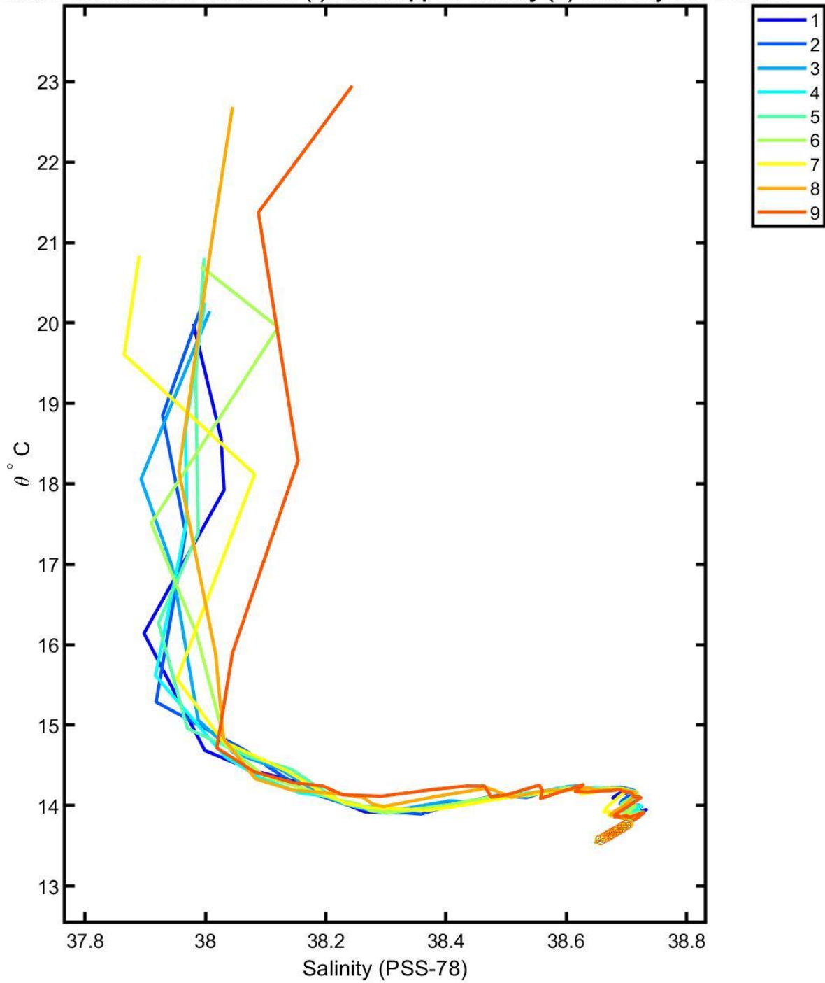
6901490 uncalibrated float data (-) and mapped salinity (o) with objective errors
