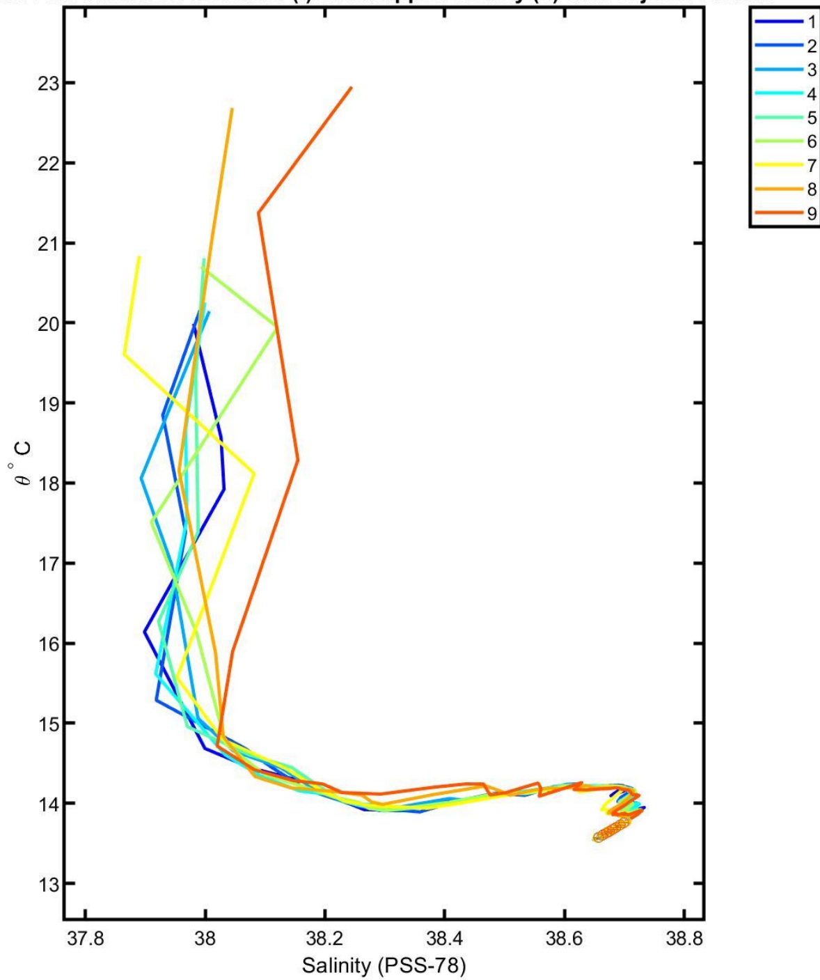
6901490 calibrated float data (-) and mapped salinity (o) with objective errors
