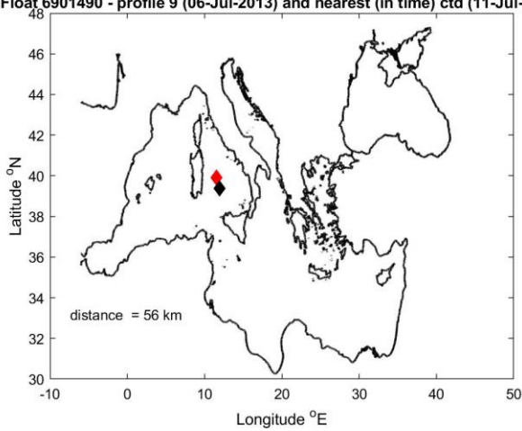
Float 6901490 - profile 9 (06-Jul-2013) and nearest (in time) ctd (11-Jul-2013)
