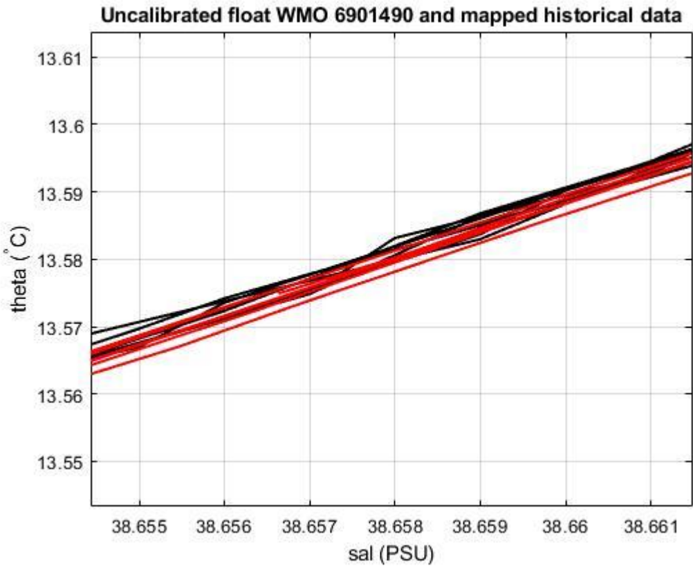
Figure 19: Float 6901490. Uncalibrated float salinity profile (black lines) and mapped historical data (red lines) in the most uniform part of the \theta -S curve.
