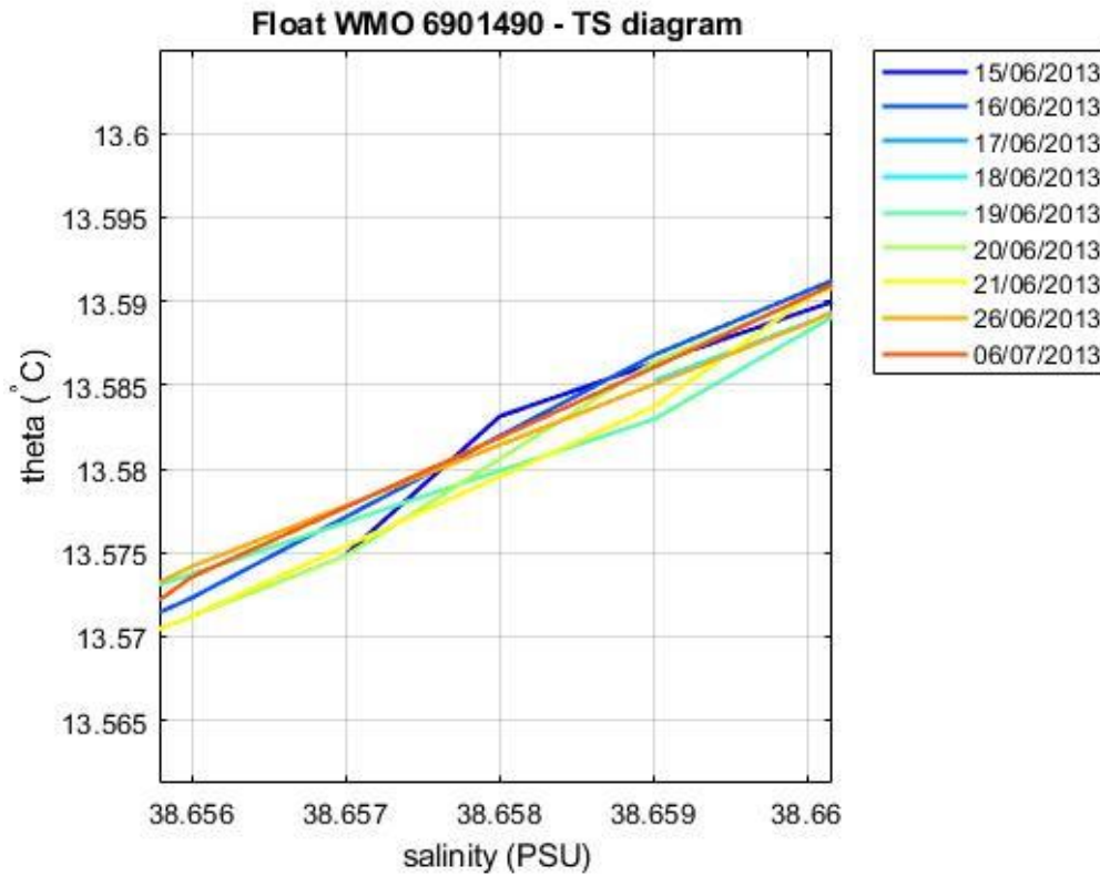
Figure 5: Float 6901490. Area of the \theta -S diagram (color-coded per cycle number) where the \theta -S relationship is more uniform.
