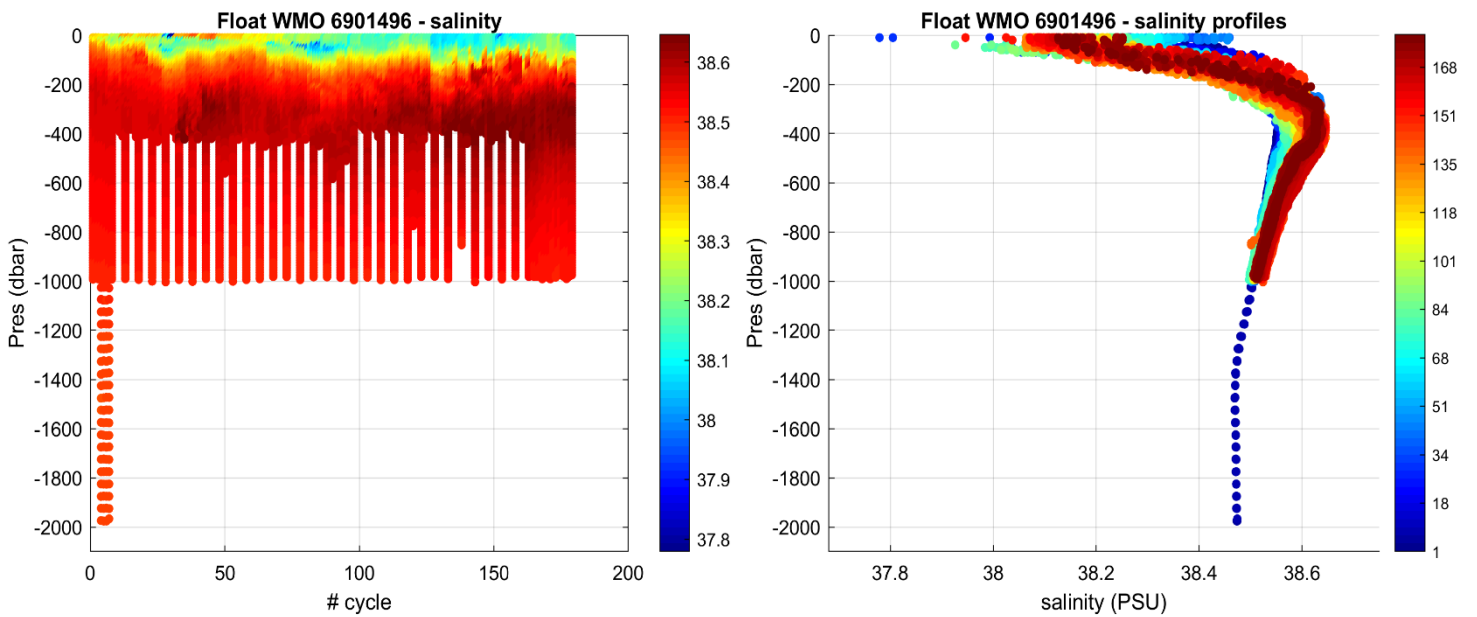
Figure 2: Float 6901496. Time series of Argo float potential salinity (PSS-78) on the left, and salinity profiles color-coded per cycle number on the right.
