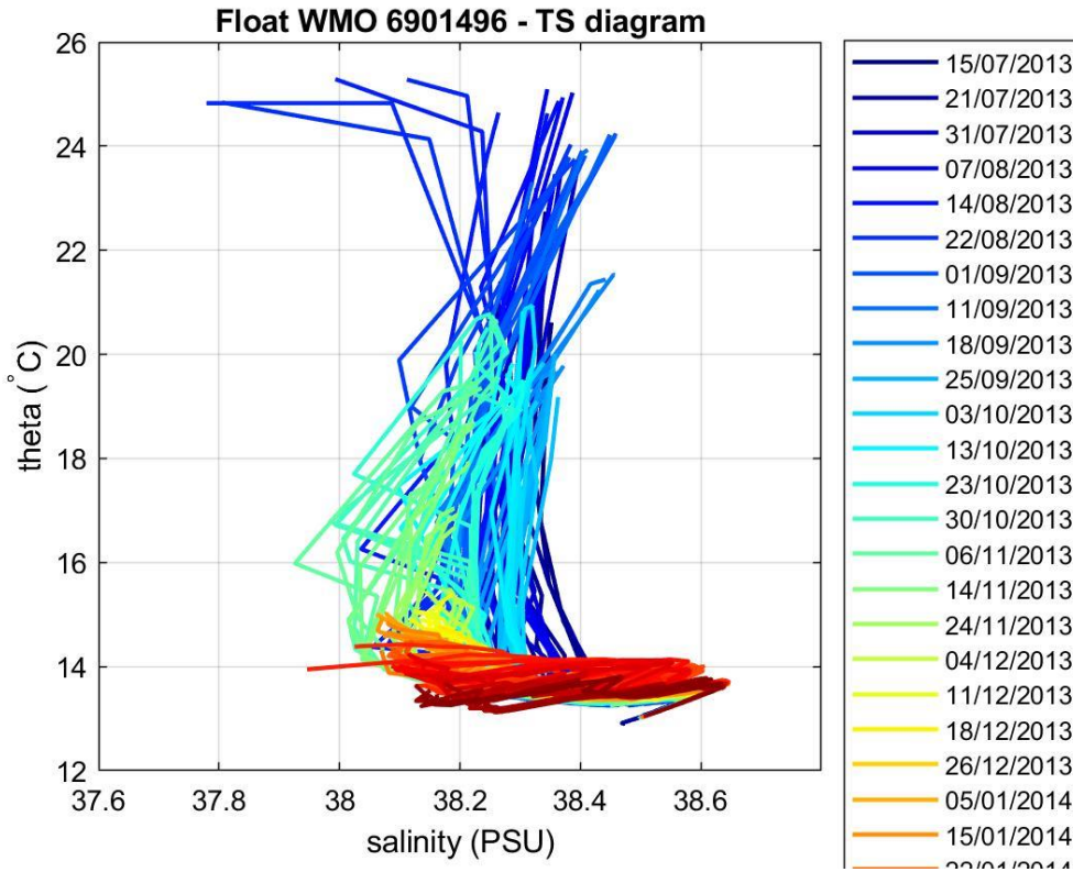
Figure 3: Float 6901496. \theta -S diagram color-coded per cycle number.
