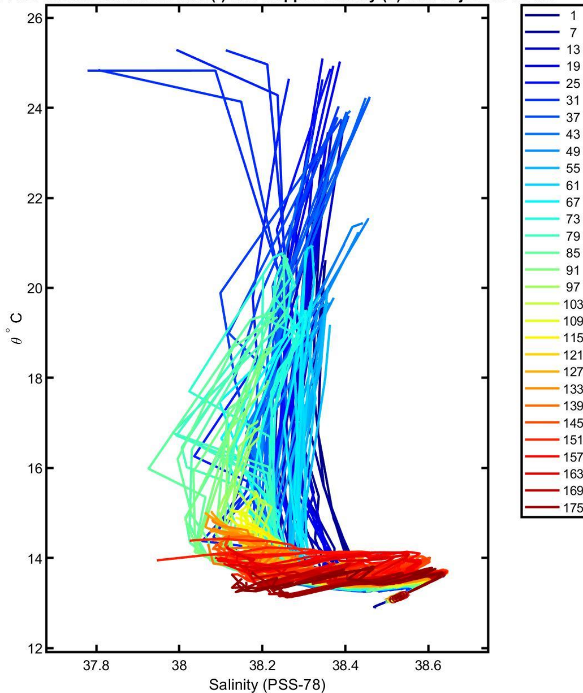
6901496 uncalibrated float data (-) and mapped salinity (o) with objective errors
