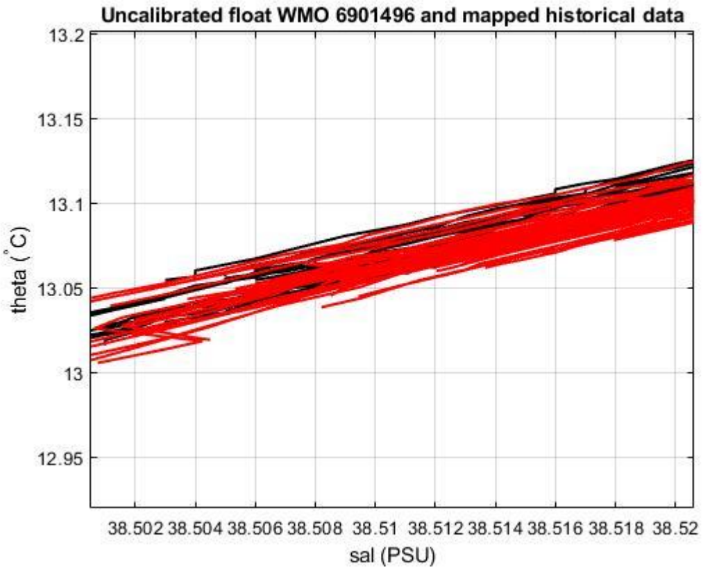
Figure 18: Float 6901496. Uncalibrated float salinity profile (black lines) and mapped historical data (red lines) in the most uniform part of the \theta -S curve.
