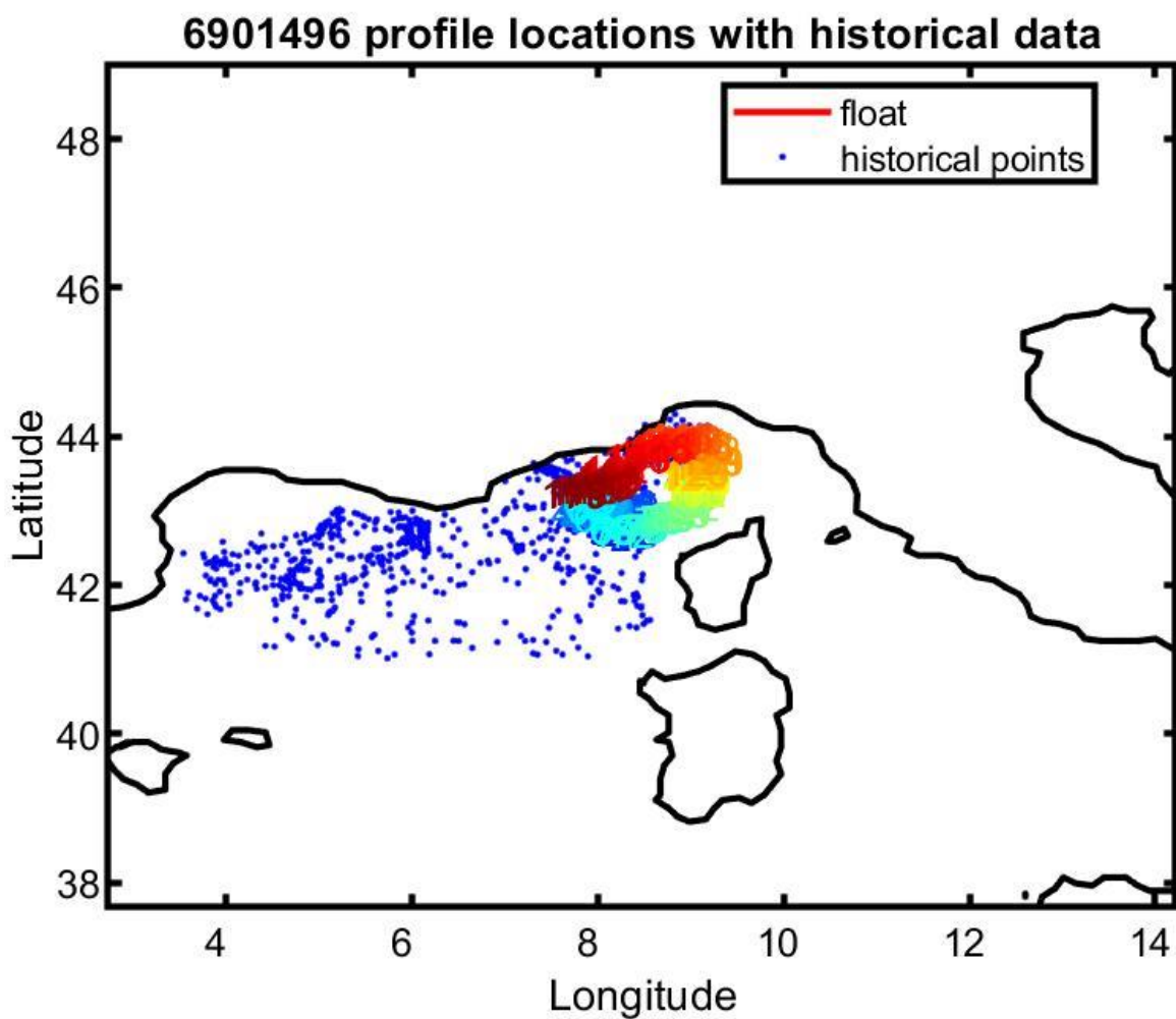
Figure 12: Float 6901496. Location of the float profiles (red line with colored numbers) and the reference data selected for mapping (blue dots).
