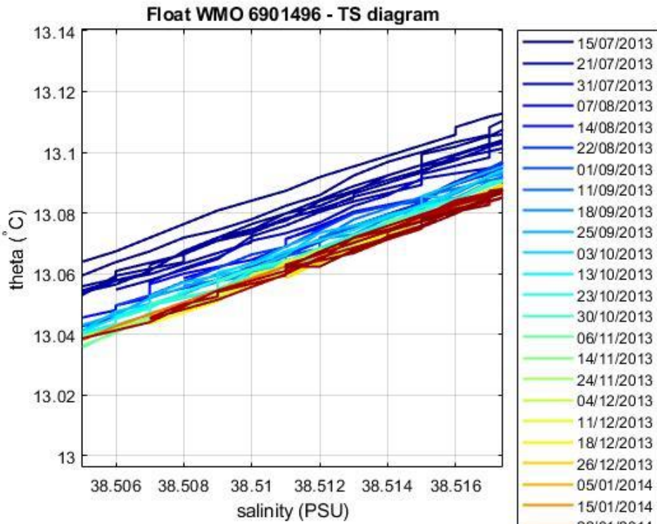
Figure 4: Float 6901496. Area of the \theta -S diagram (color-coded per cycle number) where the \theta -S relationship is more uniform.
