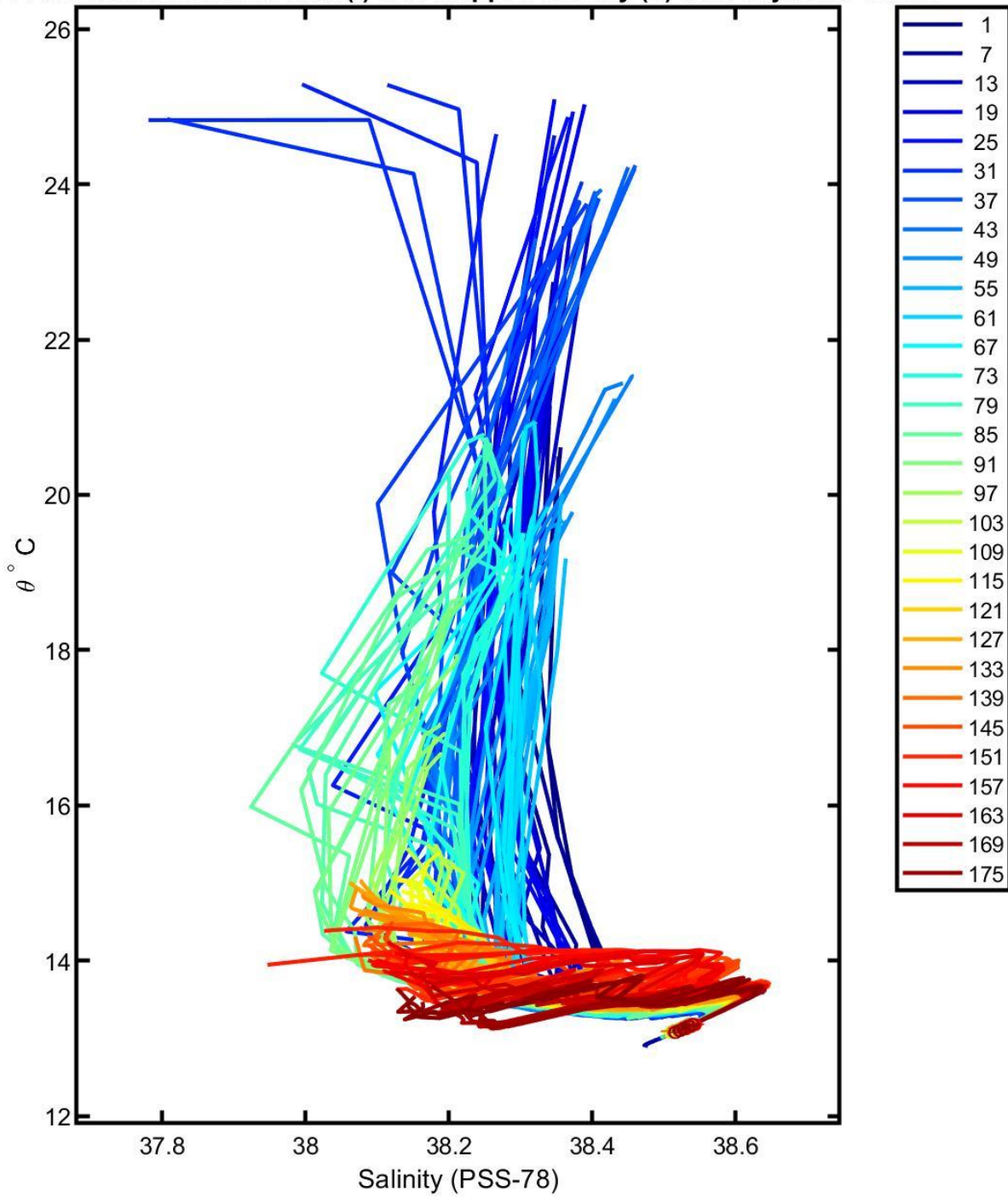
6901496 calibrated float data (-) and mapped salinity (o) with objective errors
