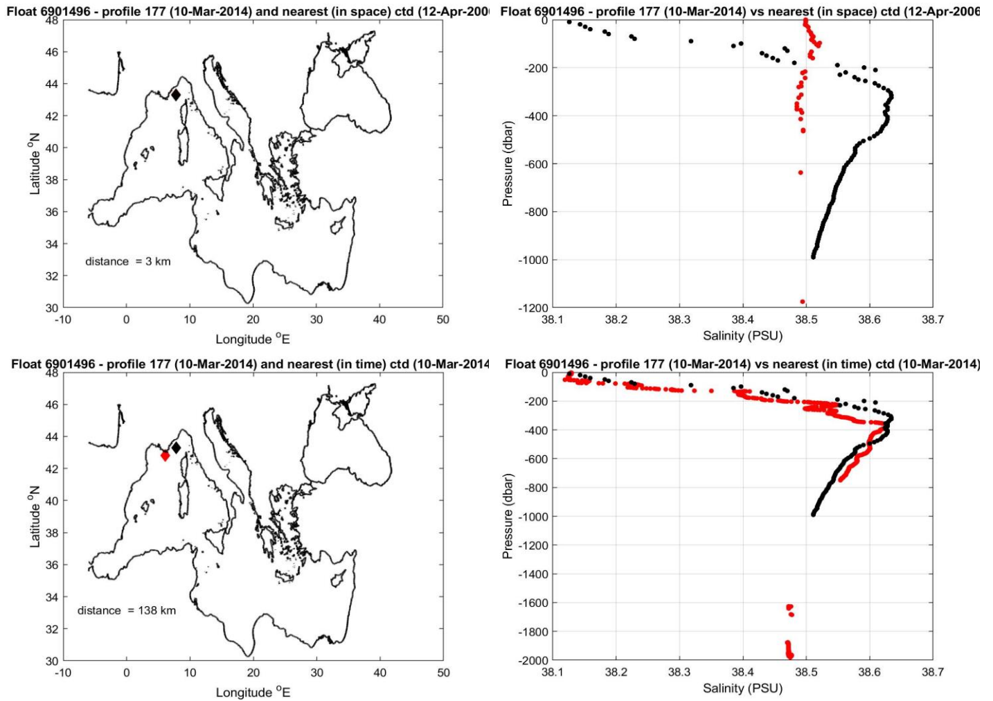
Figure 10: Float 6901496. The salinity float profile number 177 (black dots) are compared to the nearest in space (top) and in time (bottom) reference profile (red dots). The locations of the two profiles and their distance is given in the left panel.
