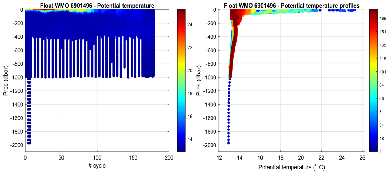
Figure 1: Float 6901496. Time series of Argo float potential temperature ( ^{\circ} C) on the left, and potential temperature profiles color-coded per cycle number on the right.
