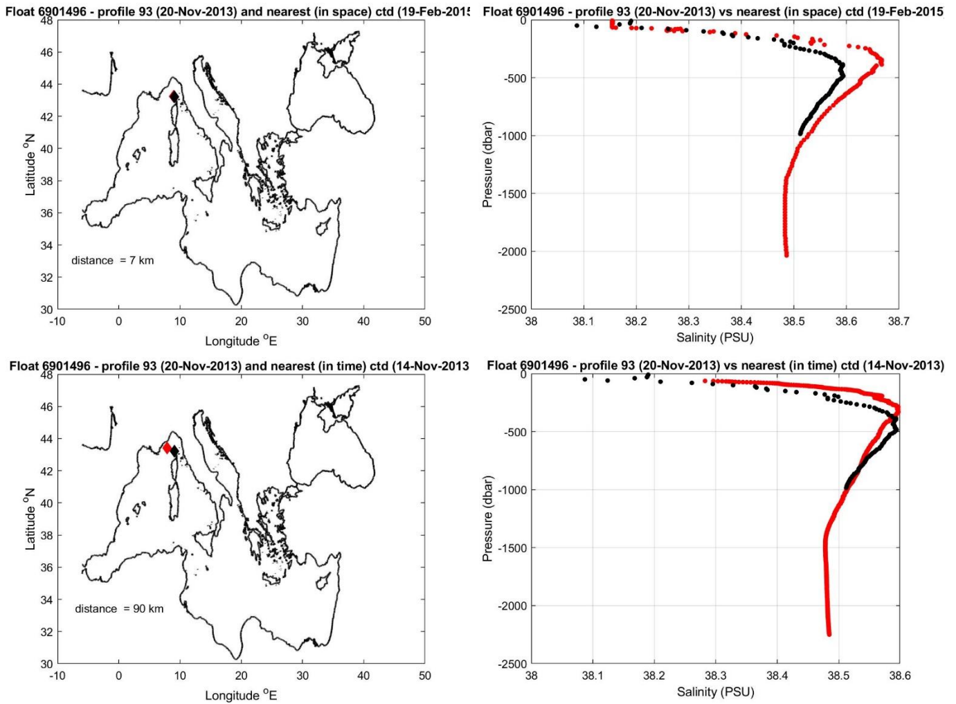
Figure 9: Float 6901496. The salinity float profile number 93 (black dots) are compared to the nearest in space (top) and in time (bottom) reference profile (red dots). The locations of the two profiles and their distance is given in the left panel.
