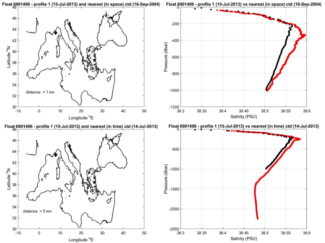
Figure 8: Float 6901496. The salinity float profile number 1 (black dots) are compared to the nearest in space (top) and in time (bottom) reference profile (red dots). The locations of the two profiles and their distance is given in the left panel.
