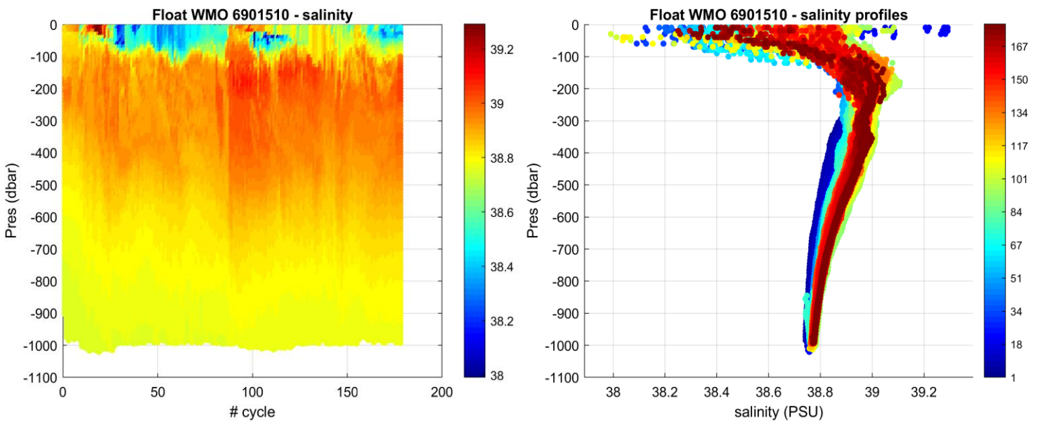
Figure 3: Float 6901510. Time series of Argo float potential salinity (PSS-78) on the left, and salinity profiles color-coded per cycle number on the right.
