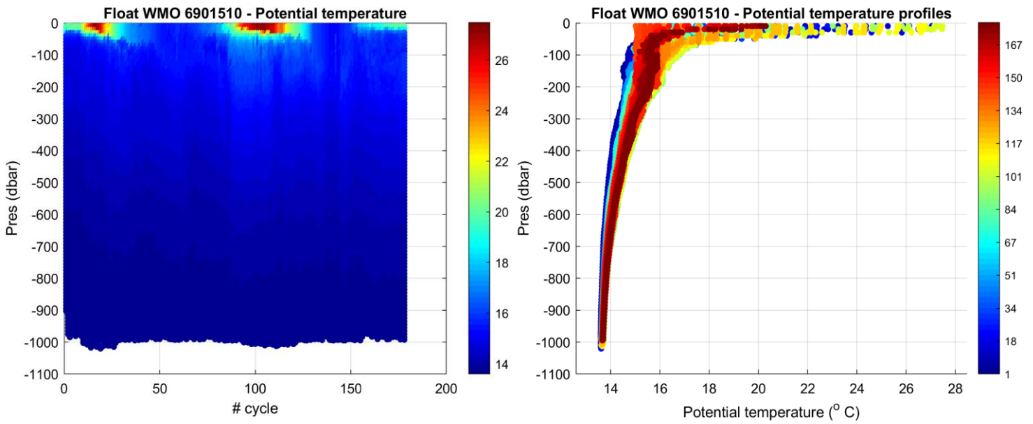
Figure 2: Float 6901510. Time series of Argo float potential temperature ( ^{\circ}\text{C} ) on the left, and potential temperature profiles color-coded per cycle number on the right.
