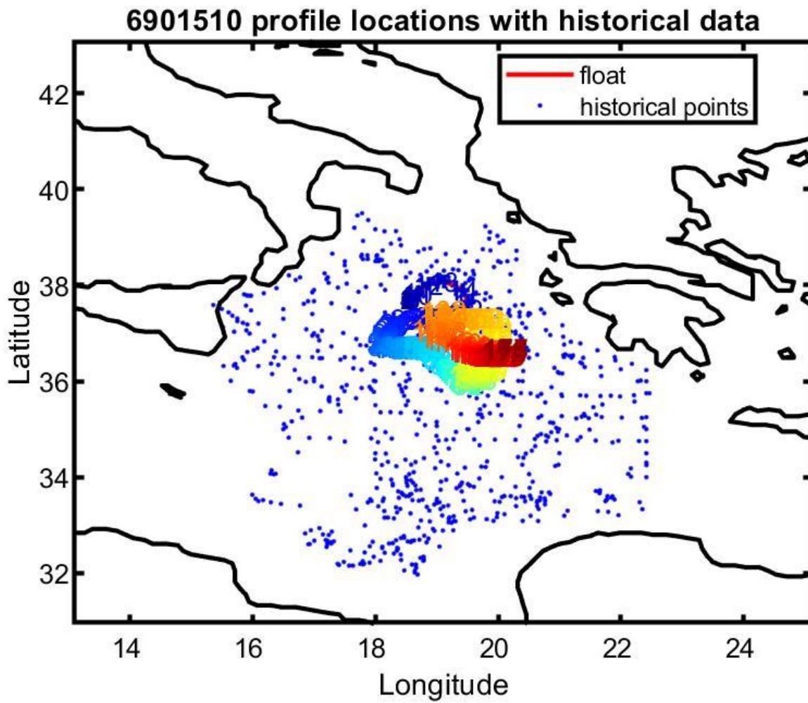
Figure 13: Float 6901510. Location of the float profiles (red line with colored numbers) and the reference data selected for mapping (blue dots).
