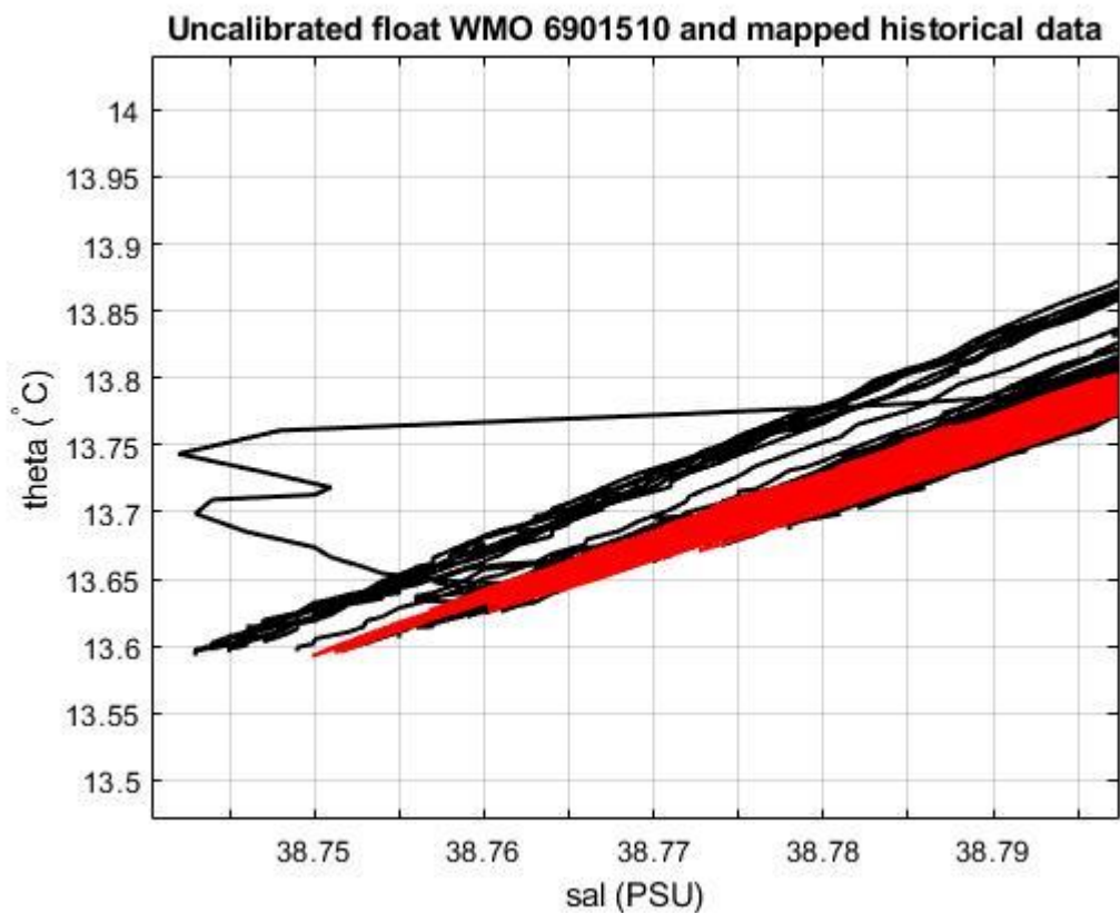
Figure 19: Float 6901510. Uncalibrated float salinity profile (black lines) and mapped historical data (red lines) in the most uniform part of the \theta -S curve.
