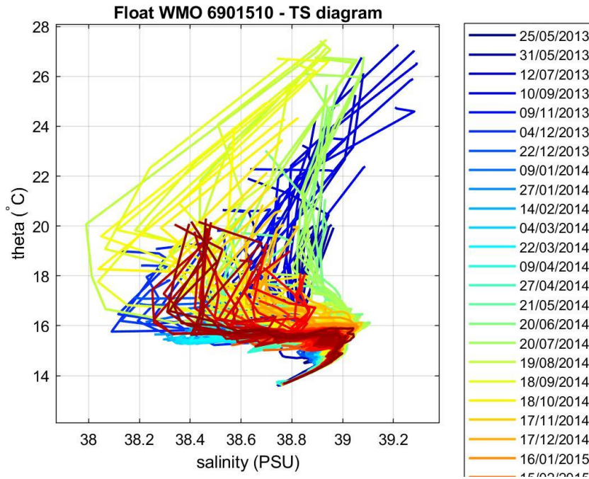
Figure 4: Float 6901510. \theta -S diagram color-coded per cycle number.
