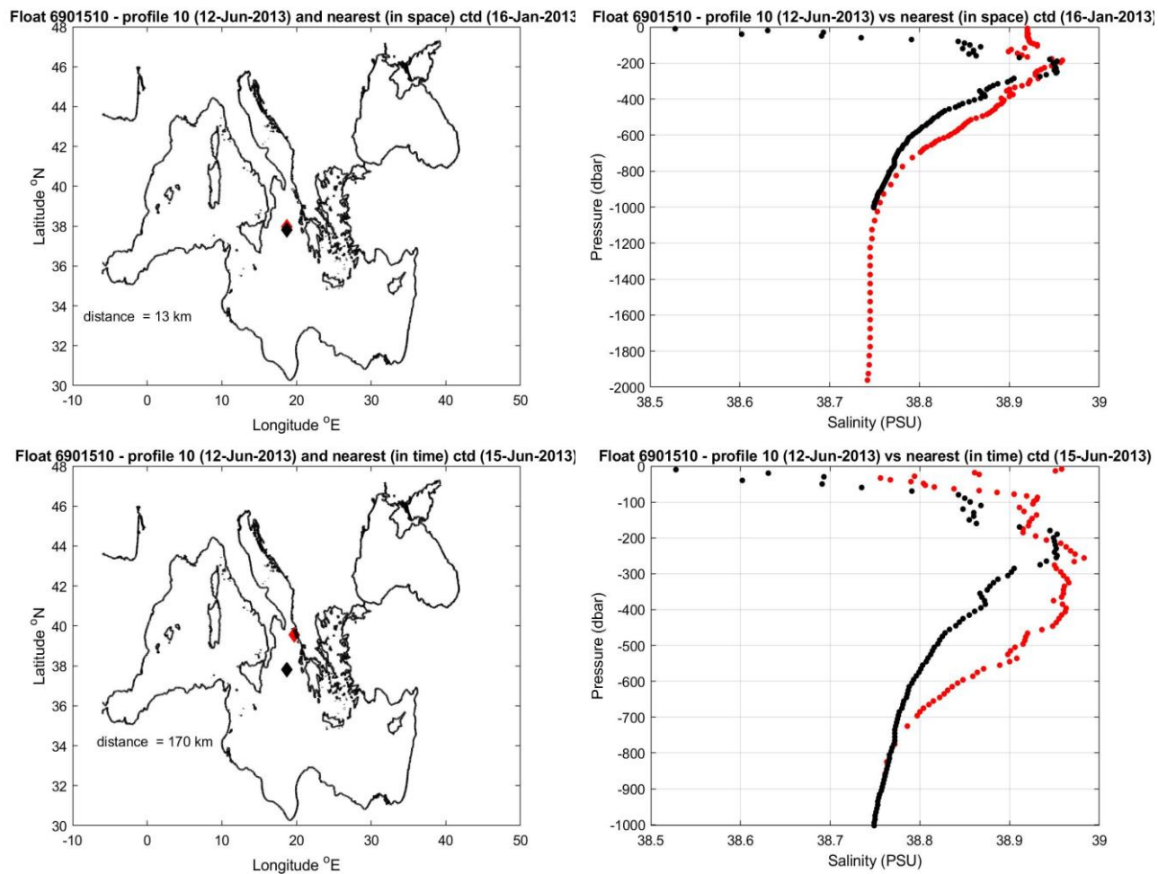
Figure 9: Float 6901510. The salinity float profile number 10 (black dots) are compared to the nearest in space (top) and in time (bottom) reference profile (red dots). The locations of the two profiles and their distance is given in the left panel.
