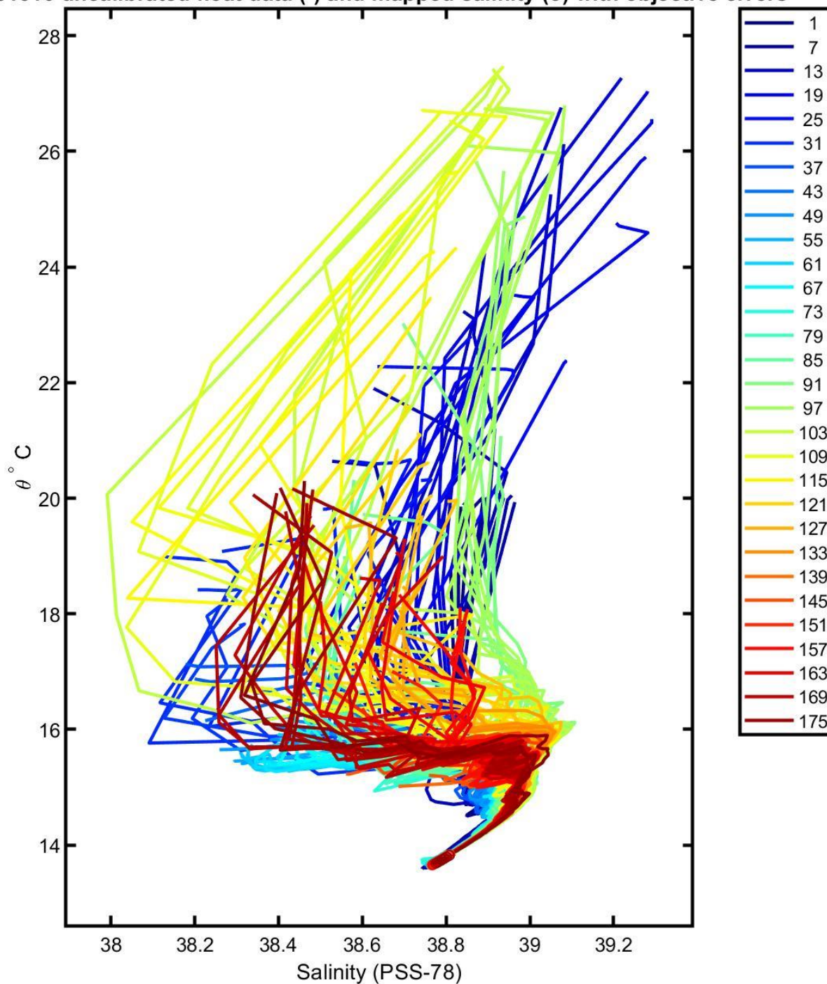
6901510 uncalibrated float data (-) and mapped salinity (o) with objective errors
