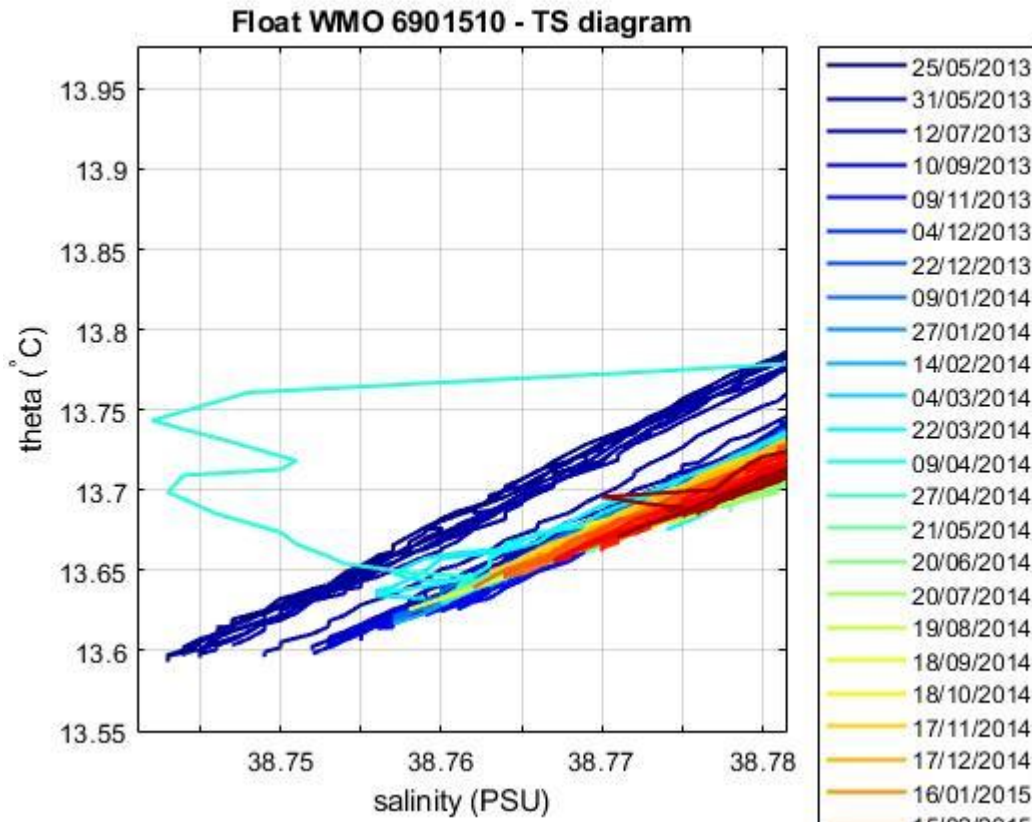
Figure 5: Float 6901510. Area of the \theta -S diagram (color-coded per cycle number) where the \theta -S relationship is more uniform.
