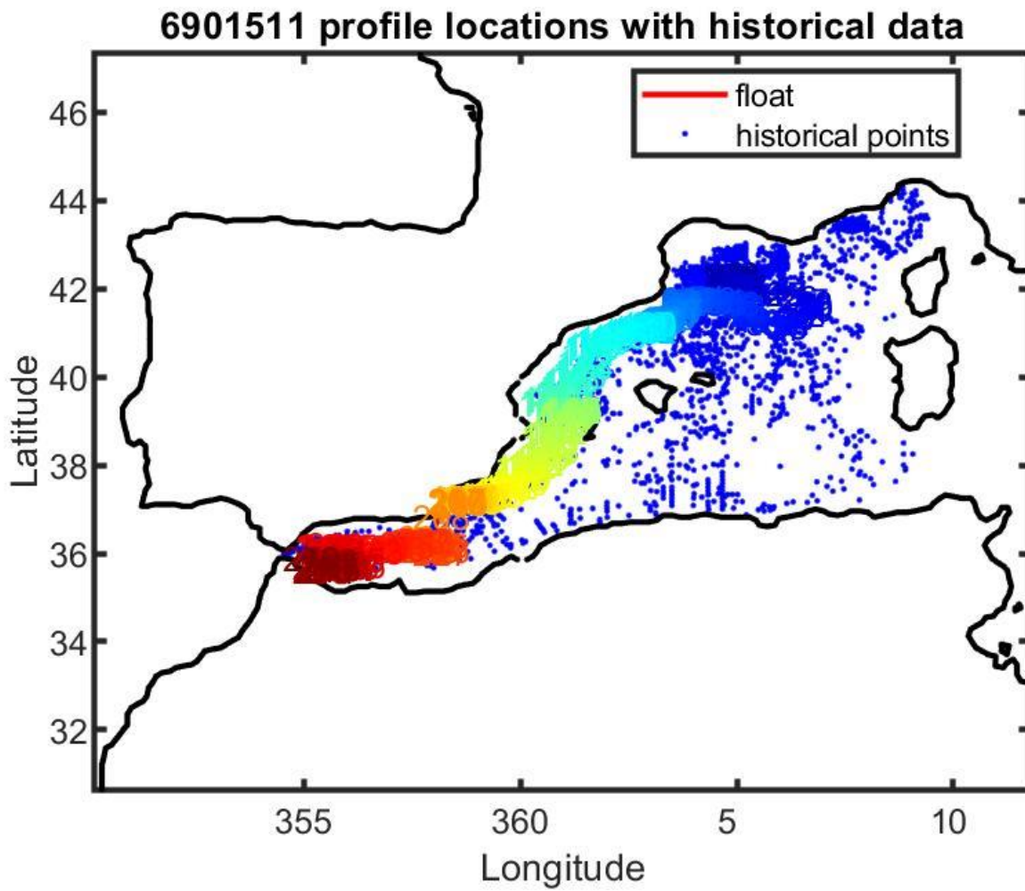
Figure 13: Float 6901511. Location of the float profiles (red line with colored numbers) and the reference data selected for mapping (blue dots).
