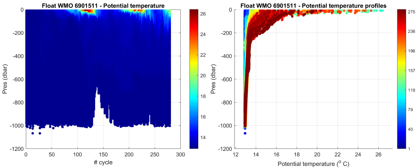
Figure 2: Float 6901511. Time series of Argo float potential temperature ( ^{\circ}\text{C} ) on the left, and potential temperature profiles color-coded per cycle number on the right.
