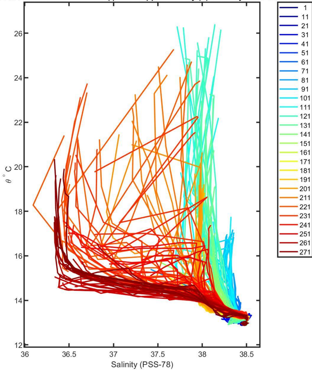
6901511 calibrated float data (-) and mapped salinity (o) with objective errors
