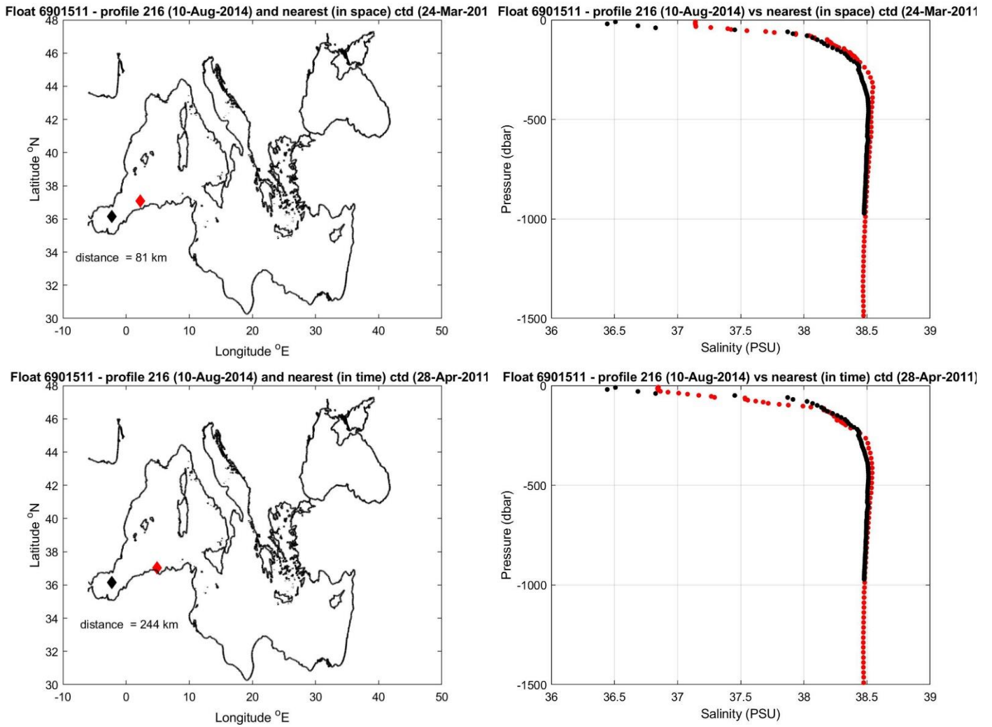
Figure 11: Float 6901511. The salinity float profile number 216 (black dots) are compared to the nearest in space (top) and in time (bottom) reference profile (red dots). The locations of the two profiles and their distance is given in the left panel.
