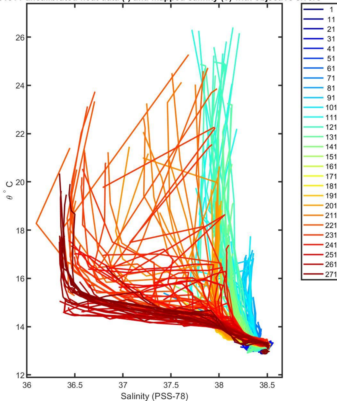
6901511 uncalibrated float data (-) and mapped salinity (o) with objective errors
