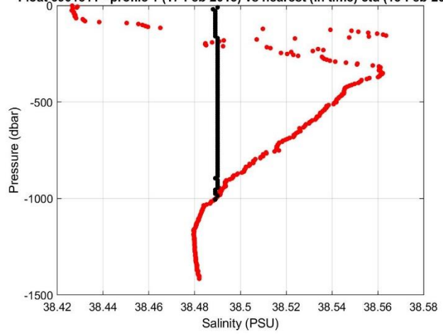
Float 6901511 - profile 1 (17-Feb-2013) vs nearest (in time) ctd (18-Feb-2013)
