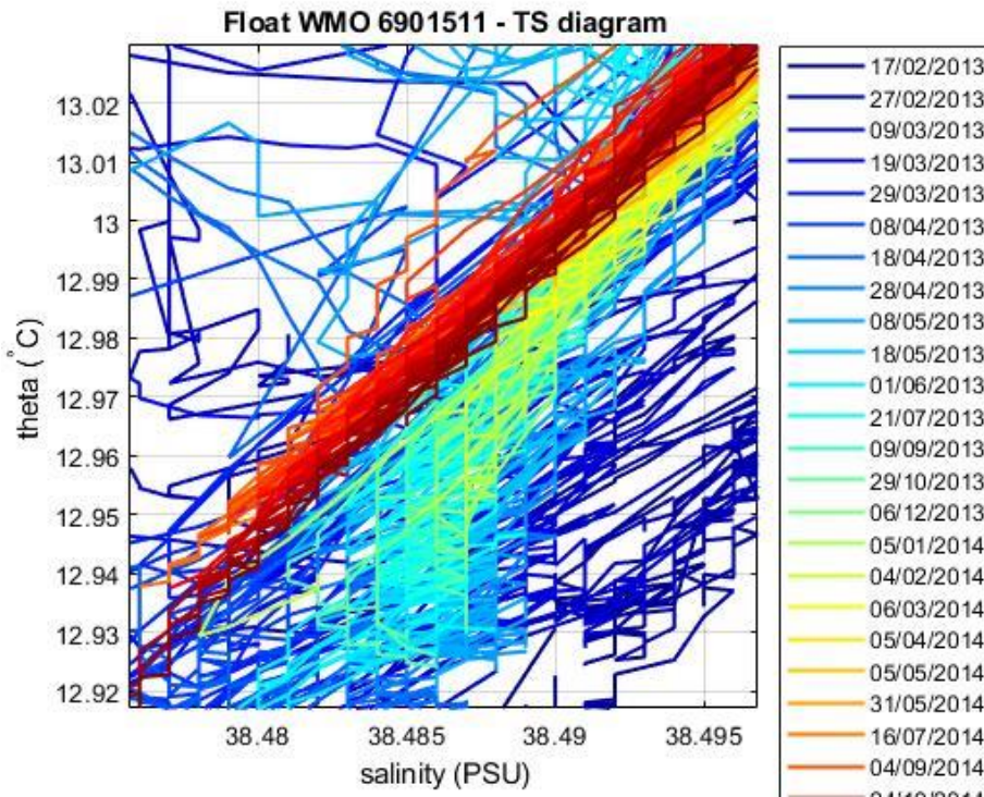
Figure 5: Float 6901511. Area of the \theta -S diagram (color-coded per cycle number) where the \theta -S relationship is more uniform.
