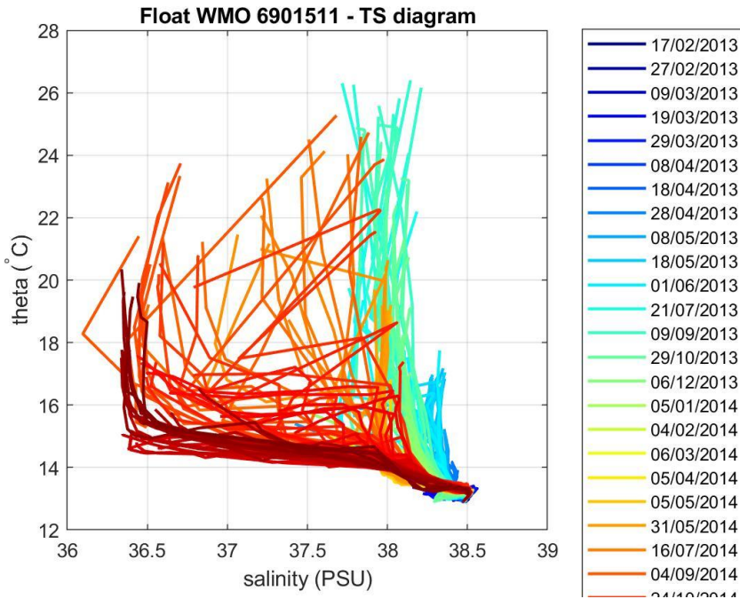
Figure 4: Float 6901511. \theta -S diagram color-coded per cycle number.
