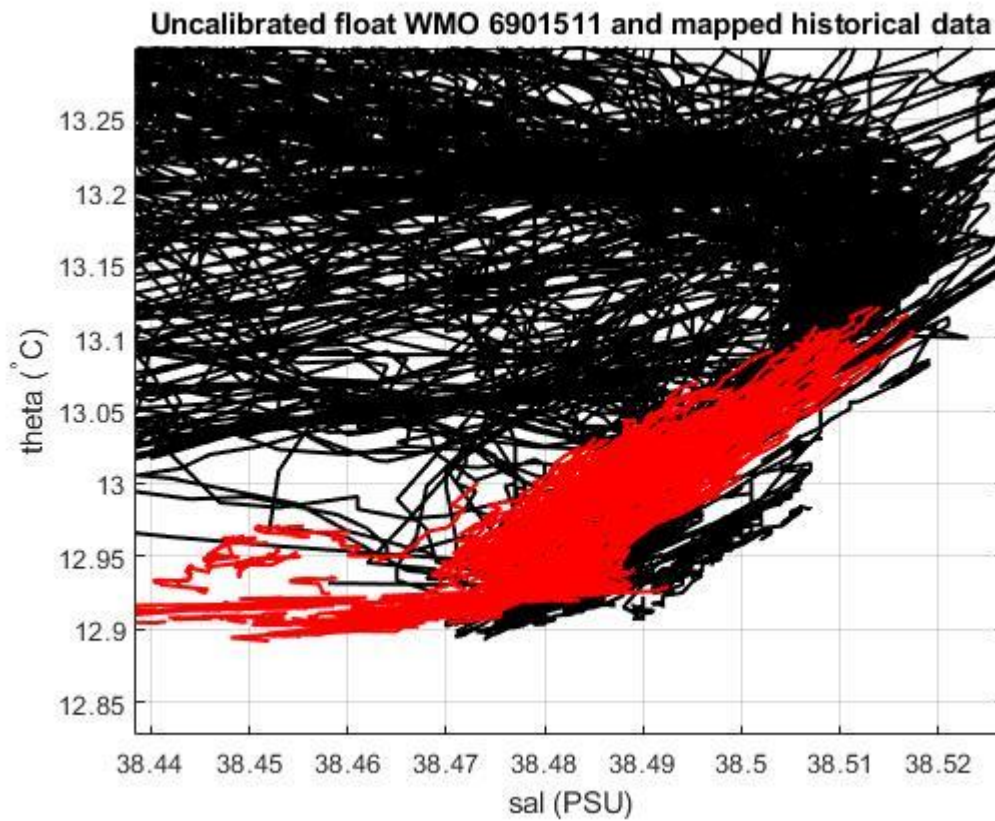
Figure 19: Float 6901511. Uncalibrated float salinity profile (black lines) and mapped historical data (red lines) in the most uniform part of the \theta -S curve.
